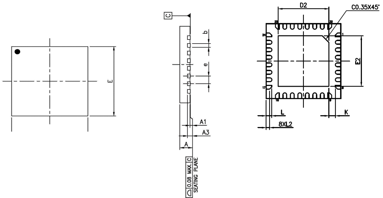
Figure 15 QFN-32 (4mm X 4mm X 0.55mm)
