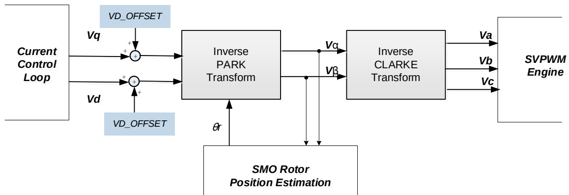
Figure 19.23.1 : Inverse Coordinate Transformation Block Architecture
