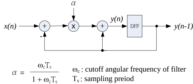
Figure 19.30.1 : first order digital low-pass filter Architecture
