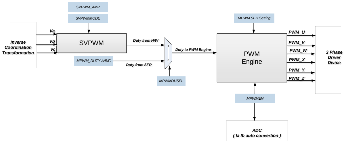
Figure 19.25.1 : SVPWM Engine Block Architecture
