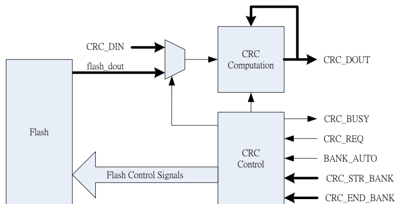
Figure 19.2 : The byte and flash bank CRC computation architecture
