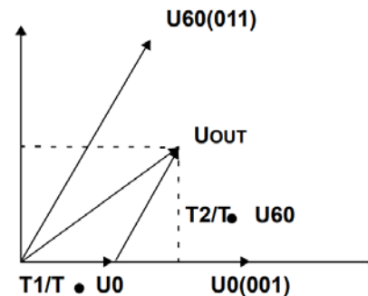
Figure 19.25.3 : AVERAGE SVPWM
