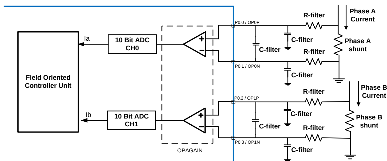
Figure 14.2.1 The block diagram of ADC CH0 and CH1 for Sensor-less FOC motor driving
