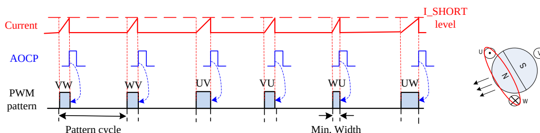
Figure 19.28.1 : IPD principle
