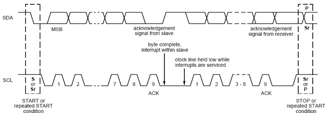
Figure 16.2.1 : Acknowledgement bit in the 9th bit of a byte transmission
