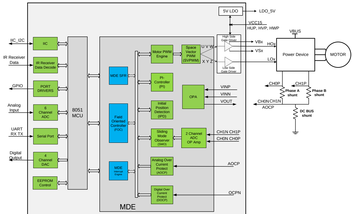
Figure 2.1 BLDC motor controller block diagram
