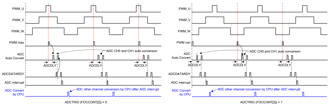
Figure 14.3.1 : The Timing Diagram of ADC Convert by MDE and CUP
