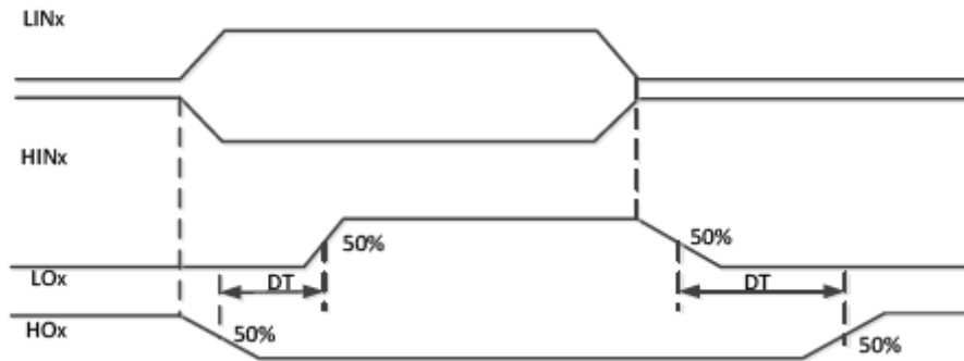
Figure 20.4.1 Dead Time
