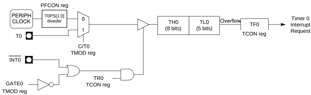
Figure 13.4.5 Timer0 Mode 0
