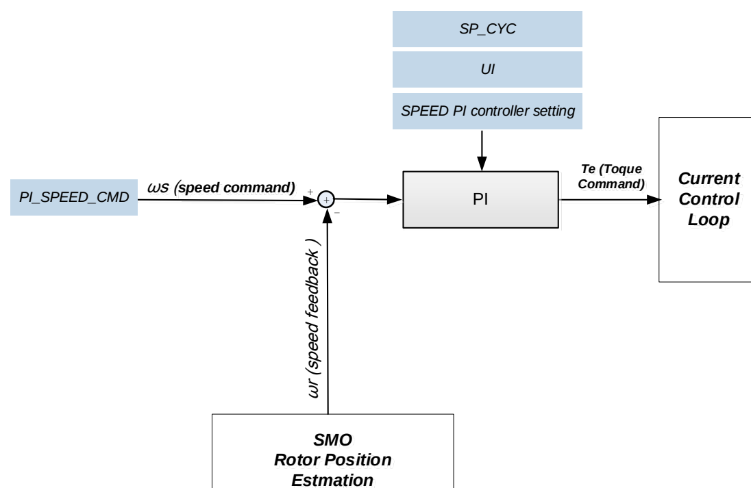
Figure 19.26.1 : Speed Control Loop Block Architecture
