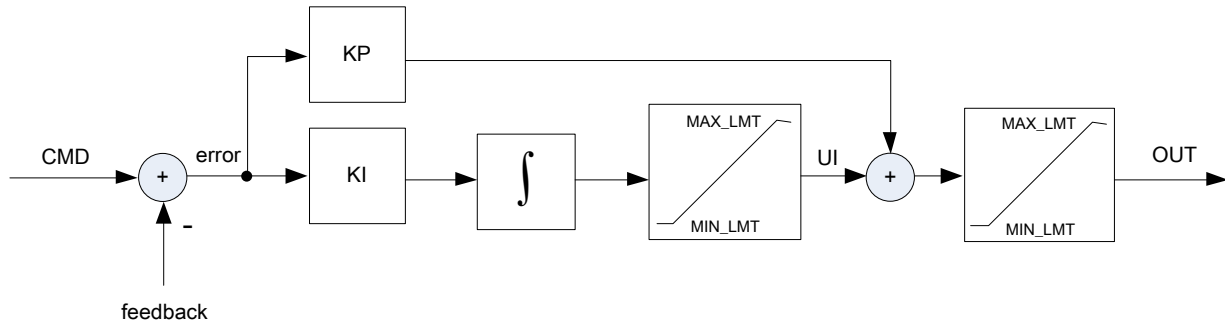
Figure 19.27.3 : User PI Block Architecture
