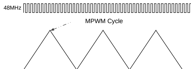
Figure 19.25.6 : Motor PWM is count up and down timer
