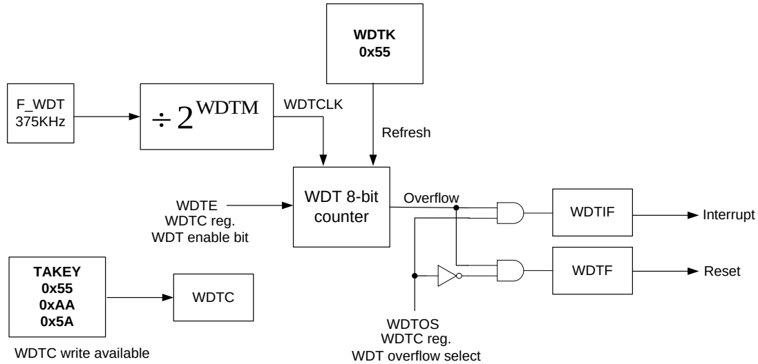
Figure 13.5 Watchdog Timer
