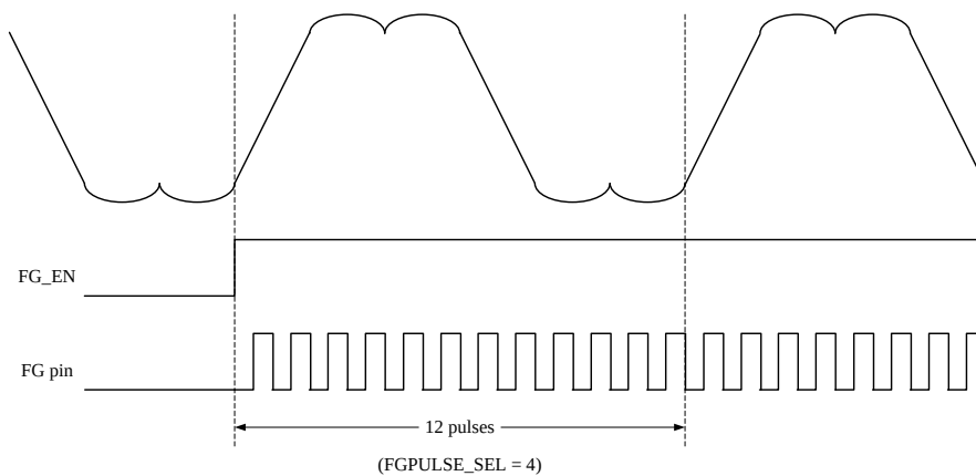
Figure 19.31.1 :FG Output Waveform
