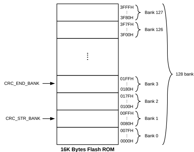
Figure 19.2 : The byte and flash bank CRC computation architecture
