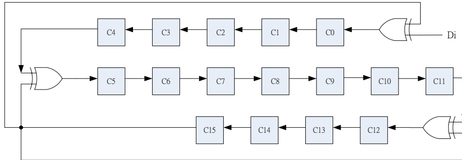
Figure 19.1 : The general LFSR architecture of CRC16-CCITT
