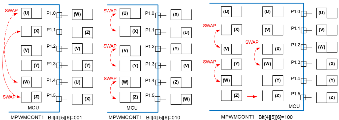
Figure 19.25.7 : PWM Pin swap Unit Architecture
