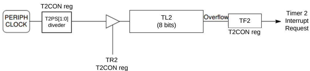
Figure 13.4.15 Timer2 Mode 3
