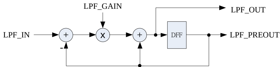
Figure 19.30.2 : LPF architecture and corresponding parameters
