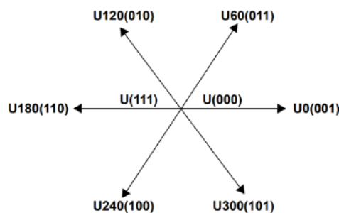
Figure 19.25.2 : Space Vector Pulse Width Modulation (SVPWM)
