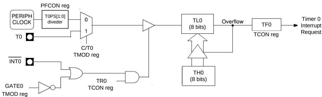
Figure 13.4.7 Timer0 Mode 2
