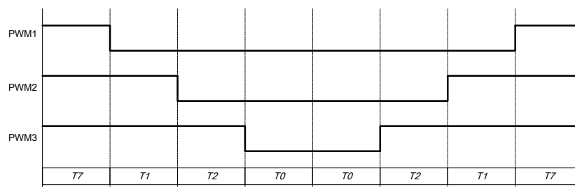
Figure 19.25.4 : 7-segment SVPWM output voltage
