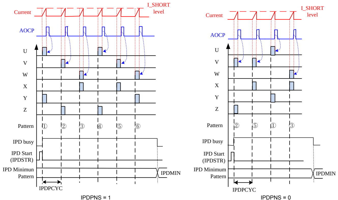
Figure 19.28.2 : IPD for rotor position detect before spin up in 6-pattern or 4-pattern
