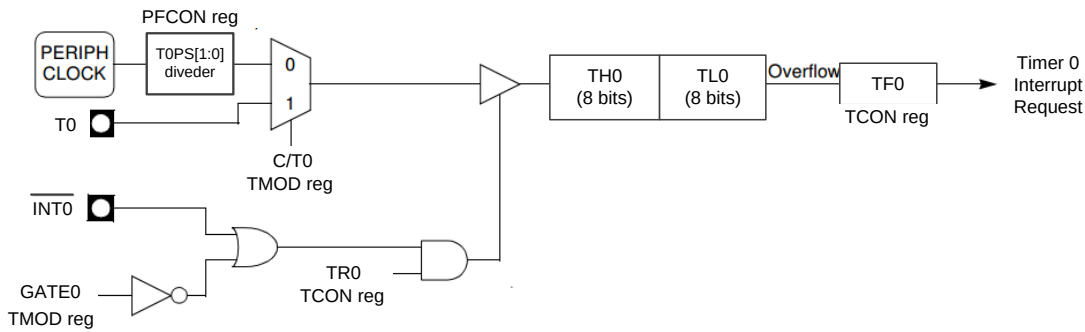
Figure 13.4.6 Timer0 Mode 1
