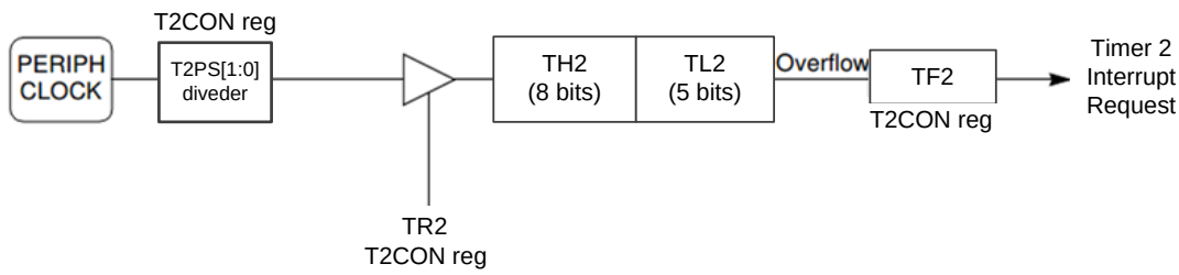
Figure 13.4.12 Timer2 Mode 0
