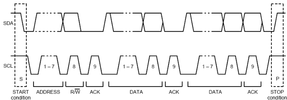
Figure 16.3.1 : RW bit in the 8th bit after IIC address
