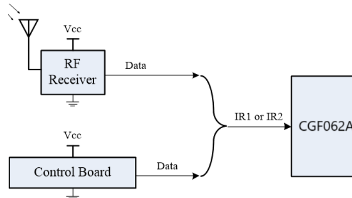
Figure 19.10 : One wire signal decode by CGF062A
