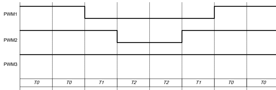
Figure 19.25.5 : 5-segment SVPWM output voltage
