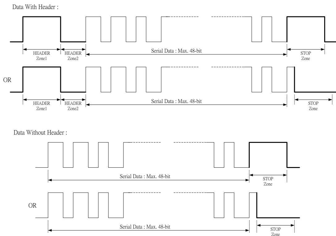
Figure 19.11.1 : The header and stop signal express
