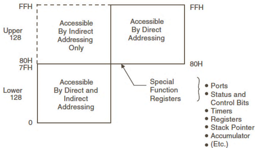
Figure 11.2.1 Data Memory (IRAM)(00H~FFH)
