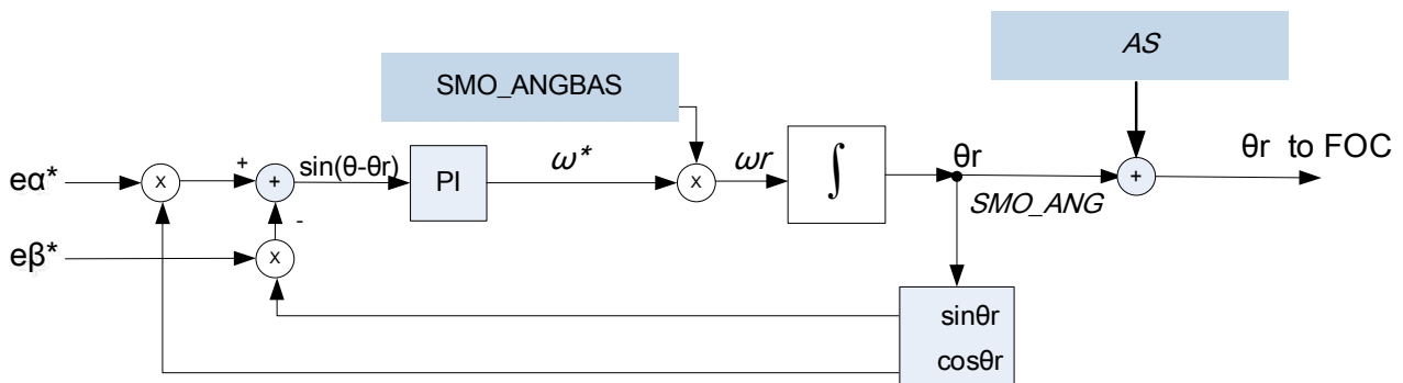
Figure 19.24.3 : PLL Architecture
