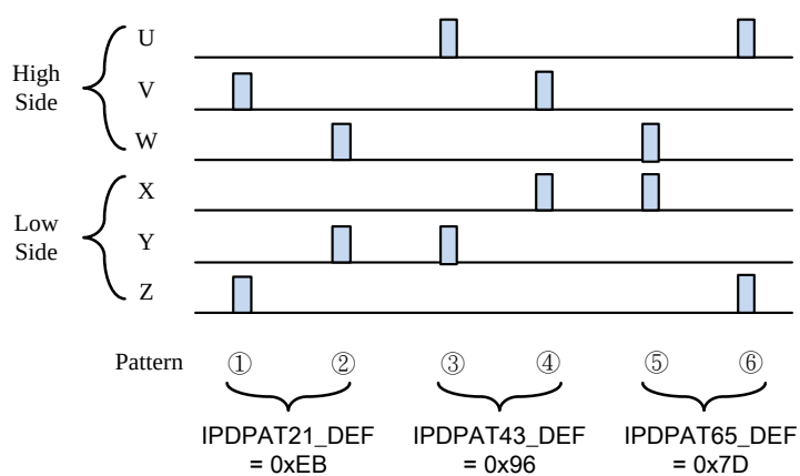
Figure 19.28.3 : IPD pattern high/low side on state initial setting
