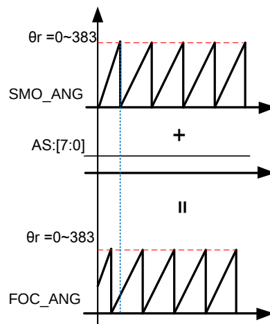
Figure 19.24.4 : Angle Supplement
