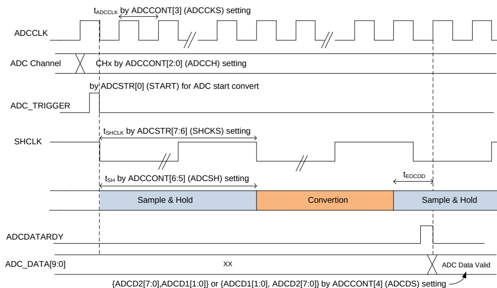
Figure14.1 ADC conversion timing
