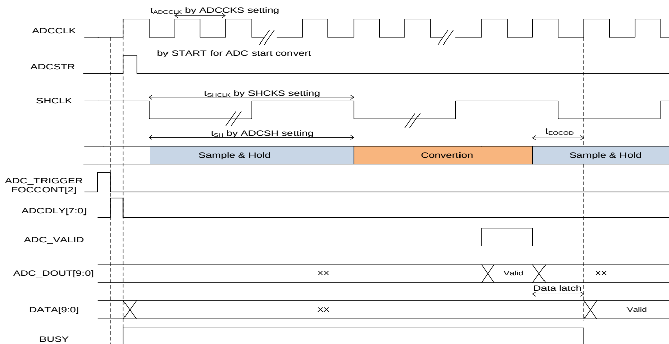
Figure 9.1 A/D Converter Characteristics
