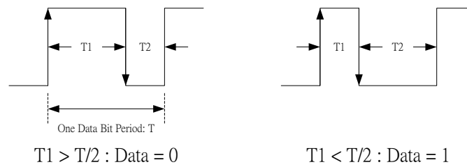
Figure 19.11.2 : The input data type select
