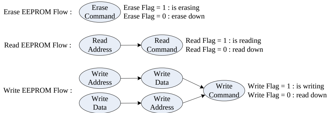
Figure 15.1 : EEPROM Erase, Read, and Write Control Flow
