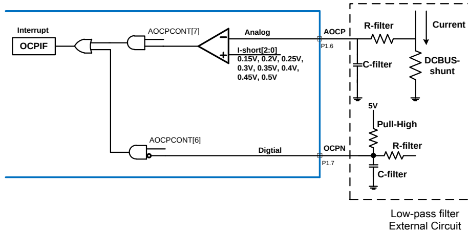
Figure 19.29.1 : Analog OCP and Digital OCPN Unit Architecture
