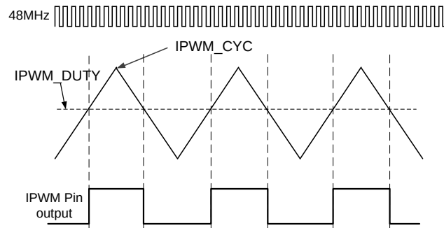
Figure 19.6 : Independent general PWM generator
