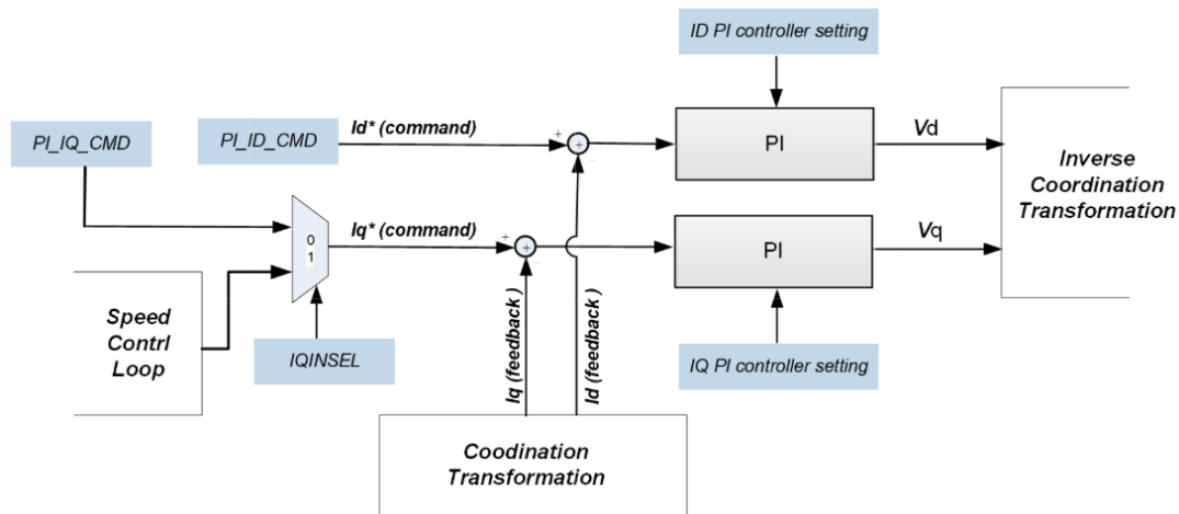
Figure 19.22.1 : Current Control Loop Block Architecture
