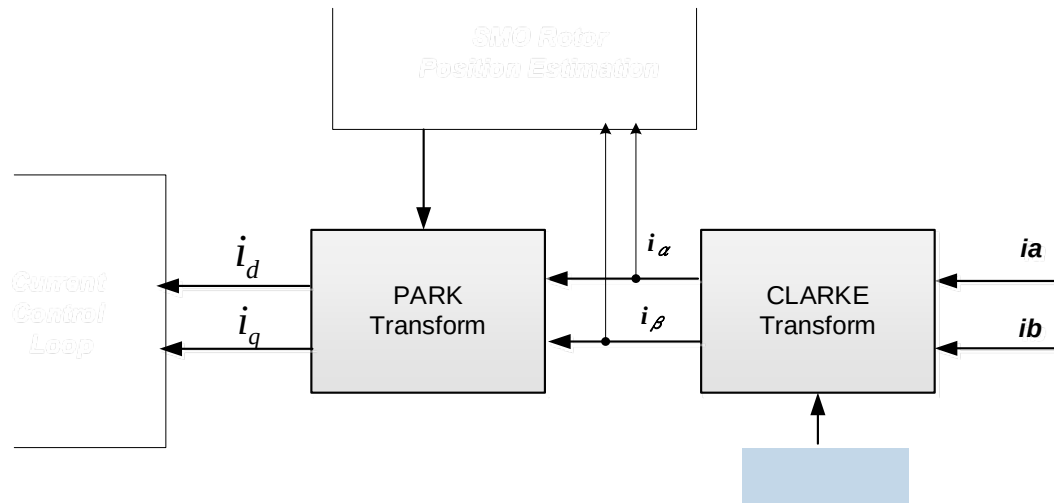
Figure 19.21.1 : Coordinate Transformation Block Architecture
