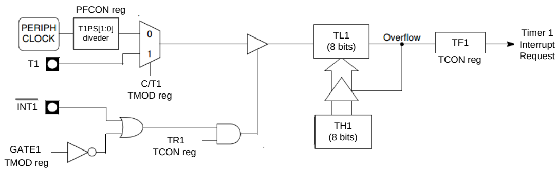
Figure 13.4.11 Timer1 Mode 2
