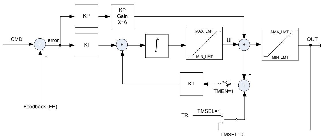
Figure 19.27.1 : PI Block Architecture
