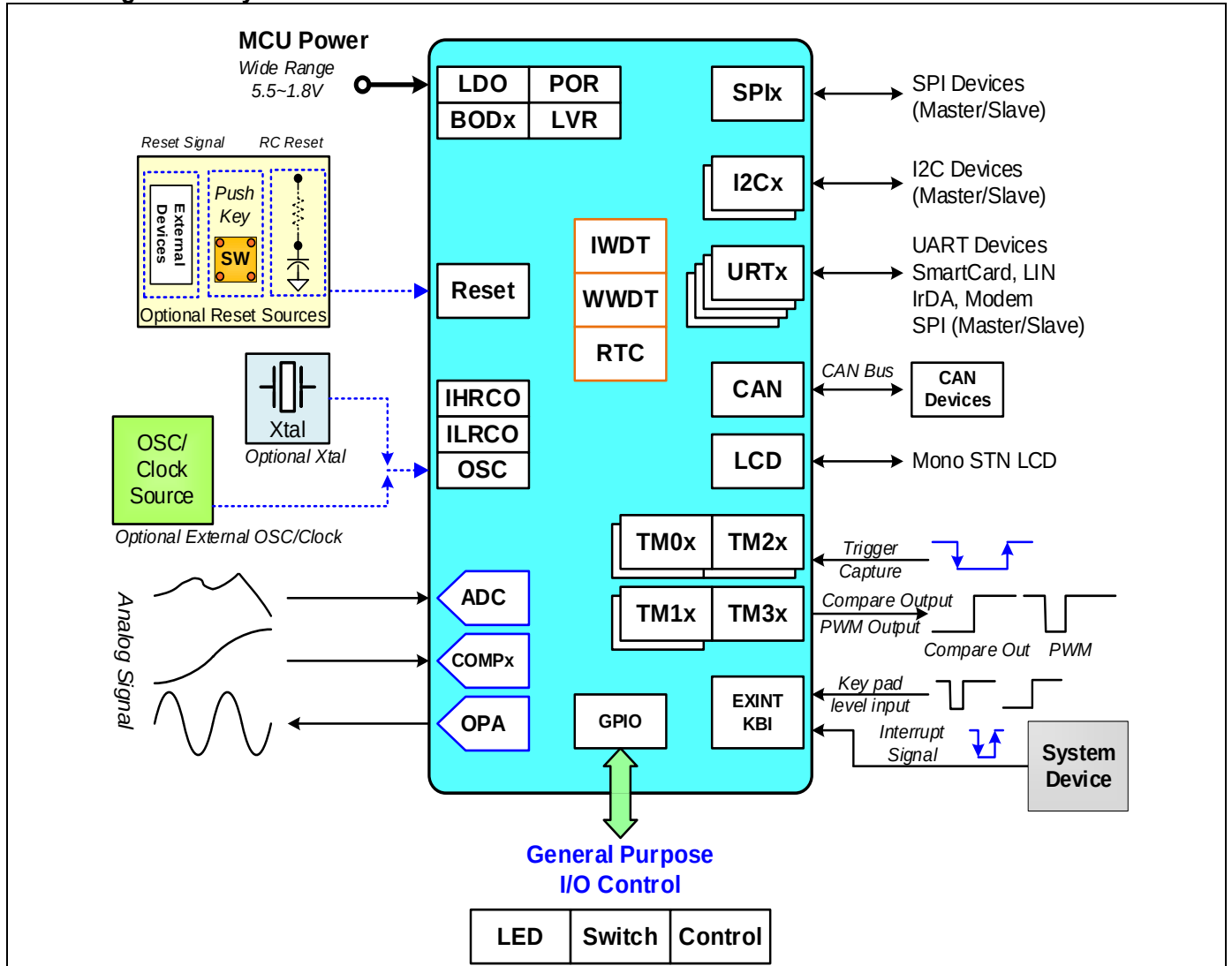
Figure 3-1. System Function Block
