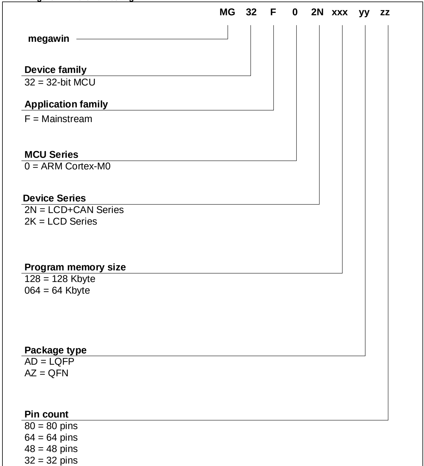
Figure 2-1. Part Numbering
