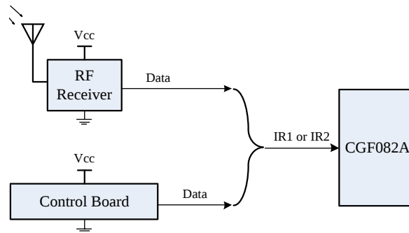
Figure 23.1 : One wire signal decode by CGF082A
