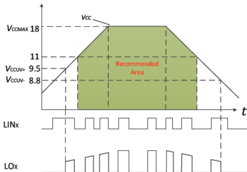
Figure 27.1.1 VCC15 supply UVLO operating area
