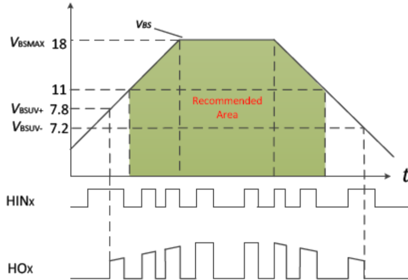
Figure 27.2.1 VBS supply UVLO operating area
