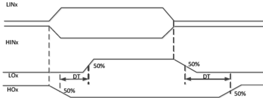
Figure 27.5.1 Dead Time
