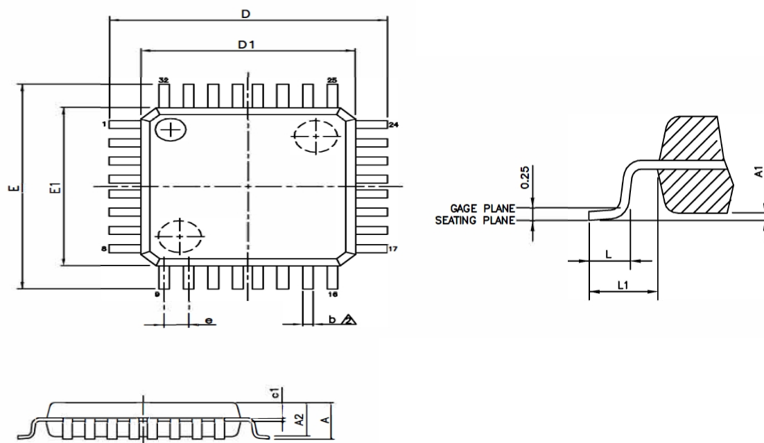
Figure 25–6. LQFP-32
