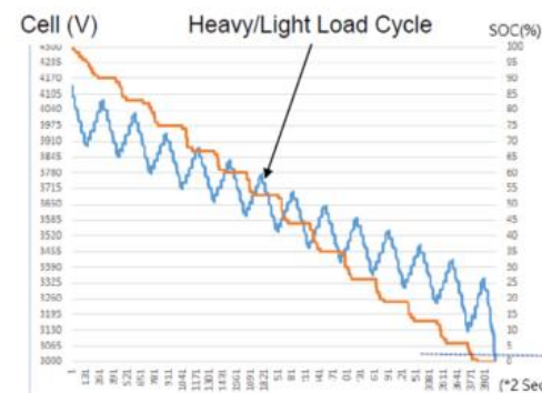
Megawin algorithm smooth the SOC curve
