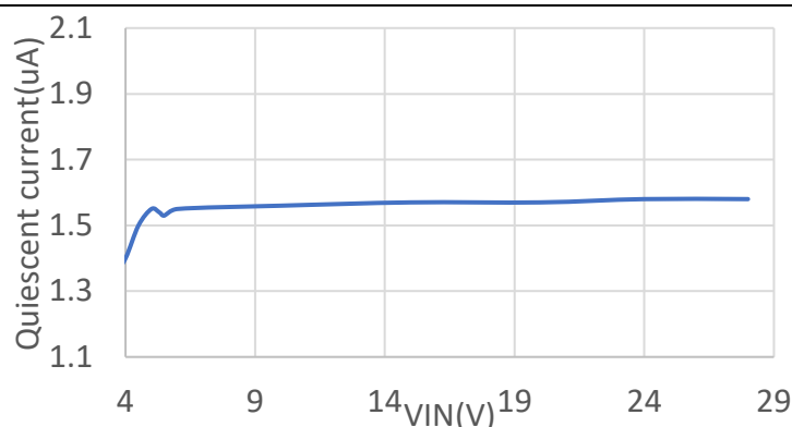
Fig 2. I_Q vs V_{IN}
