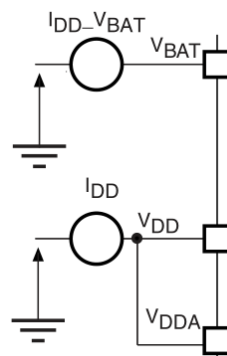
Fig 4.1-4 Current consumption measurement
