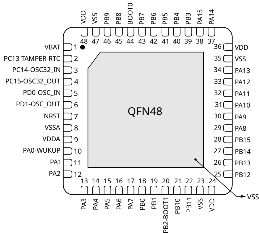
Fig 2.4-1 QFN48 pinouts
