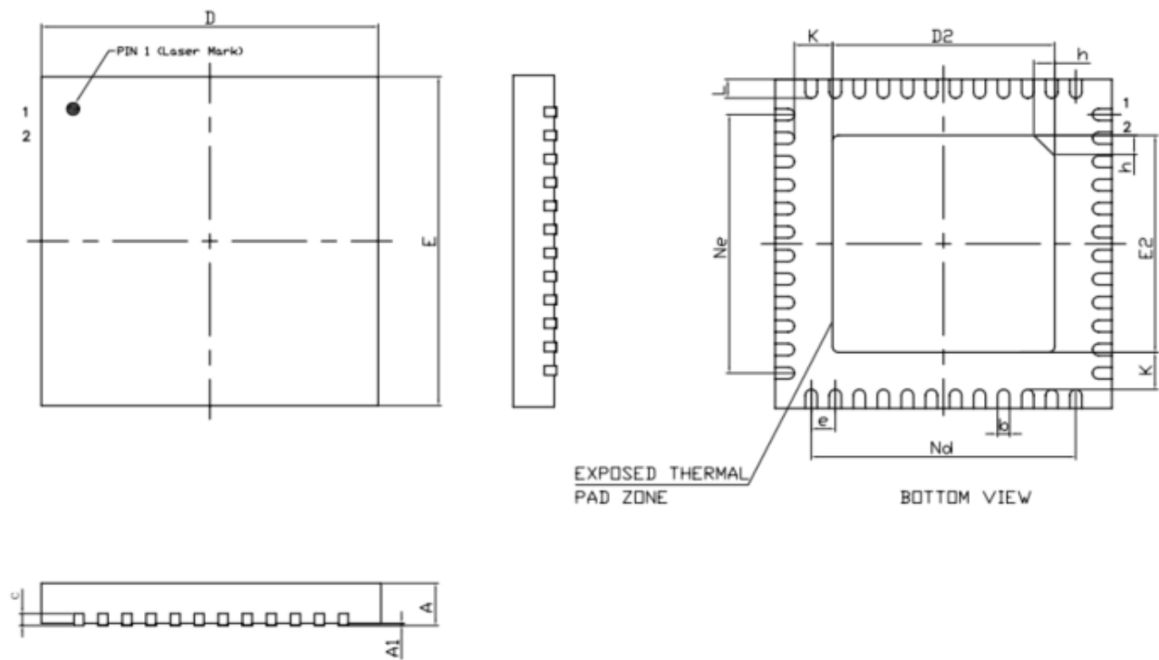
Fig 5.4-1 QFN48 6 x 6mm, 48 pin
