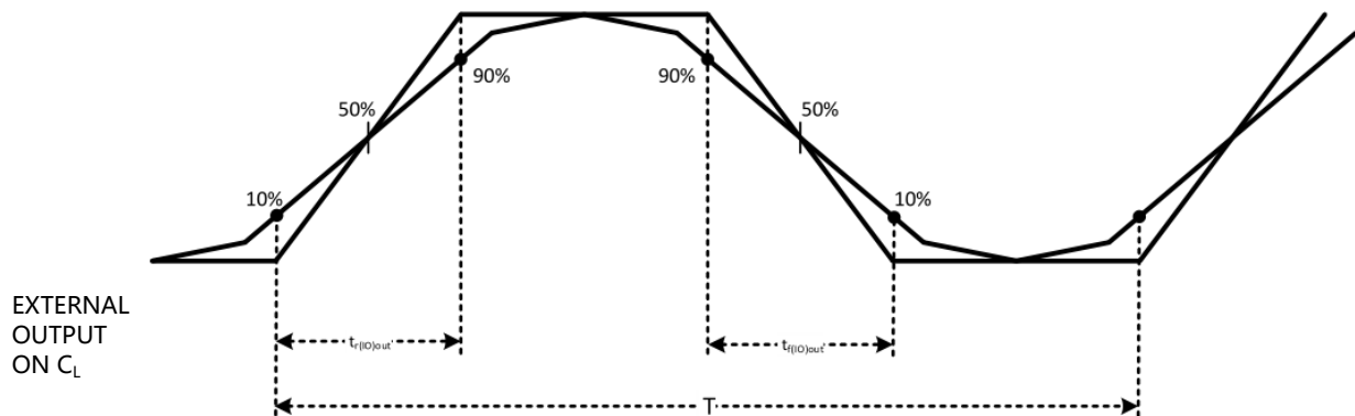
Fig 4.4-3 I/O AC characteristics definition
