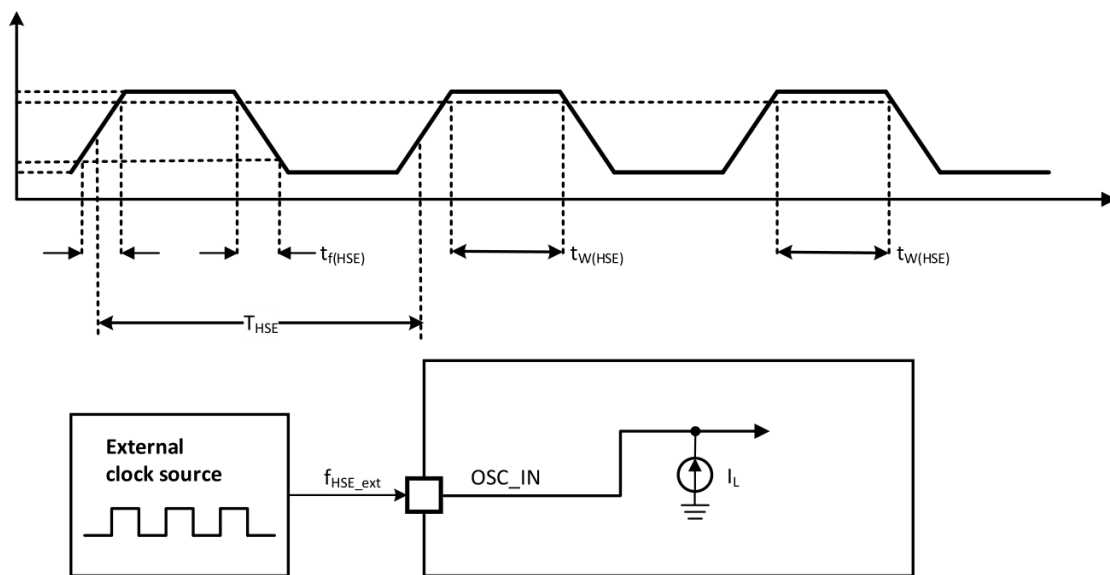
Fig 4.4-1 High-speed external clock source AC timing diagram
