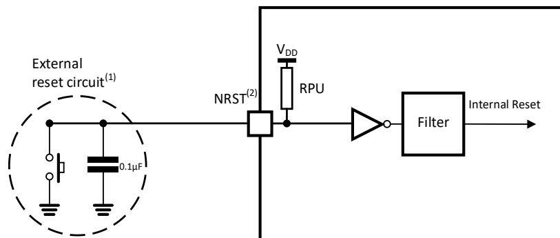
Fig 4.4-4 NRST Pin protection
