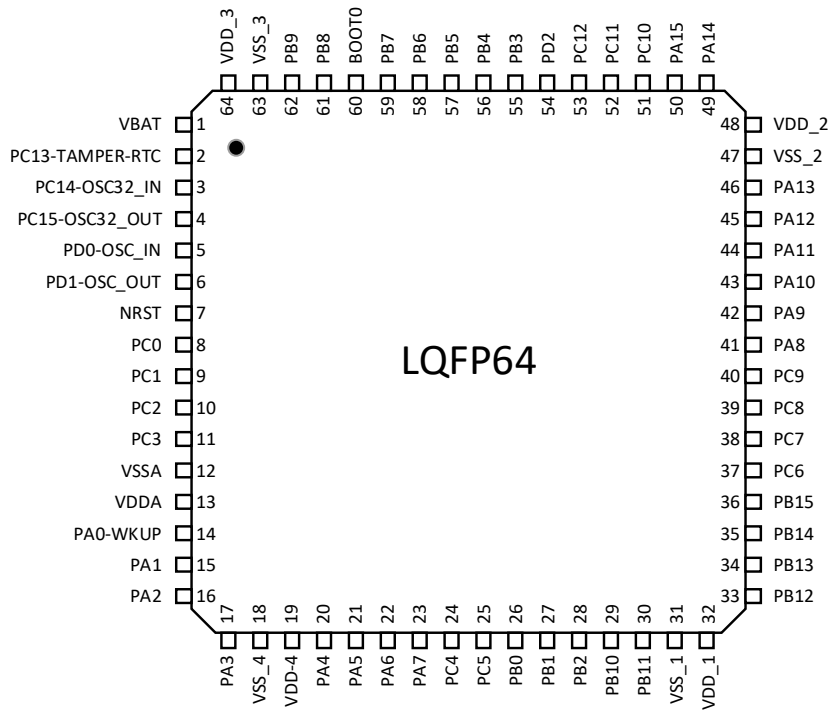
Fig 2.2-1 LQFP64 pinouts
