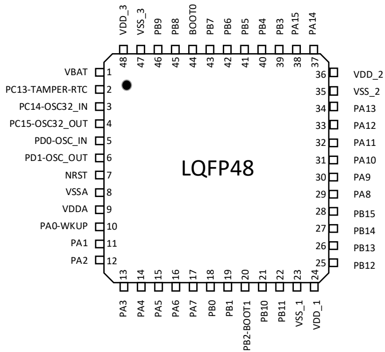
Fig 2.3-1 LQFP48 pinouts
