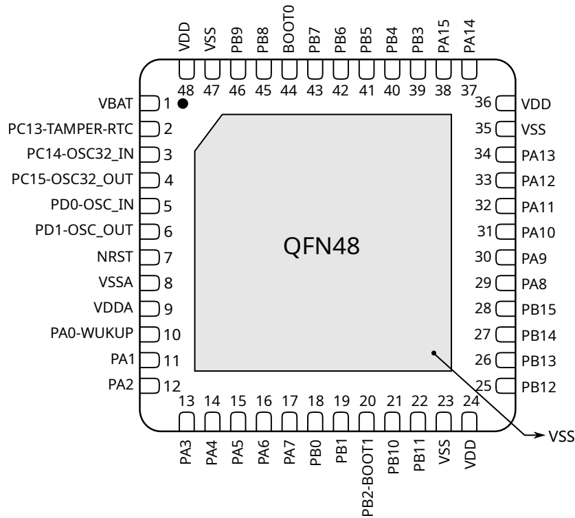
Fig 2.4-1 QFN48 pinouts
