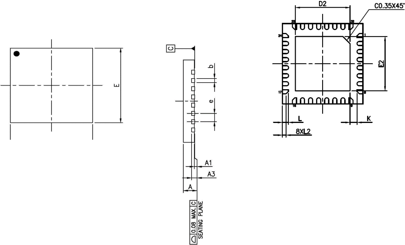
图 16 QFN-32 (4mm X 4mm X 0.55mm)
