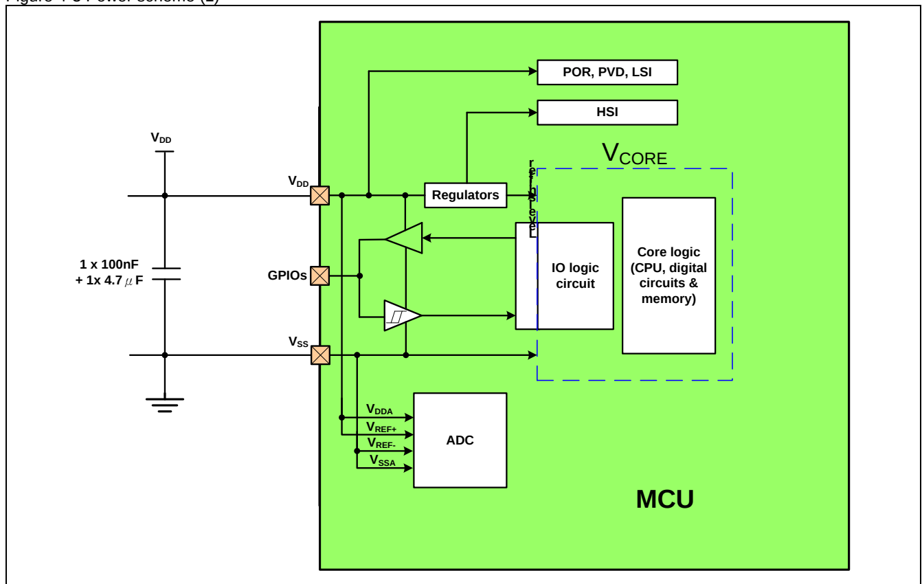
Figure 4-3 Power scheme (1)
