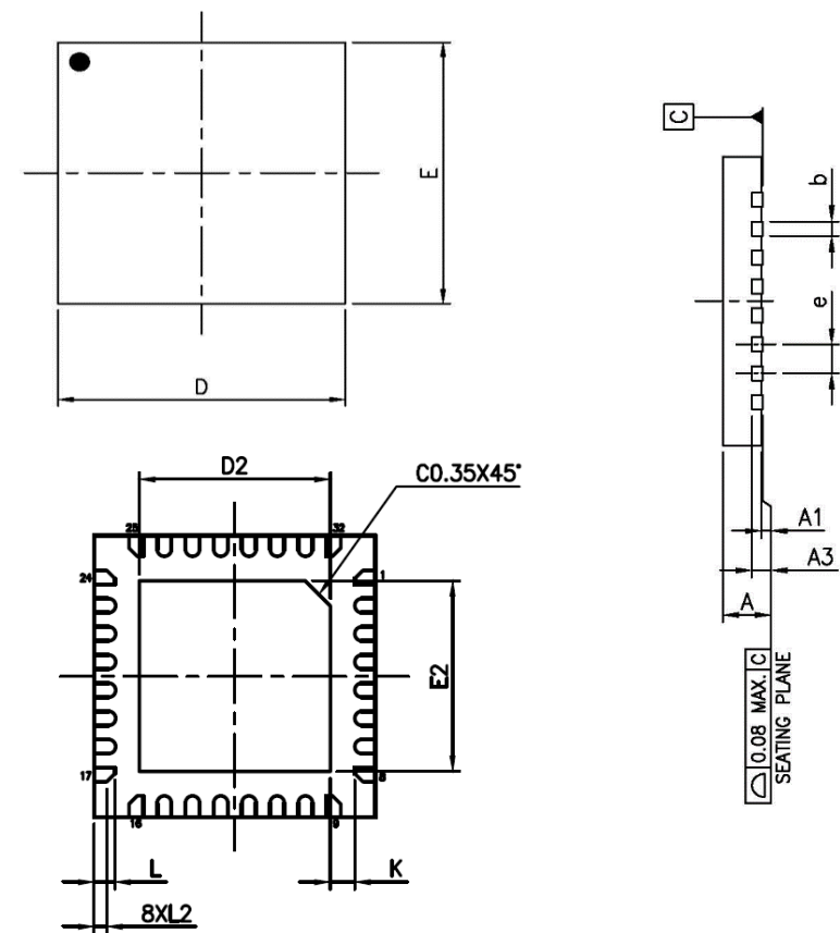
8.2 QFN-32 (4mm X 4mm X 0.55mm) 尺寸 图 16 QFN-32 (4mm X 4mm X 0.55mm) 封装尺寸
