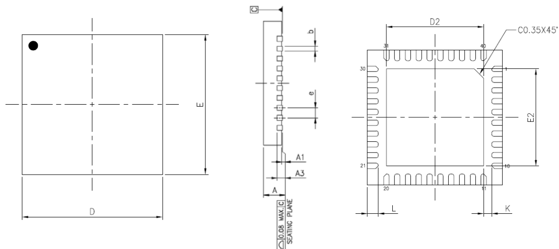
Figure 19 QFN-40 (5mm X 5mm X 0.75mm)
