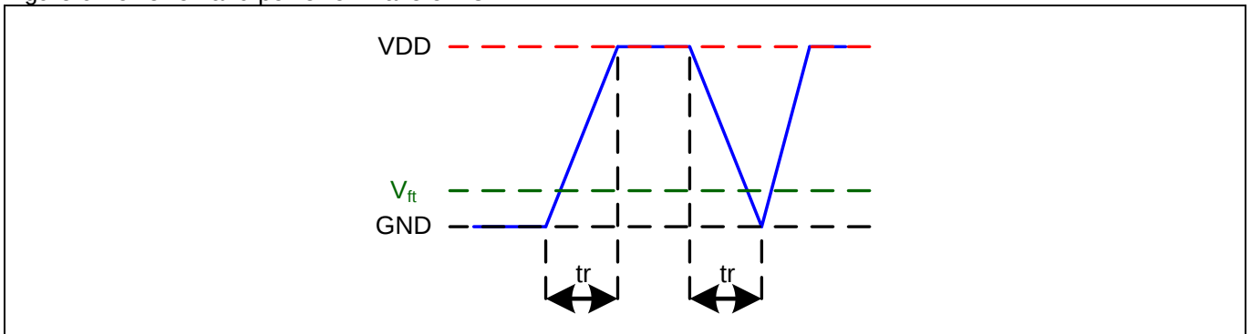
Figure 6 Power-on and power-off waveforms
