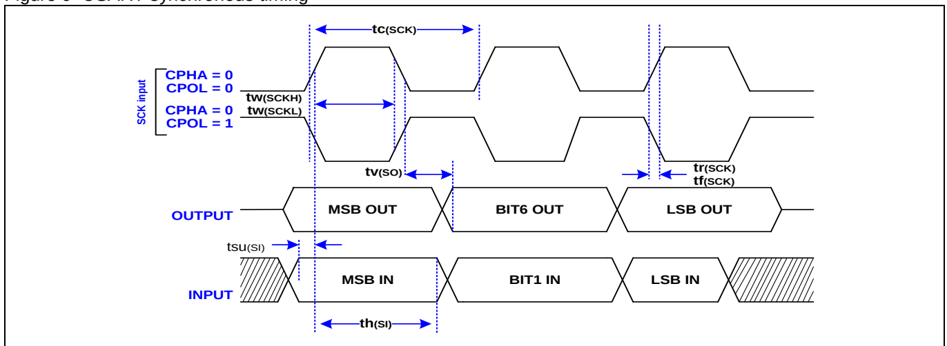
Figure 9 USART synchronous timing
