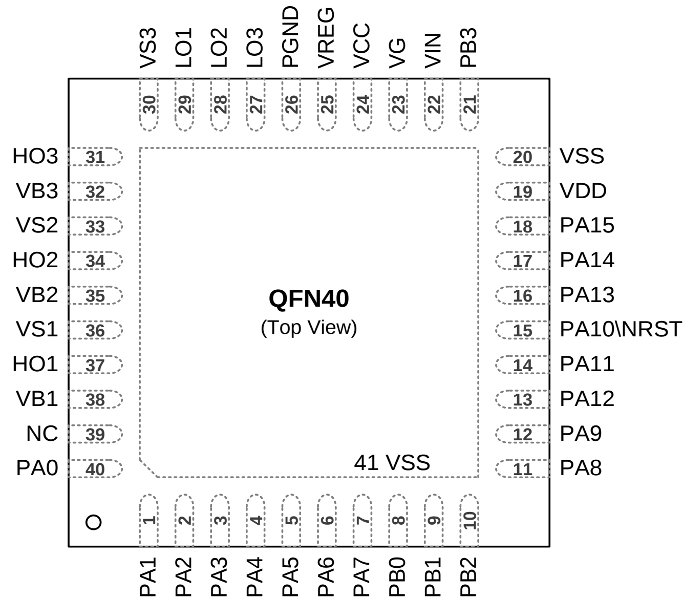
Figure 4 pinout diagram
