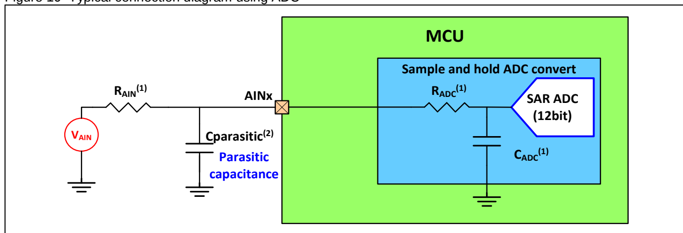
Figure 10 Typical connection diagram using ADC
