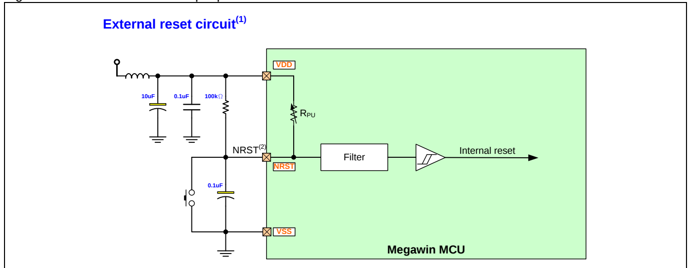
Figure 8 Recommended NRST pin protection
