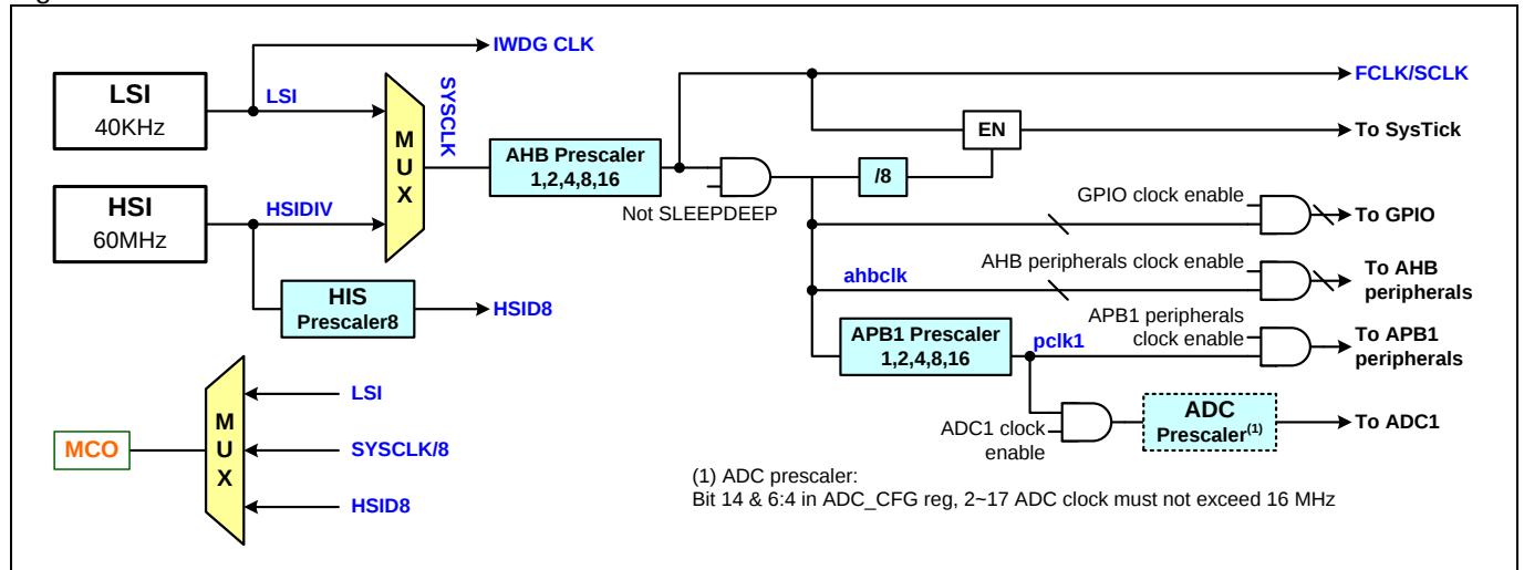
Figure 3 Clock tree
