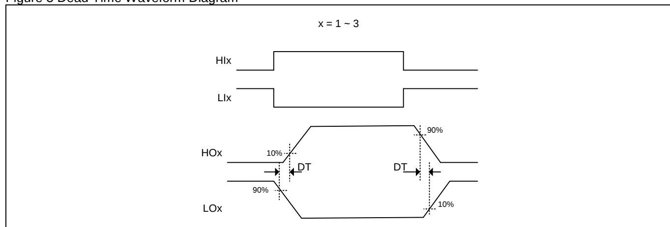
Figure 5 Dead Time Waveform Diagram
