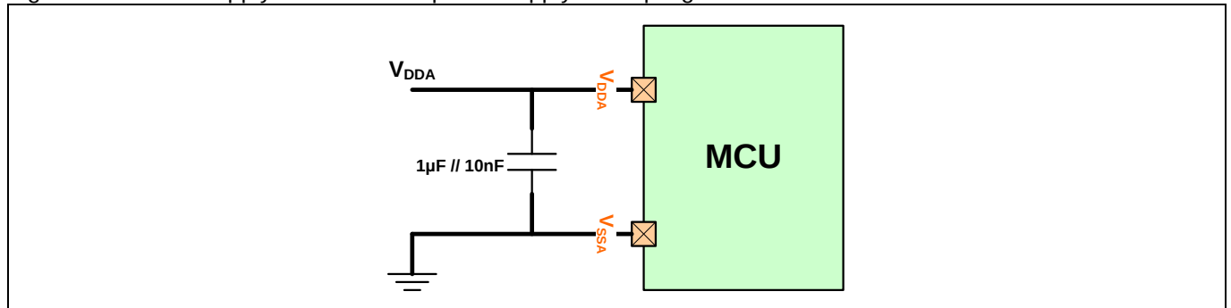
Figure 118 Power supply and reference power supply decoupling circuit
