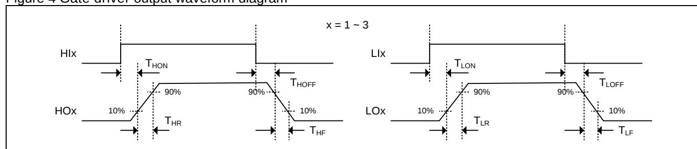
Figure 4 Gate driver output waveform diagram
