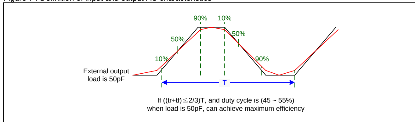
Figure 74 Definition of input and output AC characteristics
