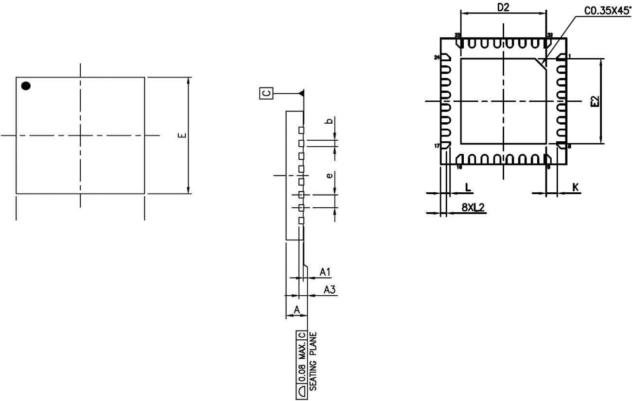
图 15 QFN-32 (4mm X 4mm X 0.55mm)
