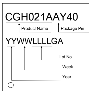
QFN40-5X5x0.75 mm
