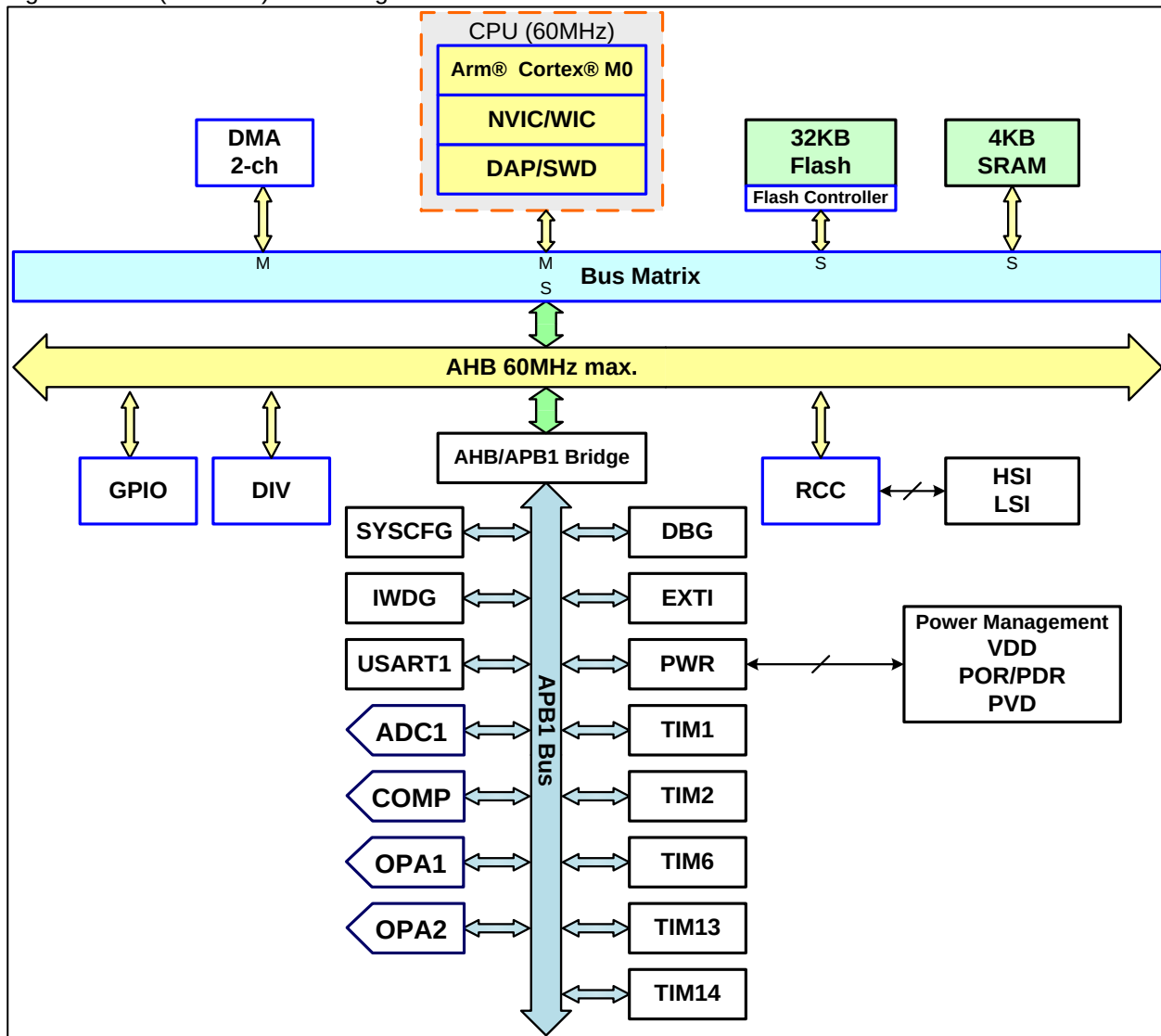
Figure 2 MCU(MDF101) block diagram
