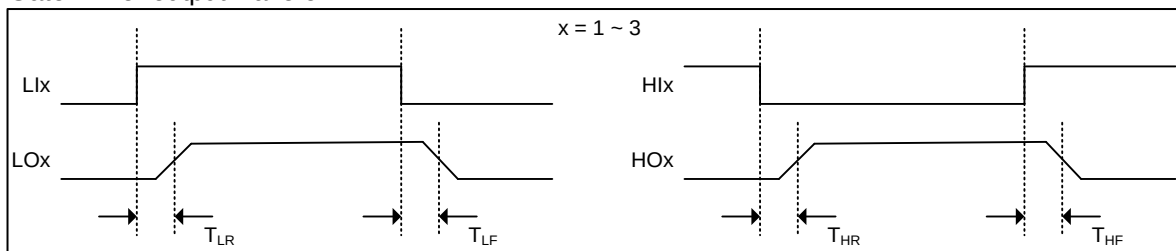
Figure 8 Gate Driver output waveform
