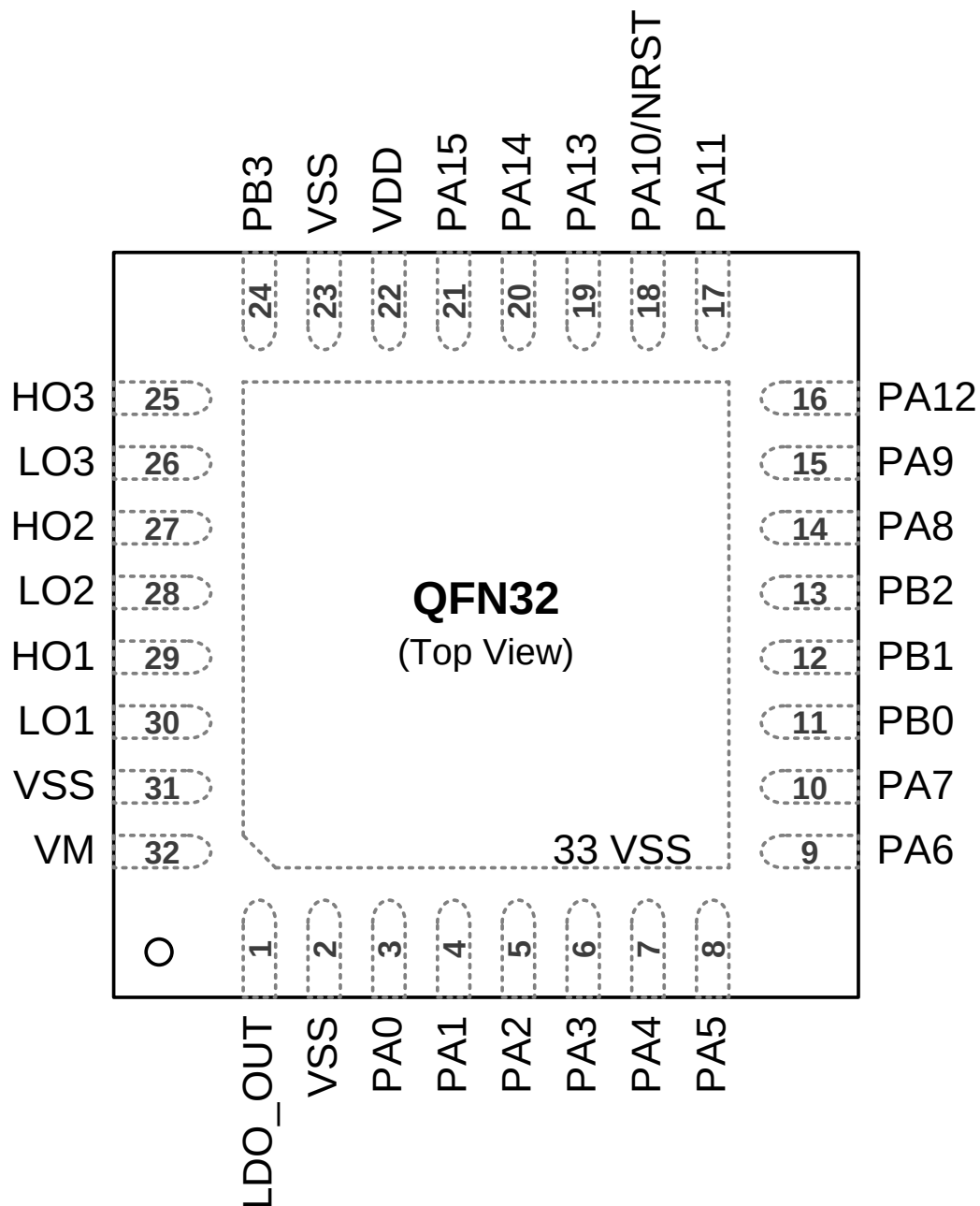
Figure 4 QFN32 pinout diagram
