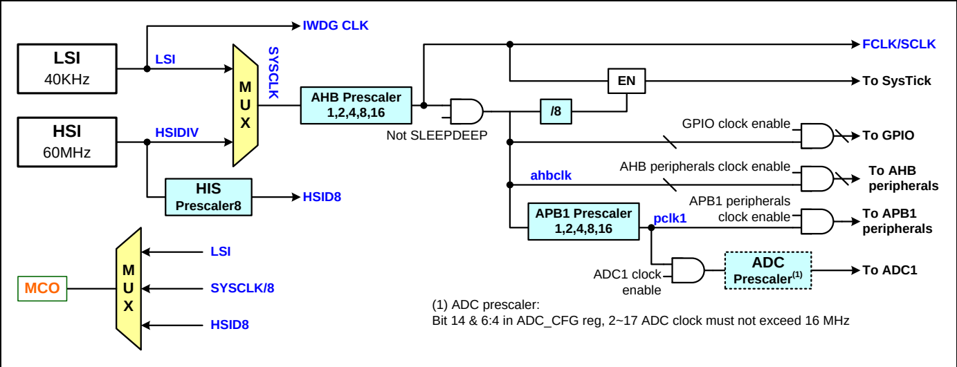
Figure 3 Clock tree
