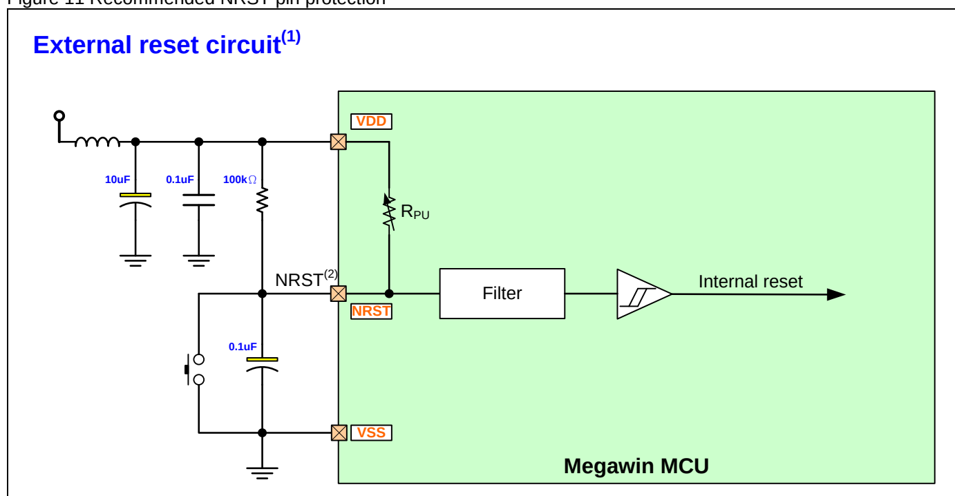
Figure 11 Recommended NRST pin protection
