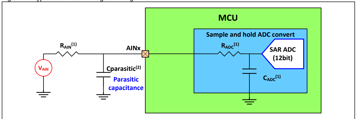
Figure 13 Typical connection diagram using ADC
