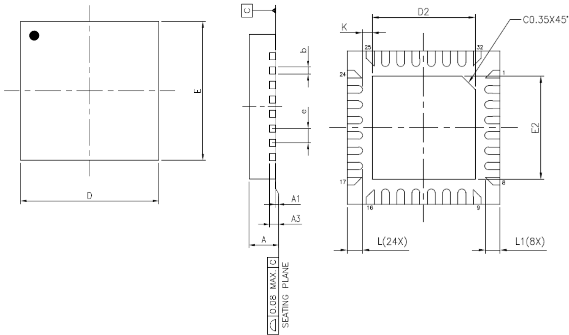
Figure 15 QFN-32 (4mm X 4mm X 0.85mm)
