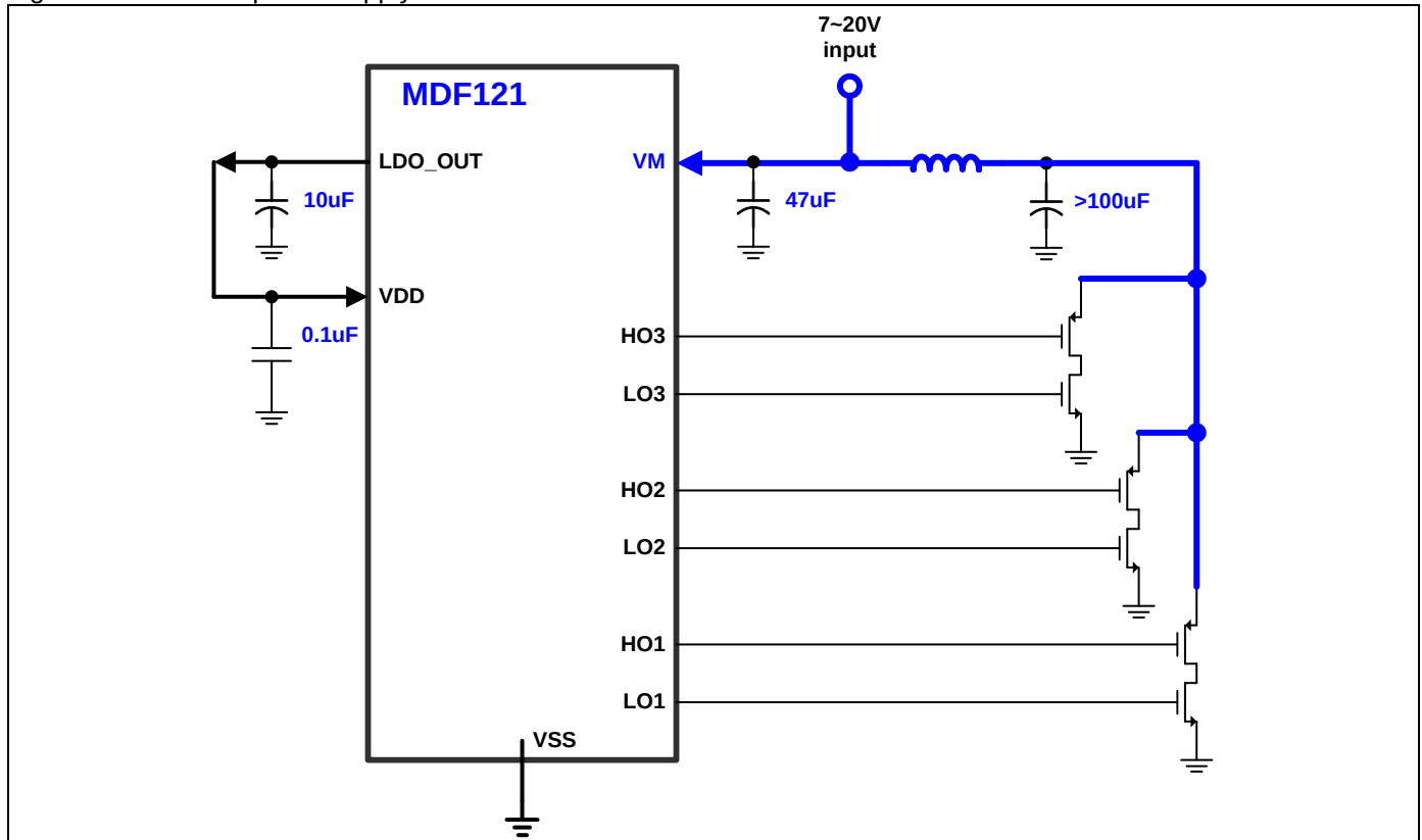
Figure 7 Scheme of power supply
