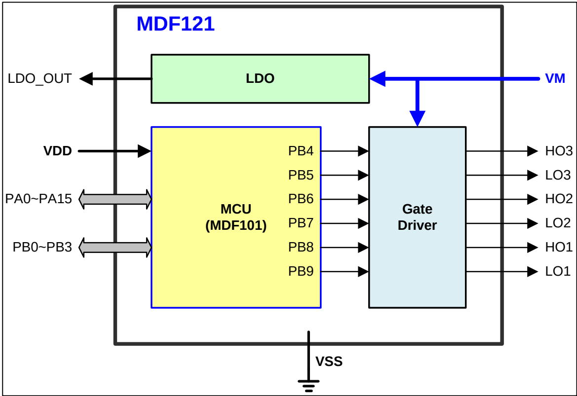
Figure 1 Block diagram
