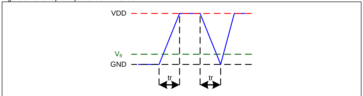
Figure 9 Power-up and power-down waveform
