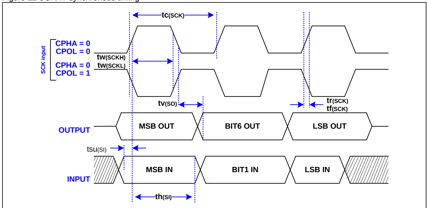
Figure 12 USART synchronous timing
