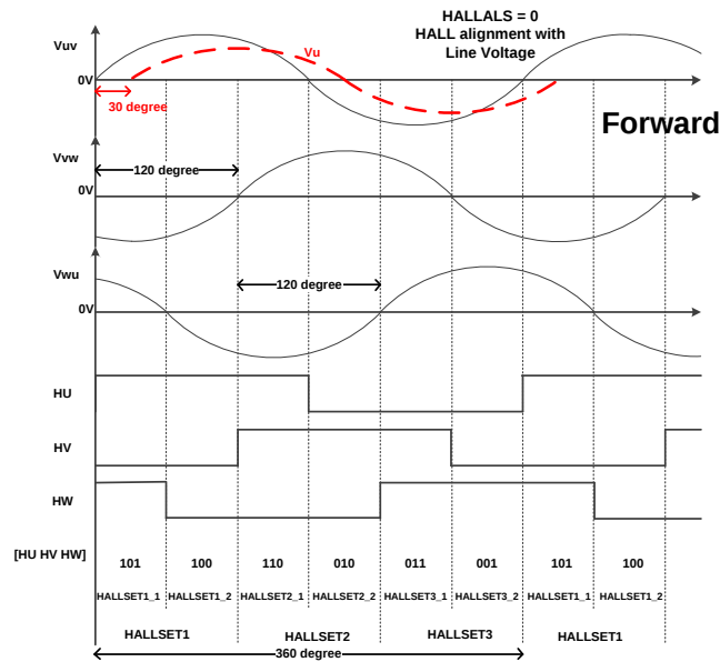
Figure 19.3.2 HALLSET (Hall Setting Register 1, 2, 3)
