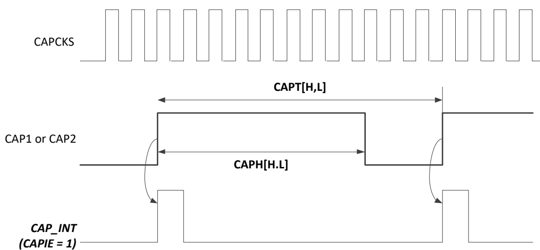
Figure 16.1 Capture
