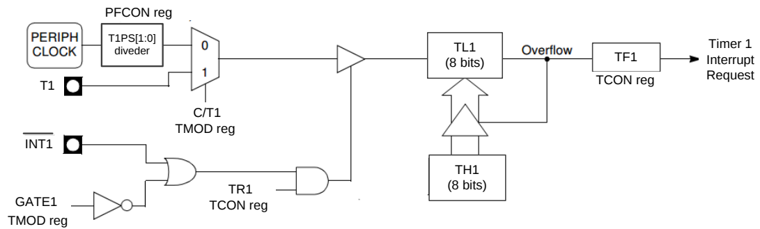
Figure 13.4.11 Timer1 Mode 2
