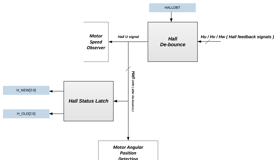
Figure 19.1.1 : Hall I/F Processor Architecture
