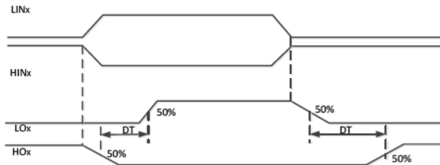
Figure 20.4.1 Dead Time
