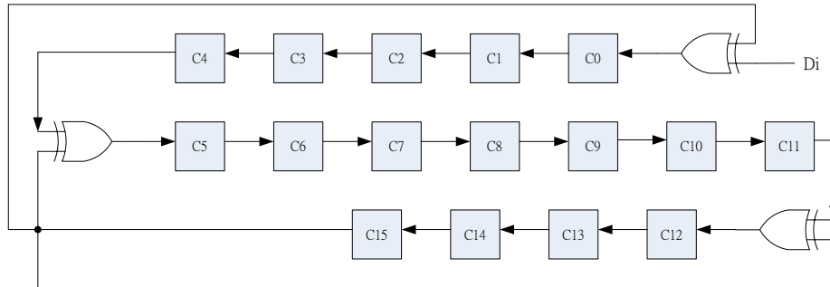
Figure 21.1 : The general LSFR architecture of CRC16-CCITT
