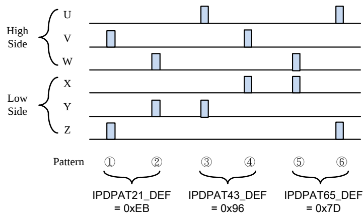
Figure 25.9.3 : IPD pattern high/low side on state initial setting
