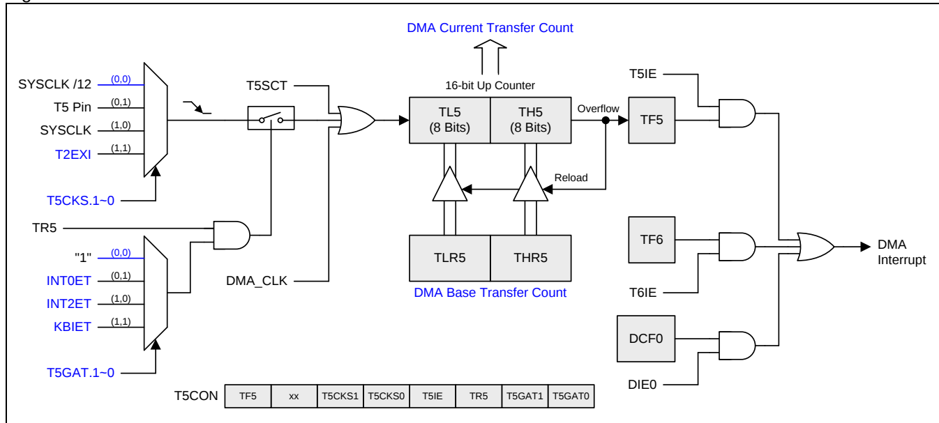
Figure 8–4. Timer 5 Structure
