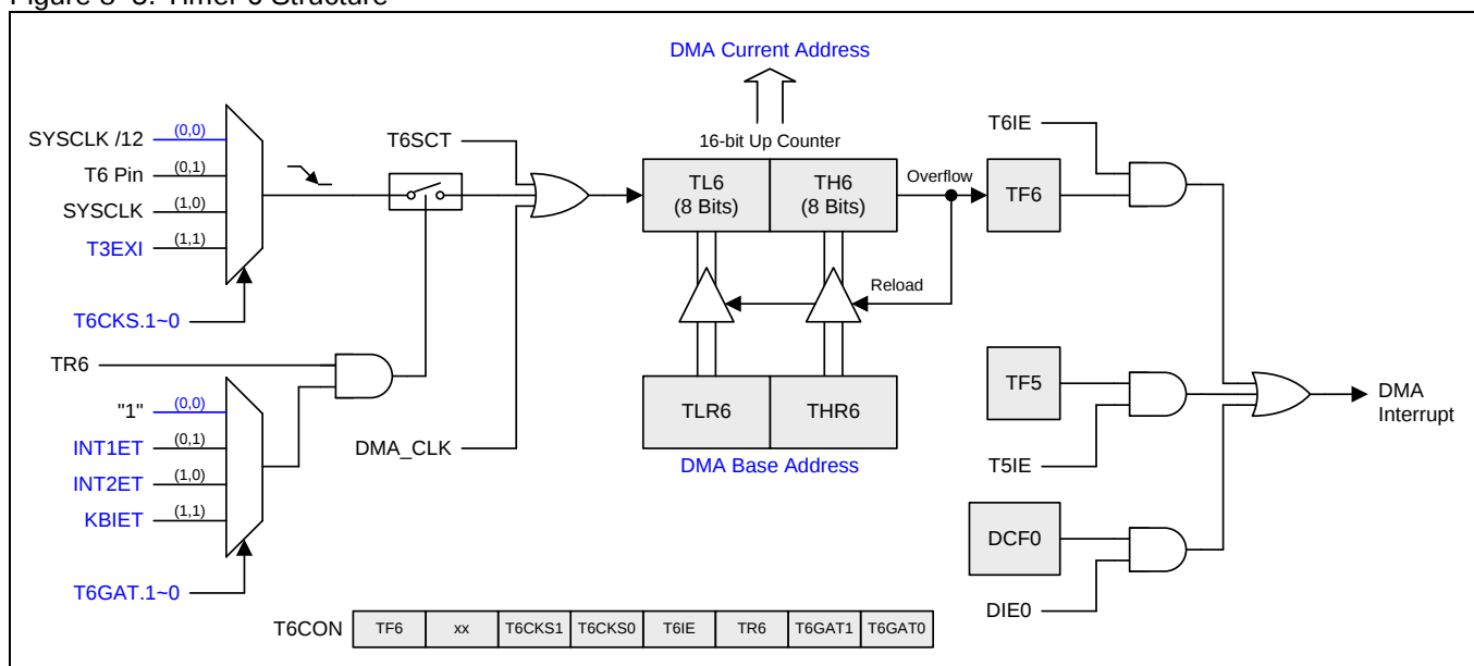
Figure 8–5. Timer 6 Structure
