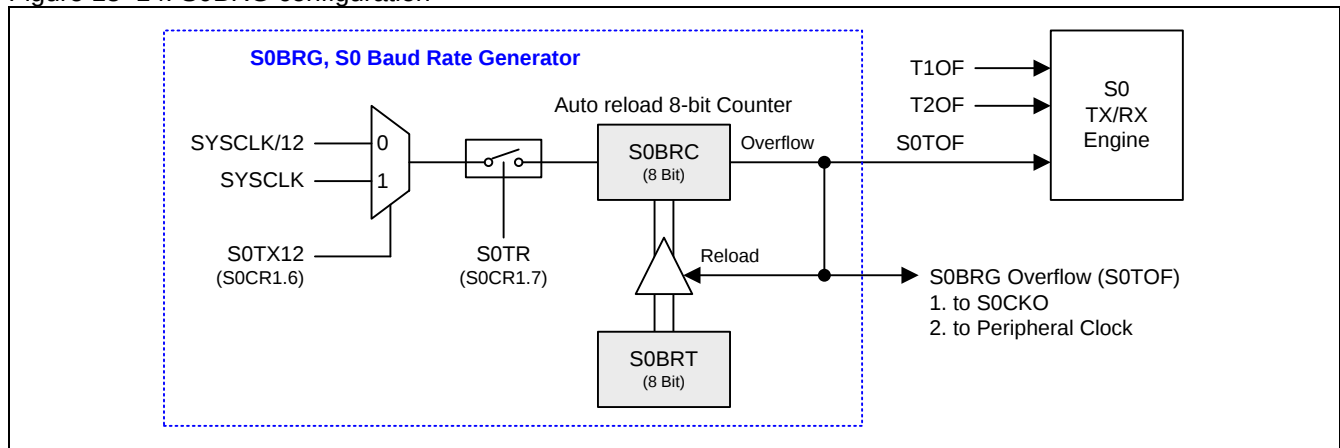
Figure 18–14. S0BRG configuration
