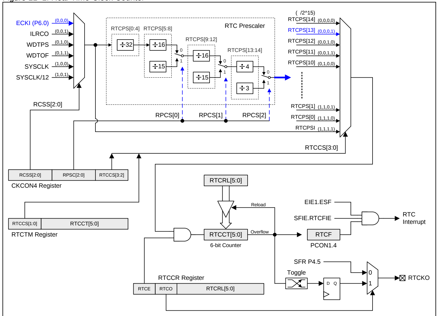
Figure 11–1. Real-Time-Clock Counter
