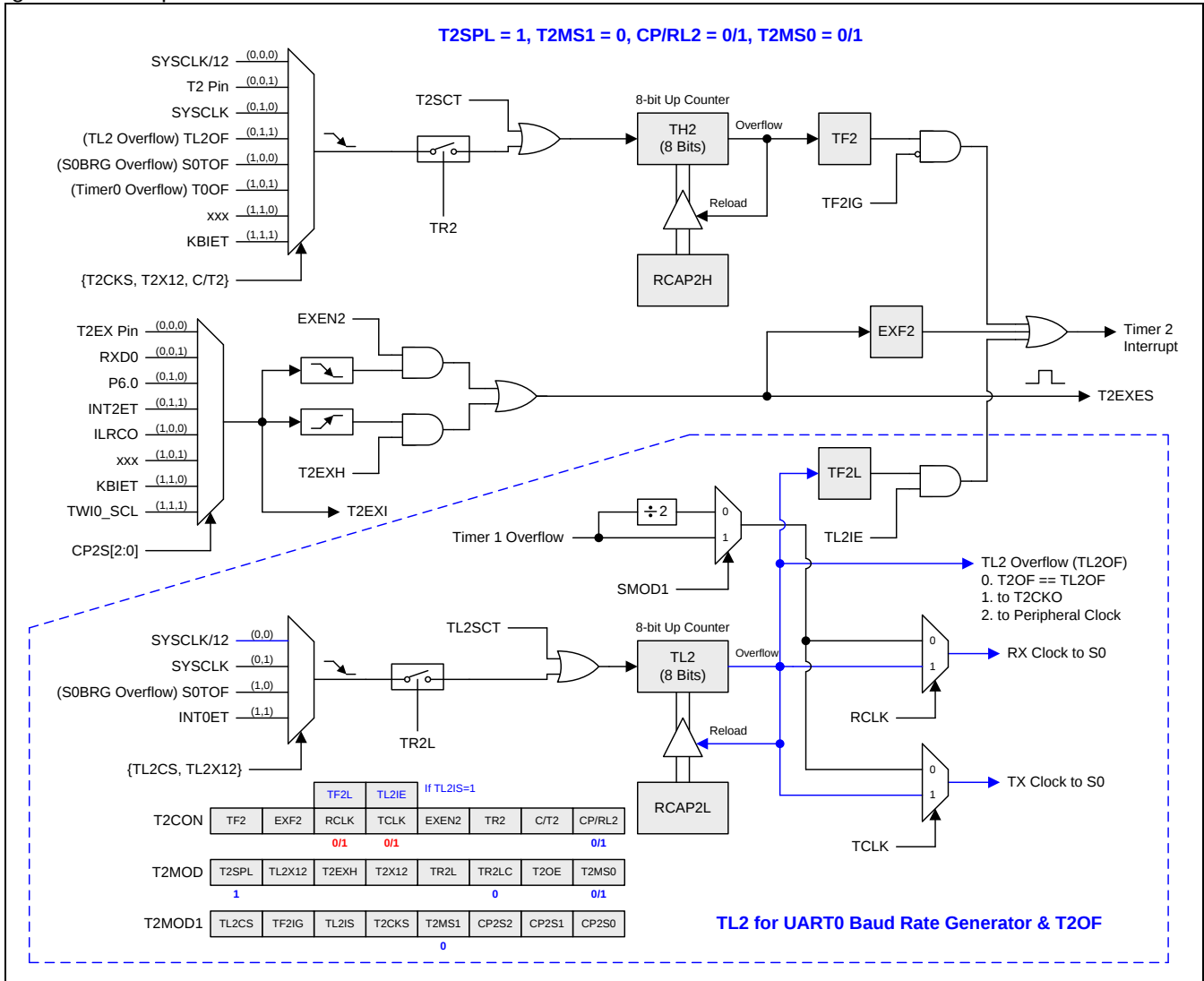
Figure 16–22. Split Timer 2 in Baud-Rate Generator Mode
