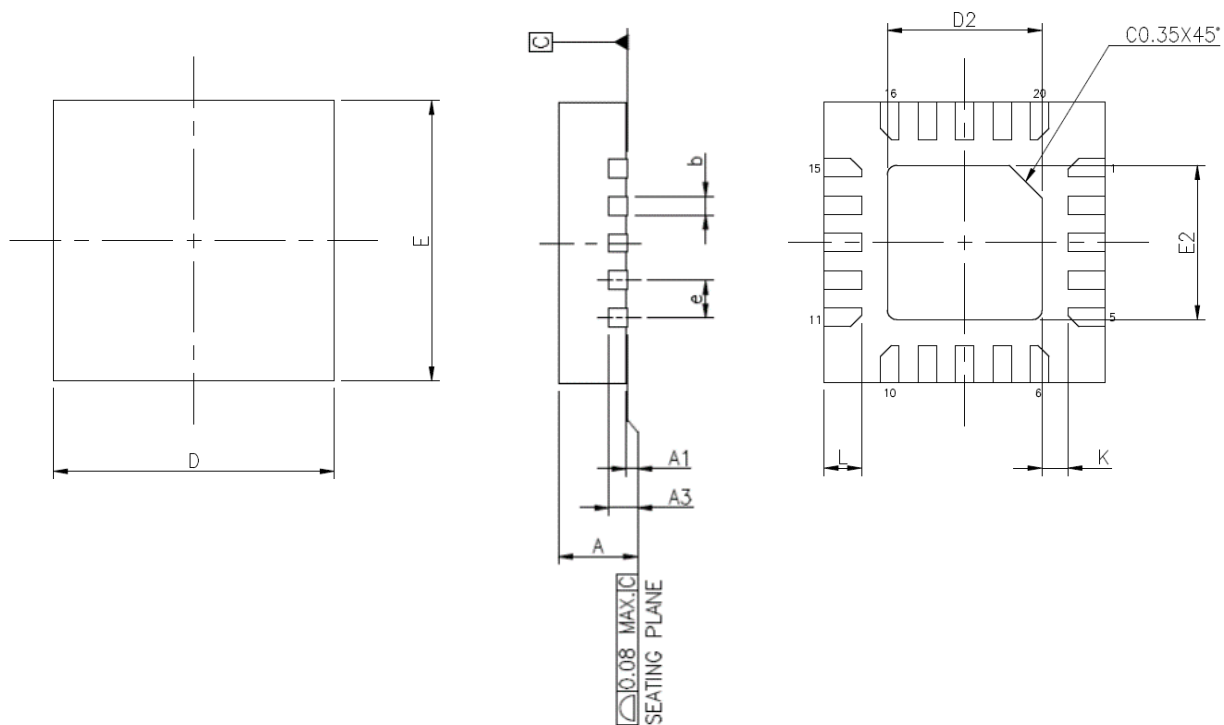
Figure 35-3. QFN-20 (3x3 x 0.75mm ) Package Dimension
