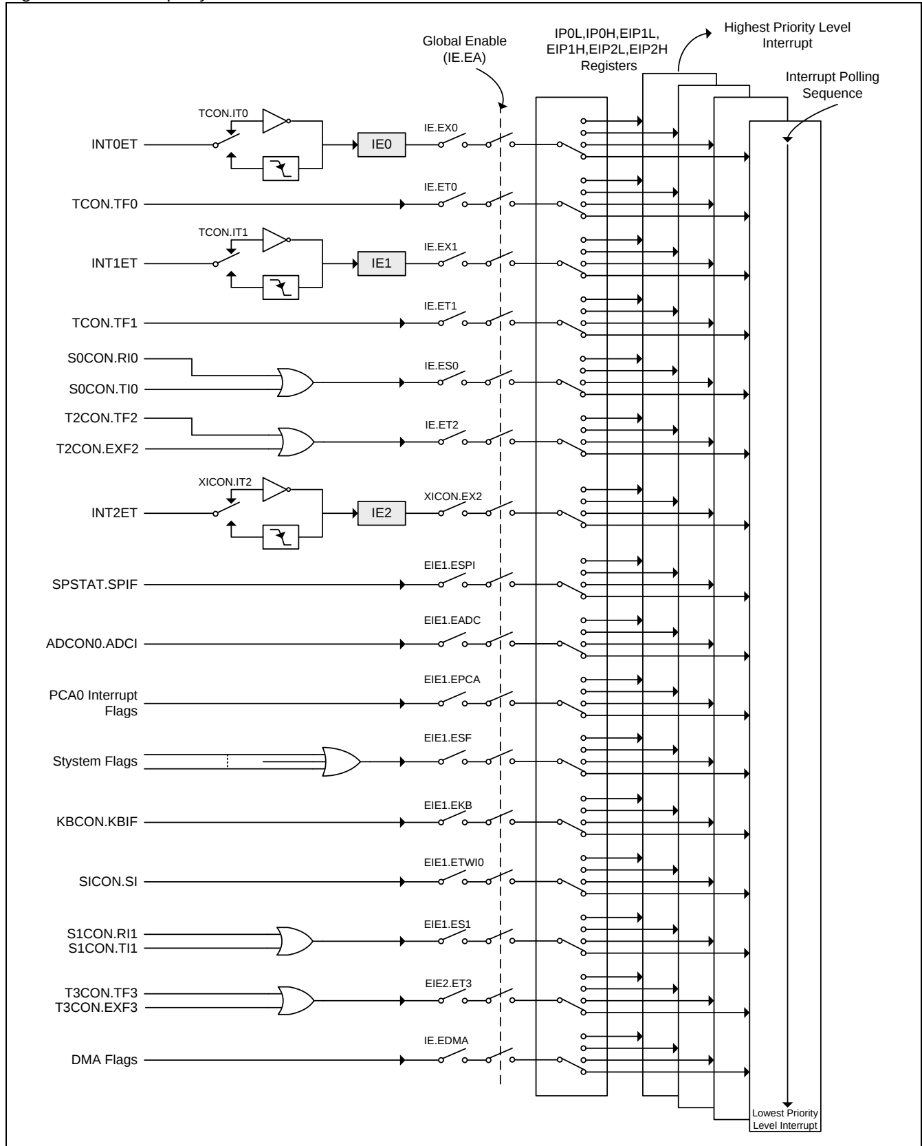
Figure 15–1. Interrupt System
