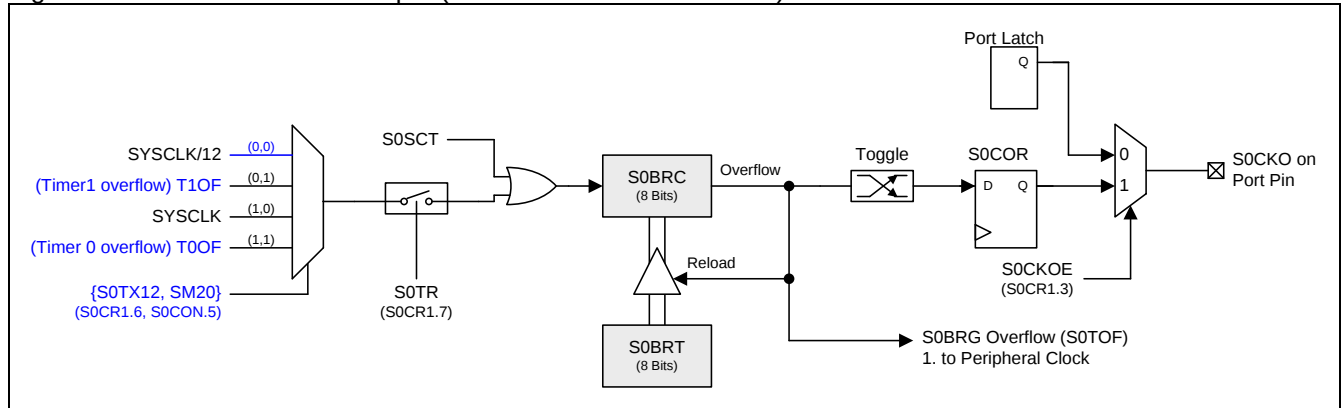
Figure 18–18. S0BRG Clock Output (S0BRG in 8-bit Timer Mode)
