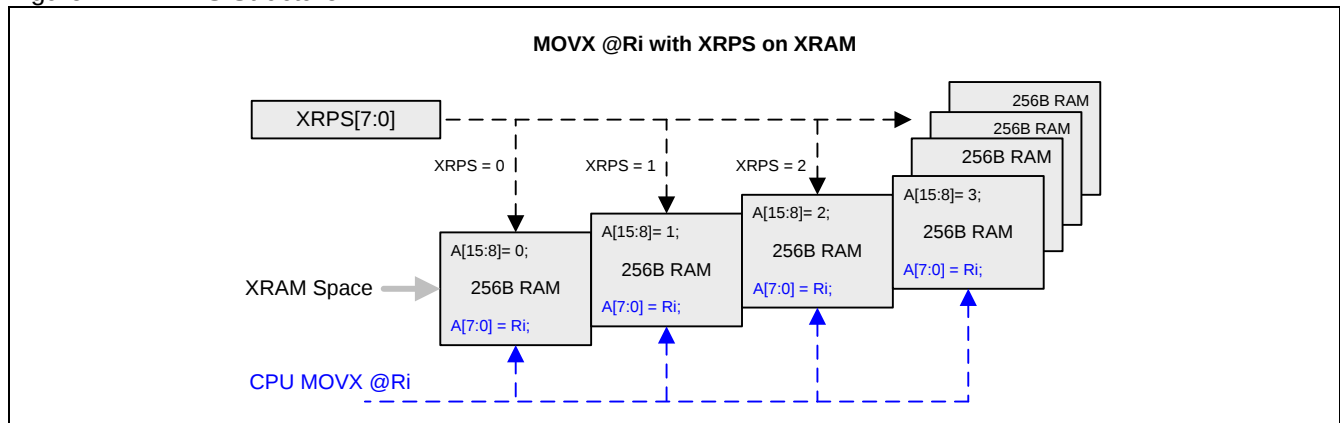
Figure 7–2. XRPS Structure
