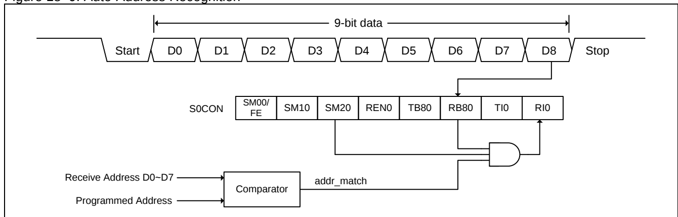
Figure 18–9. Auto-Address Recognition
