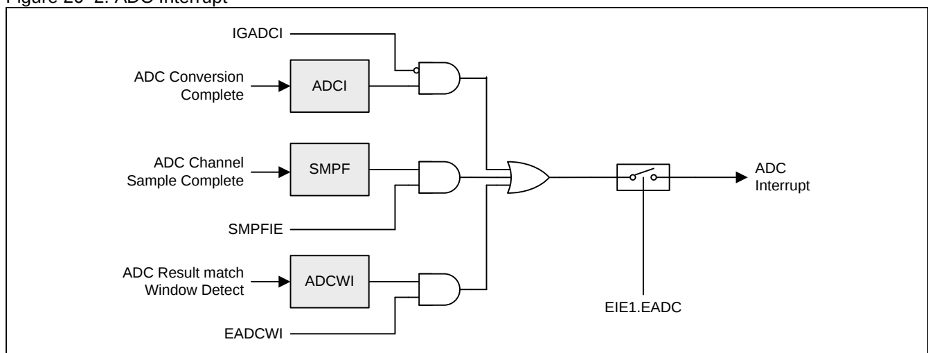
Figure 26–2. ADC Interrupt
