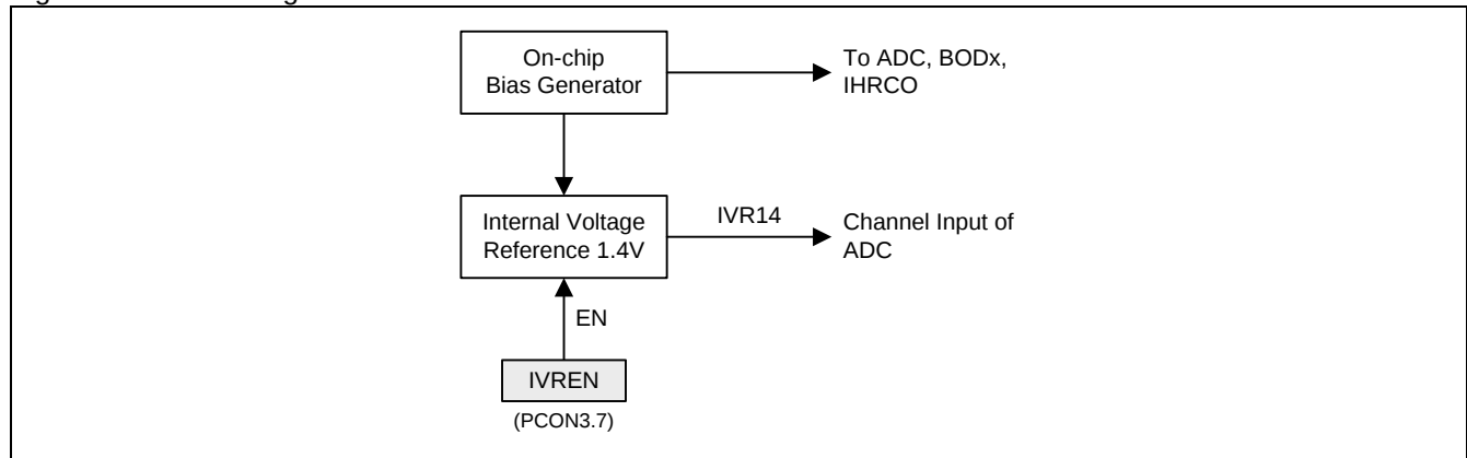
Figure 27–1. IVR Diagram
