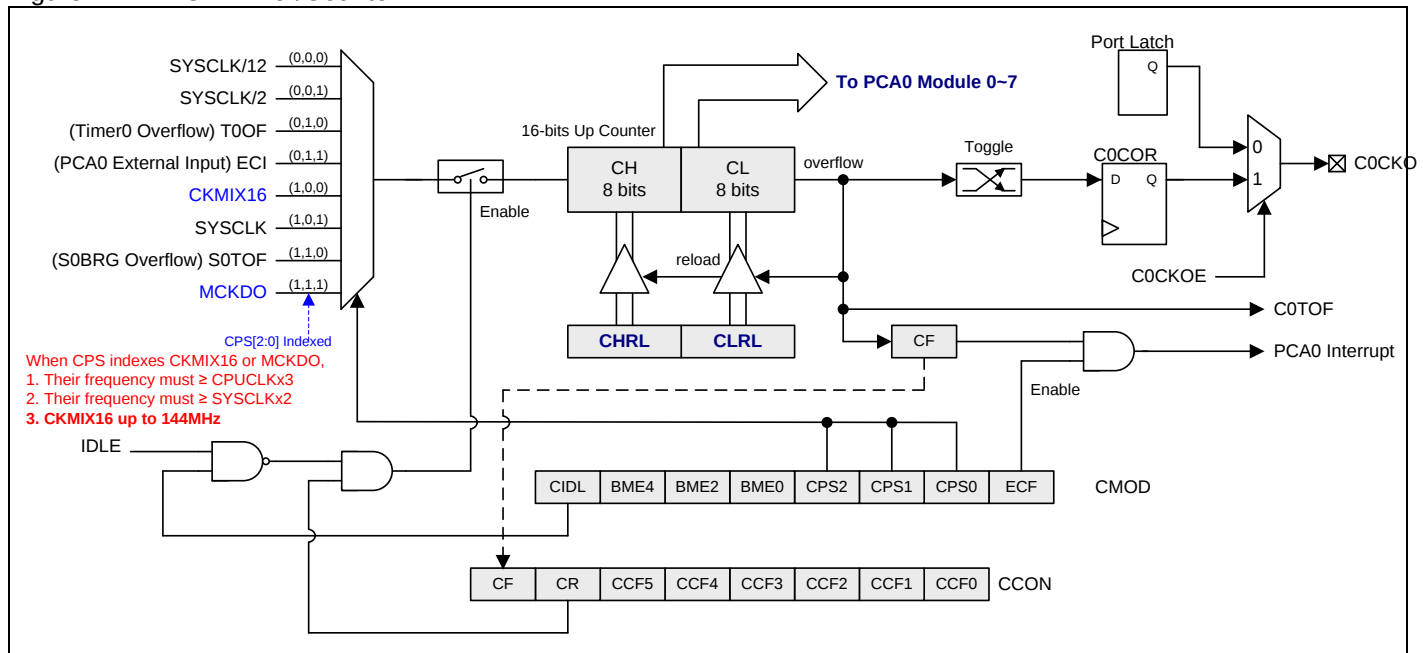
Figure 17–2. PCA Timer/Counter
