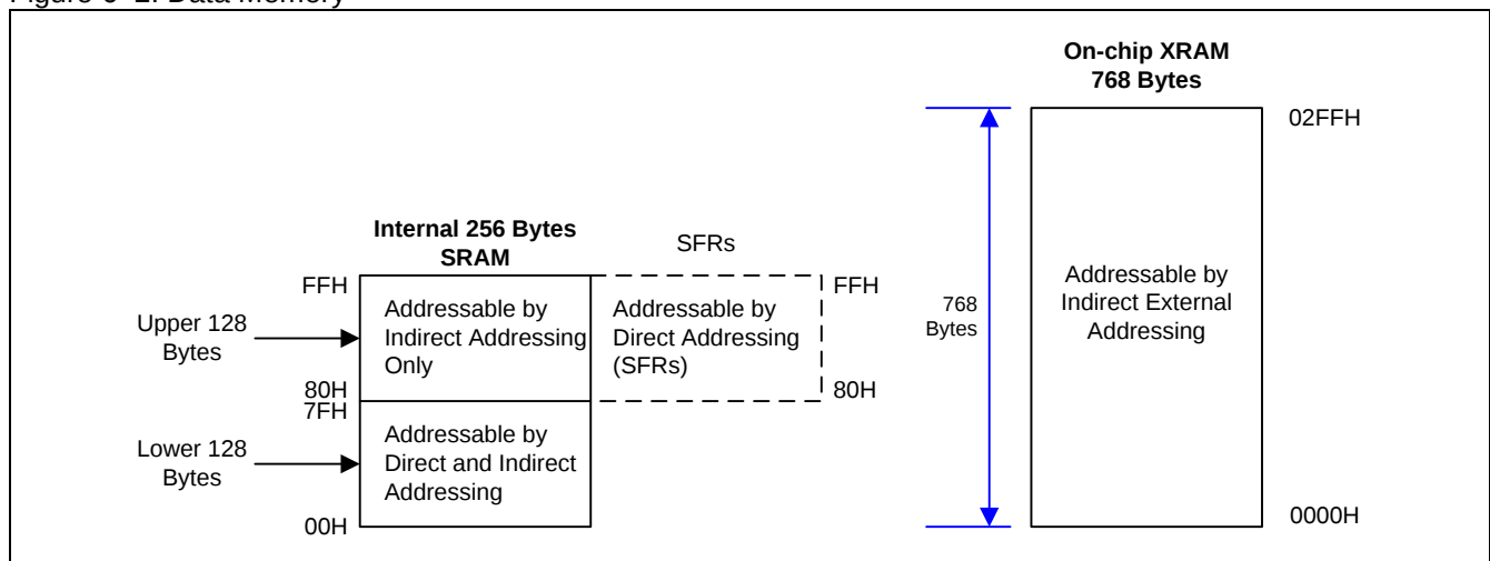
Figure 6–2. Data Memory
