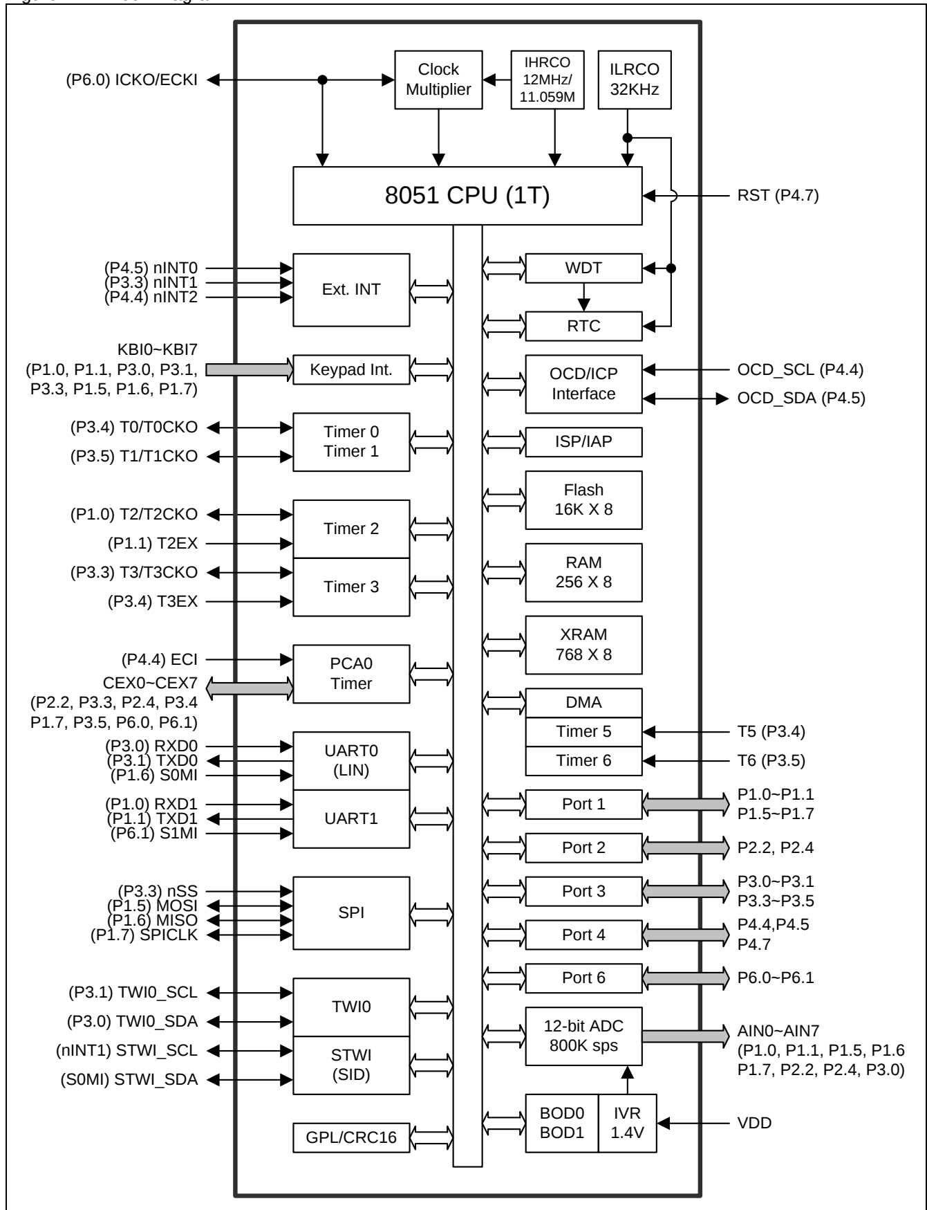
Figure 2–1. Block Diagram
