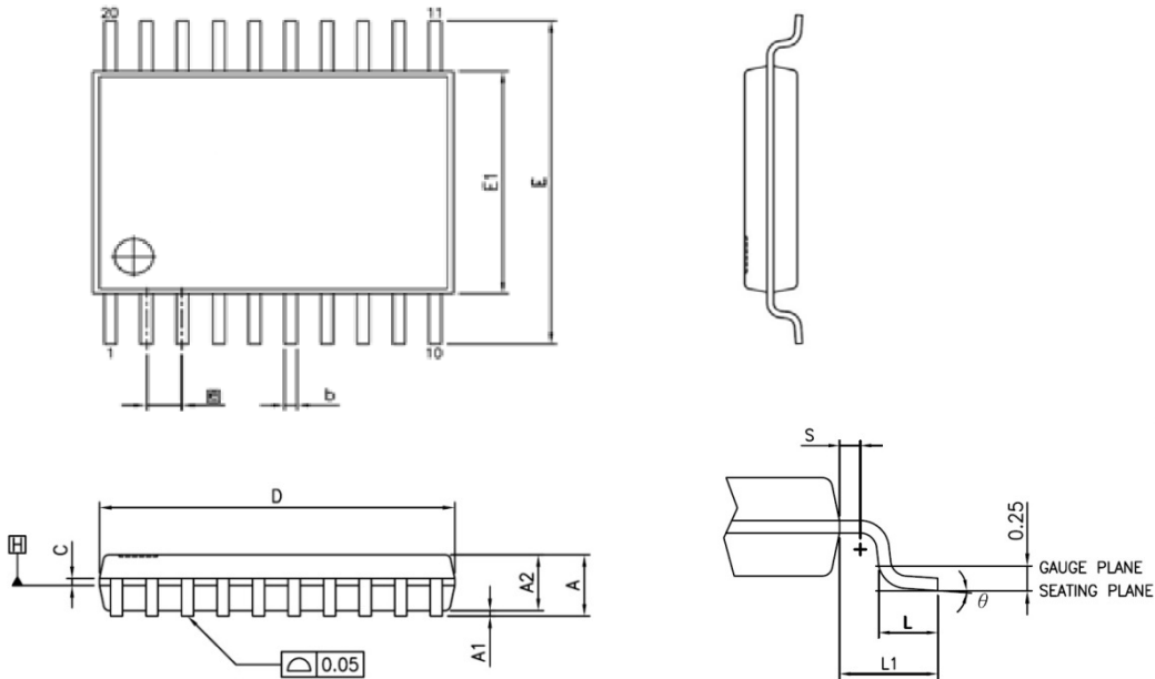
Figure 35-2. TSSOP-20 6.5 x 4.4mm, 0.65mm pitch Package Dimension
