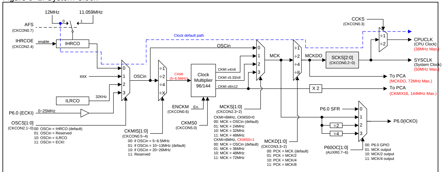
Figure 9–1. System Clock
