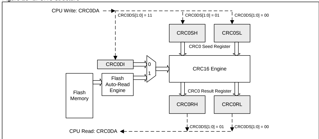
Figure 25–1. CRC structure
