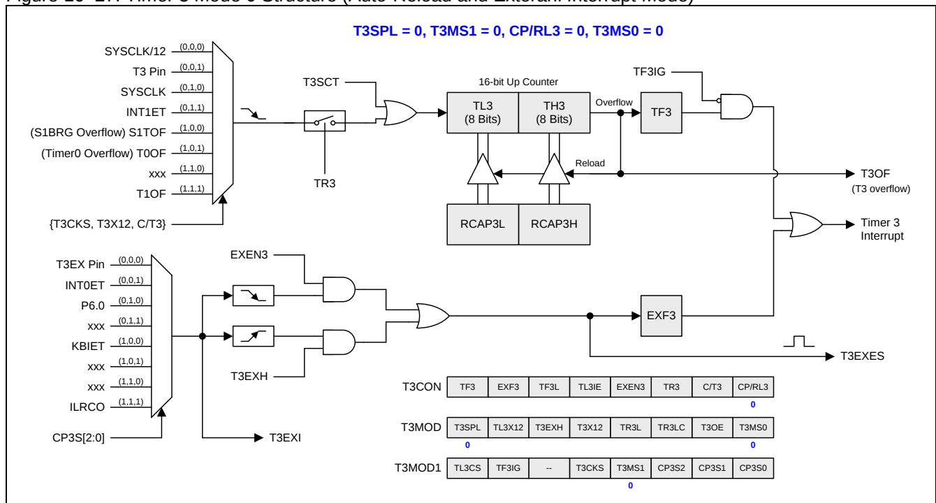
Figure 16–27. Timer 3 Mode 0 Structure (Auto-Reload and External Interrupt Mode)
