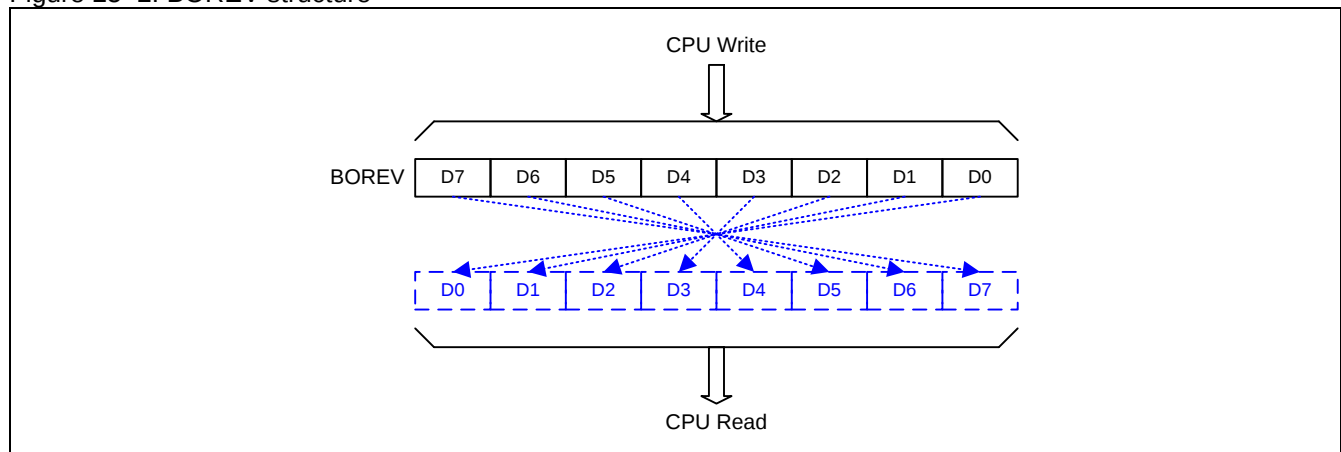
Figure 25–2. BOREV structure
