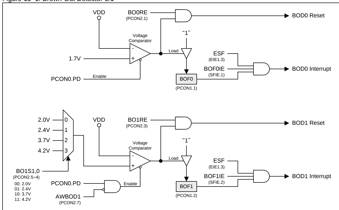
Figure 13–1. Brown-Out Detector 0/1
