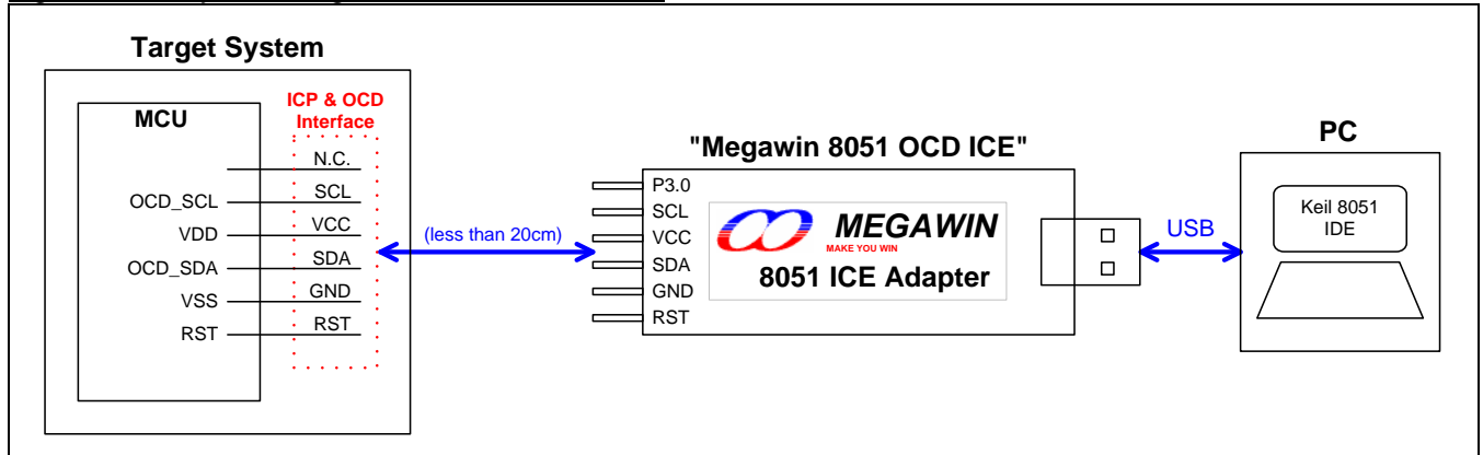
Figure 33–6. System Diagram for the ICE Function
