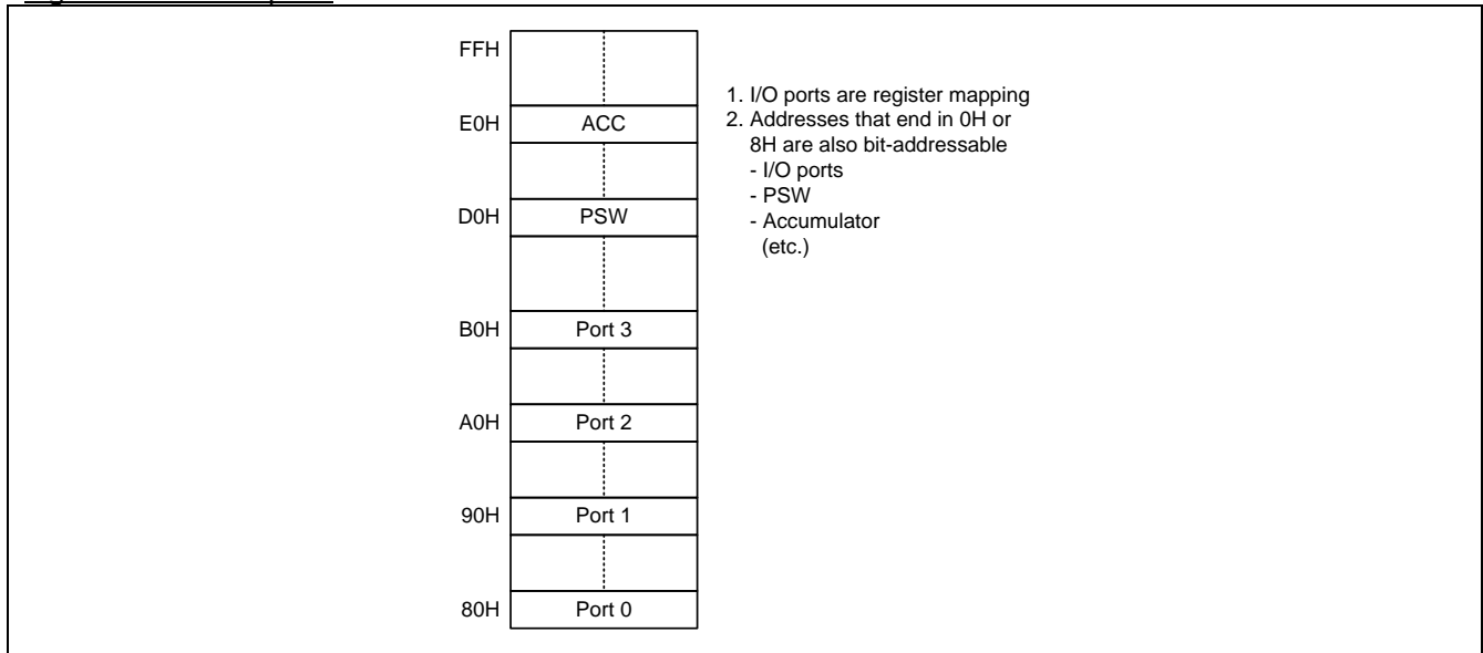
Figure 6–4. SFR Space
