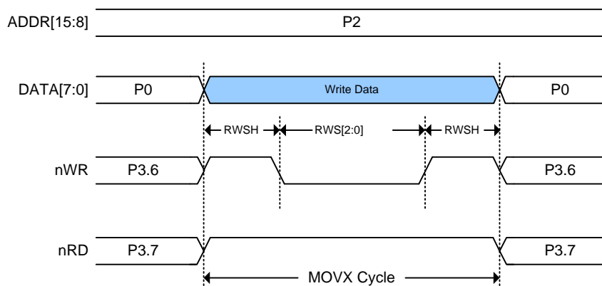
No Address Phase mode for 8-bit Data Write
