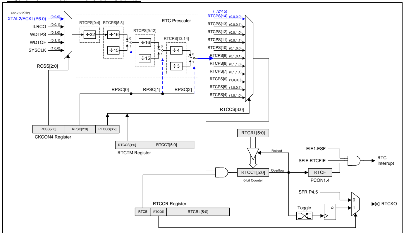
Figure 10–1. Real-Time-Clock Counter
