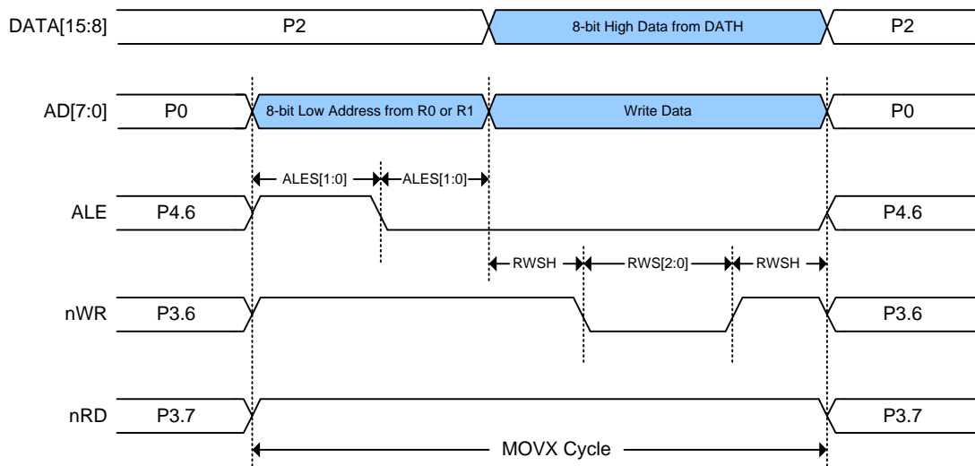
Muxed 8-bit Address mode for 16-bit Data Write
