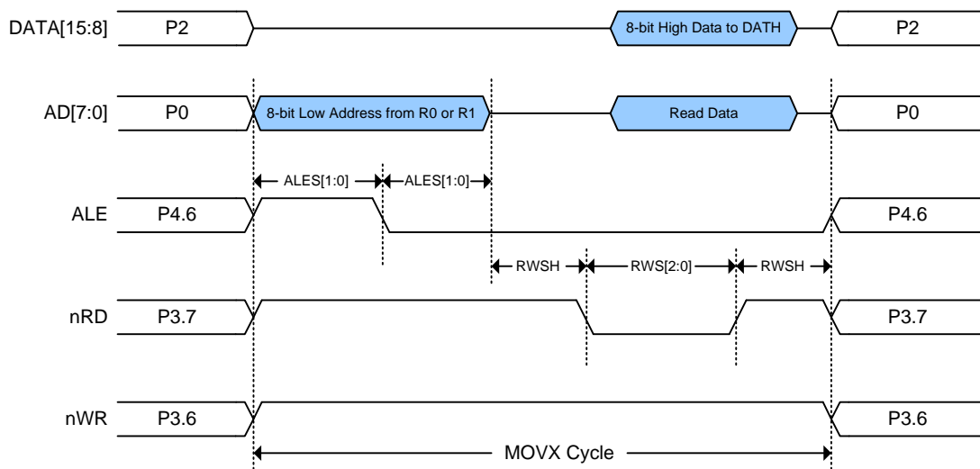
Muxed 8-bit Address mode for 16-bit Data Read
