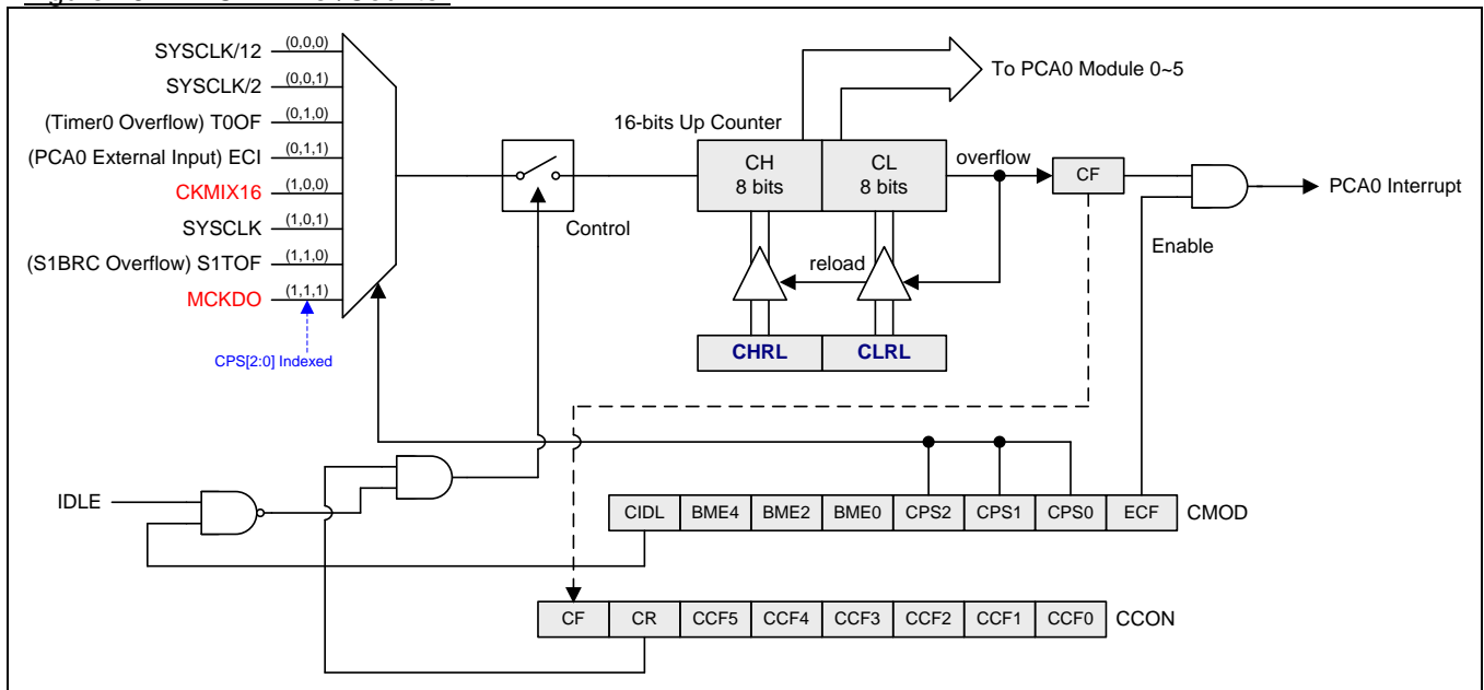
Figure 16–2. PCA Timer/Counter
