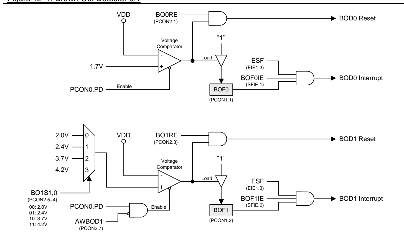
Figure 12–1. Brown-Out Detector 0/1
