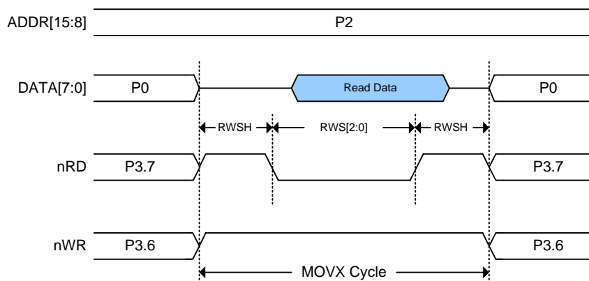
No Address Phase mode for 8-bit Data Read
