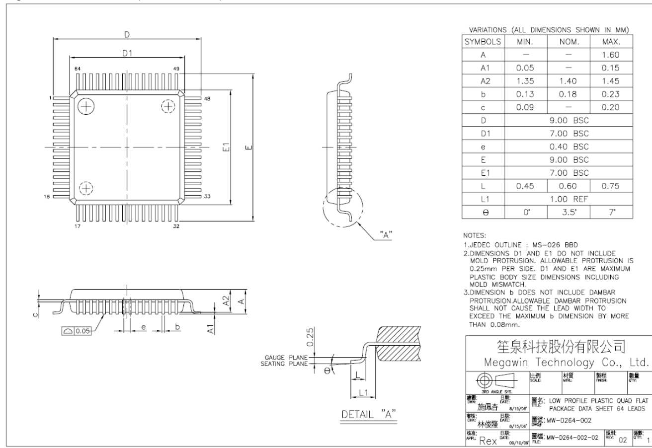
Figure 36–1 LQFP-64 (7mm X 7mm )
