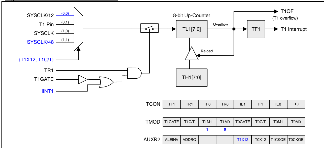
Figure 15–6. Timer 1 Mode 2 Structure
