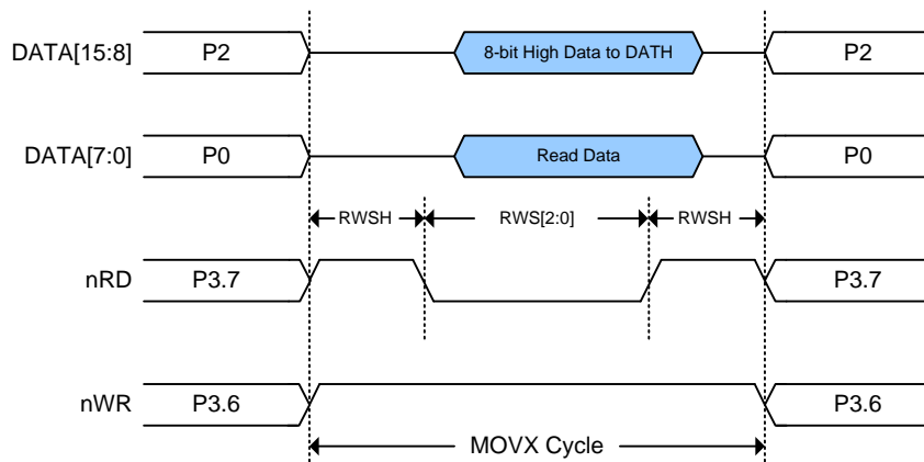
No Address Phase mode for 16-bit Data Read
