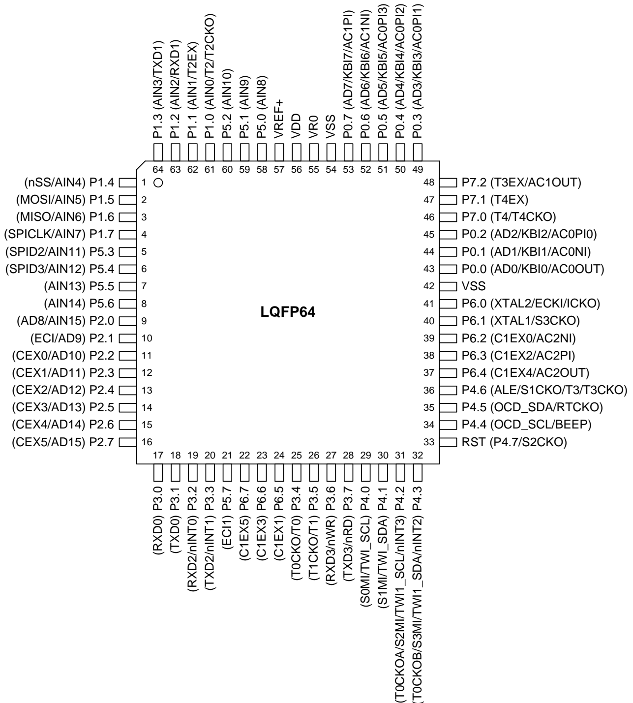
Figure 4–1. LQFP64 Top View
