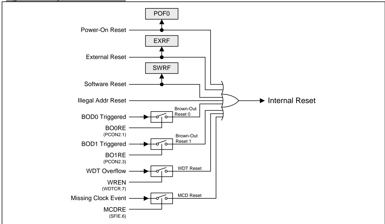
Figure 11–1. System Reset Source
