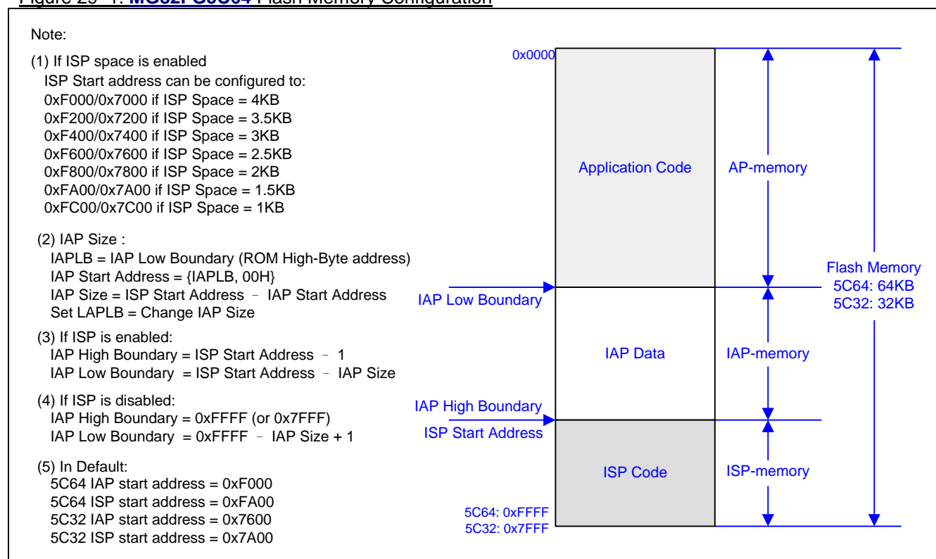
Figure 29–1. MG82FG5C64 Flash Memory Configuration
