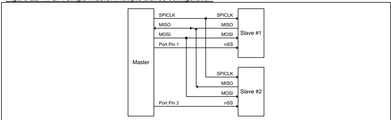
Figure 22–4. SPI single master multiple slaves configuration
