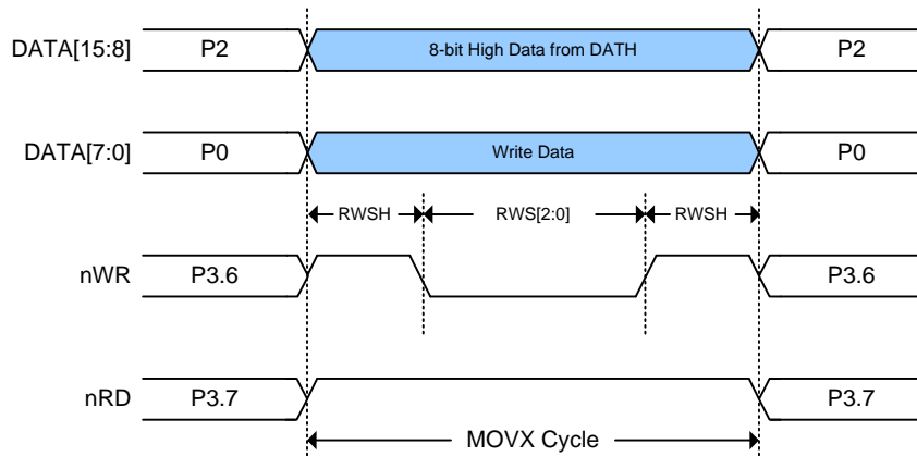
No Address Phase mode for 16-bit Data Write
