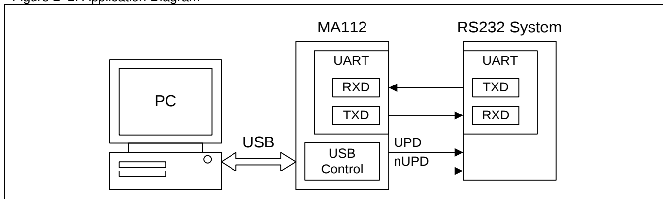
Figure 2–1. Application Diagram
