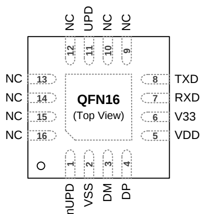
Figure 3–2. MA112 QFN16 (4x4) Top View
