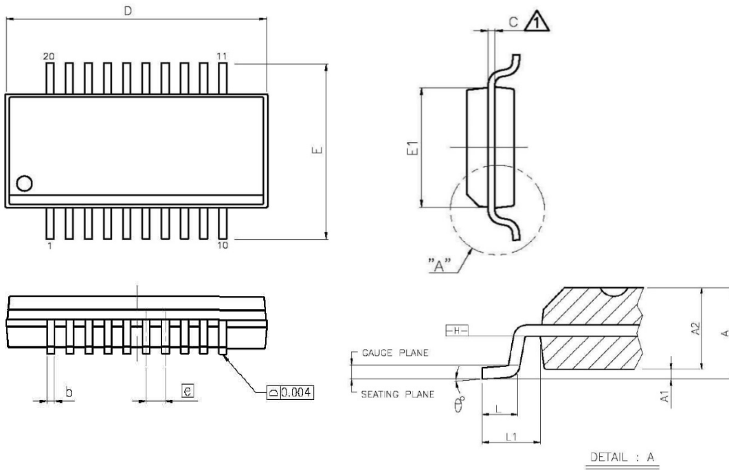
Figure 39-6. SSOP-20 (150 mil) Package Dimension
