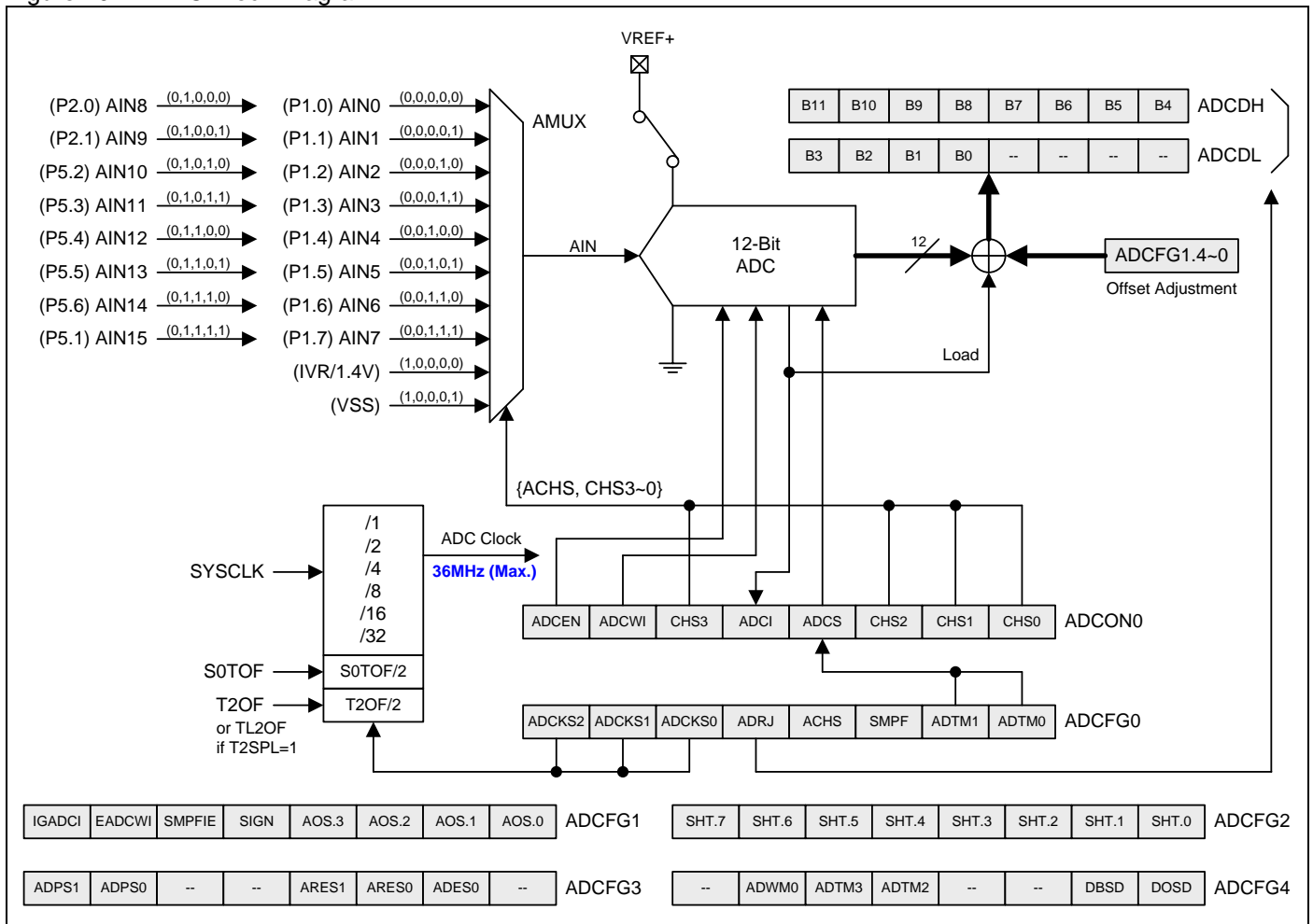
Figure 29–1. ADC Block Diagram
