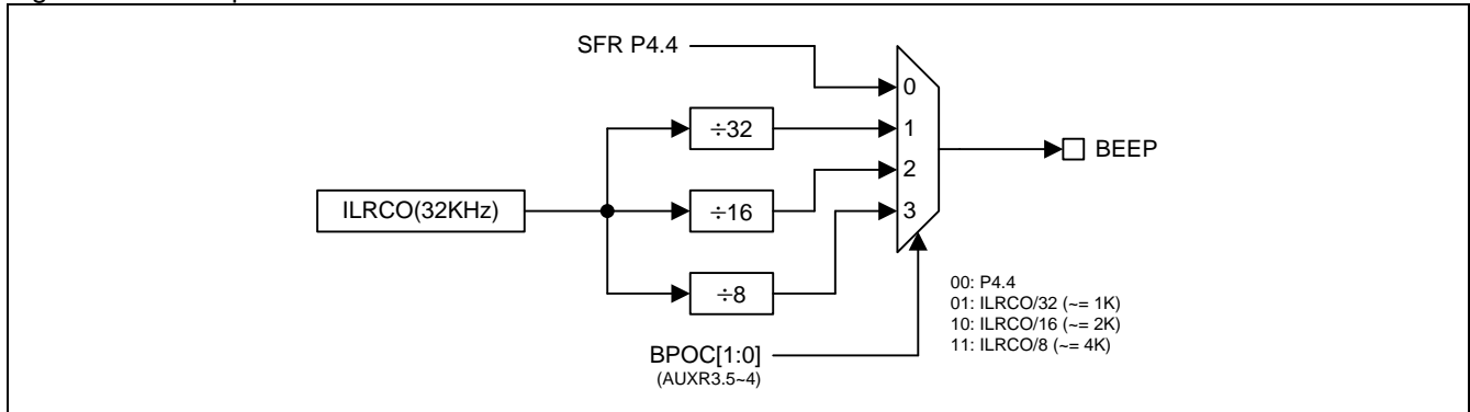
Figure 25–1. Beeper Generator
