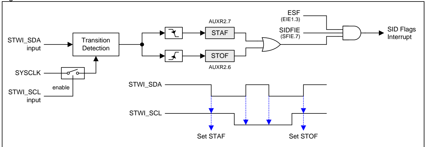
Figure 24–1. Serial Interface Detection structure
