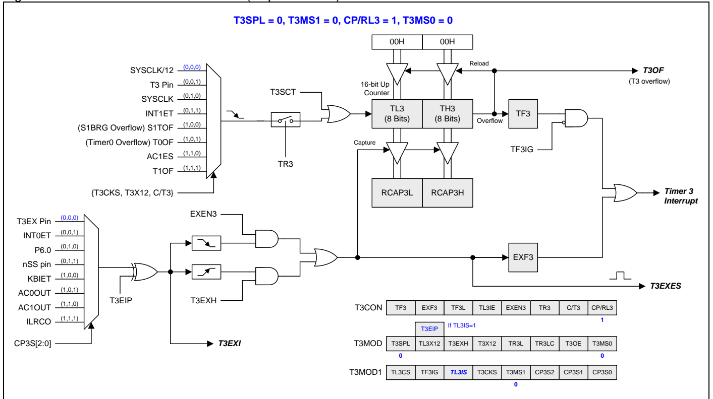
Figure 16–31. Timer 3 Mode 2 Structure (Capture Mode)
