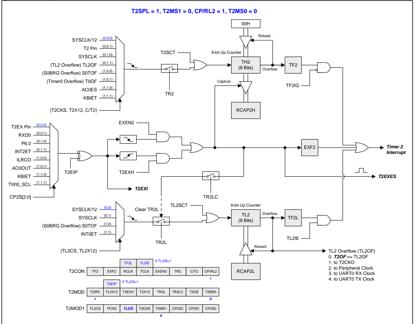
Figure 16–20. Split Timer 2 Mode 2 Structure (Capture)
