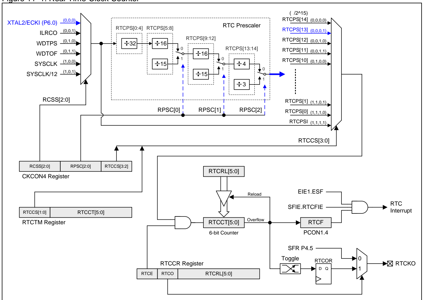
Figure 11-1. Real-Time-Clock Counter
