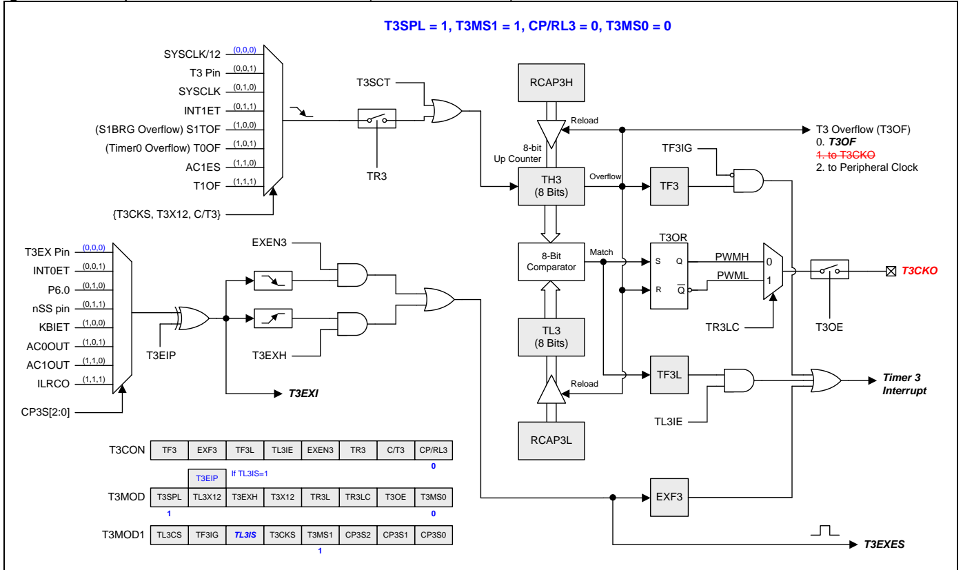
Figure 16–38. Split Timer 3 Mode 4 Structure (8-bit PWM mode)
