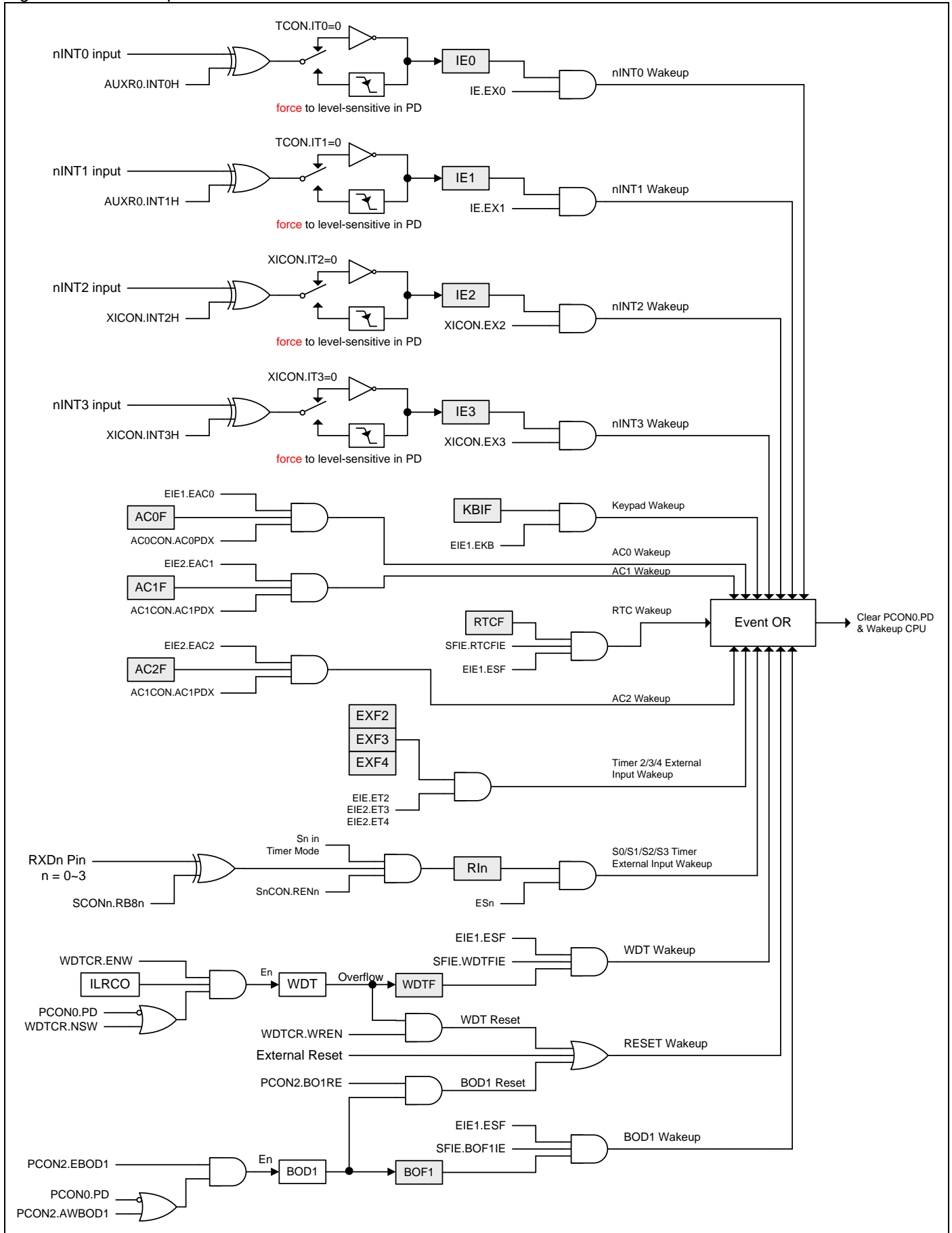
Figure 13–2. Wakeup structure of Power Down mode
