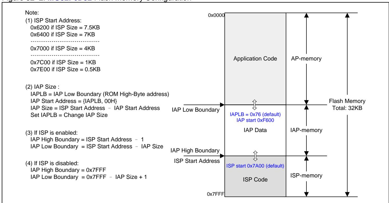
Figure 32–2. MG82F6D32 Flash Memory Configuration
