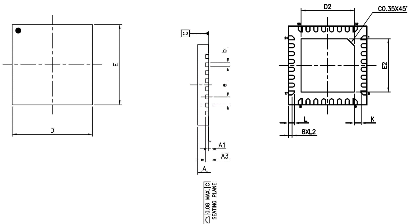
Figure 39-5. QFN-32 (4mm X 4mm X 0.55mm) Package Dimension
