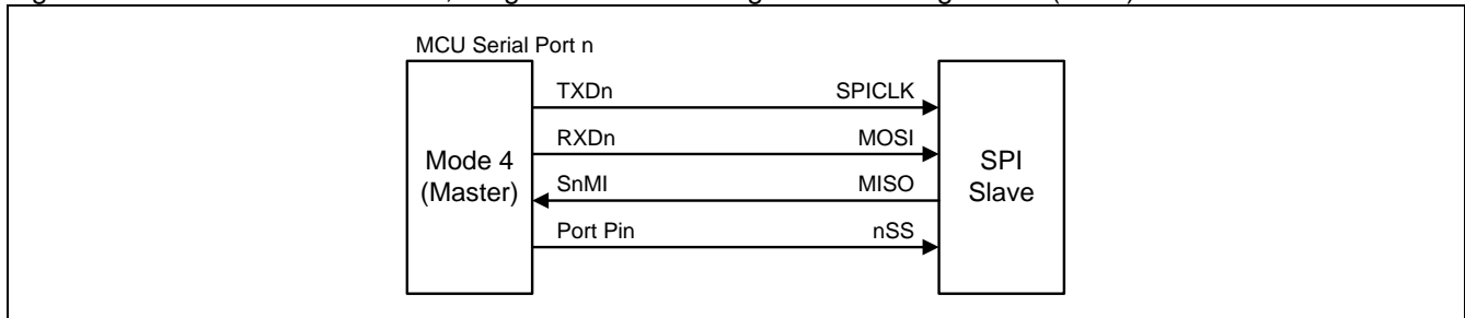
Figure 19–2. Serial Port 1 Mode 4, Single Master and Single Slave configuration (n = 1)
