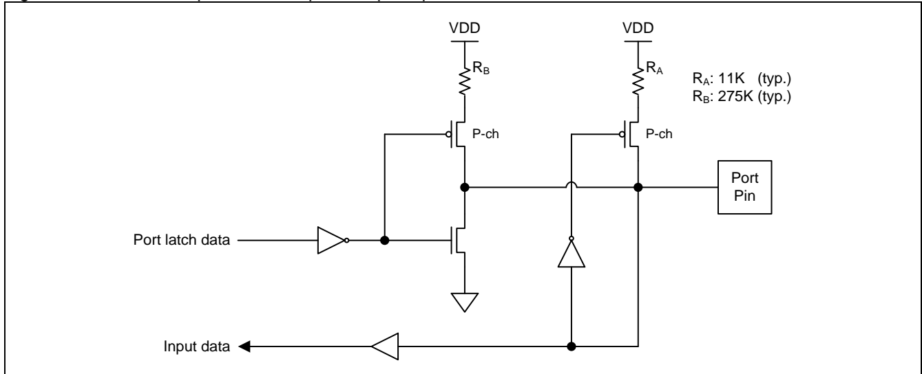
Figure 14–6. General Open-Drain output with pull-up resistor
