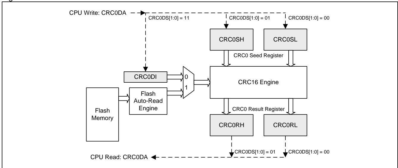
Figure 27–1. CRC structure
