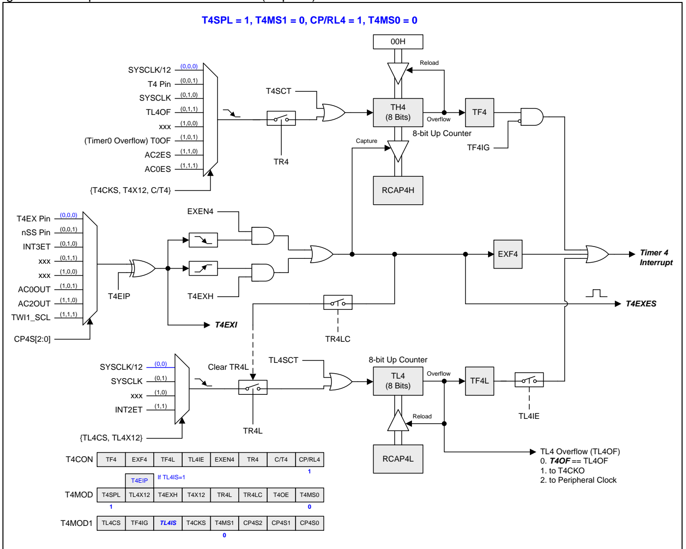
Figure 16–50. Split Timer 4 Mode 2 Structure (Capture)
