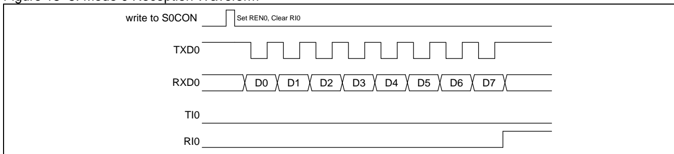
Figure 18-5. Mode 0 Reception Waveform
