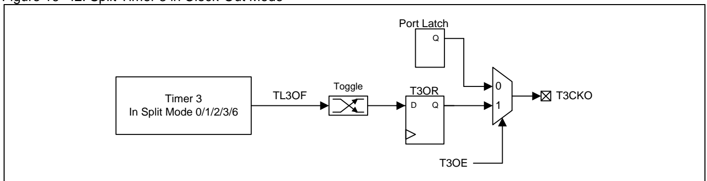
Figure 16–42. Split Timer 3 in Clock-Out Mode
