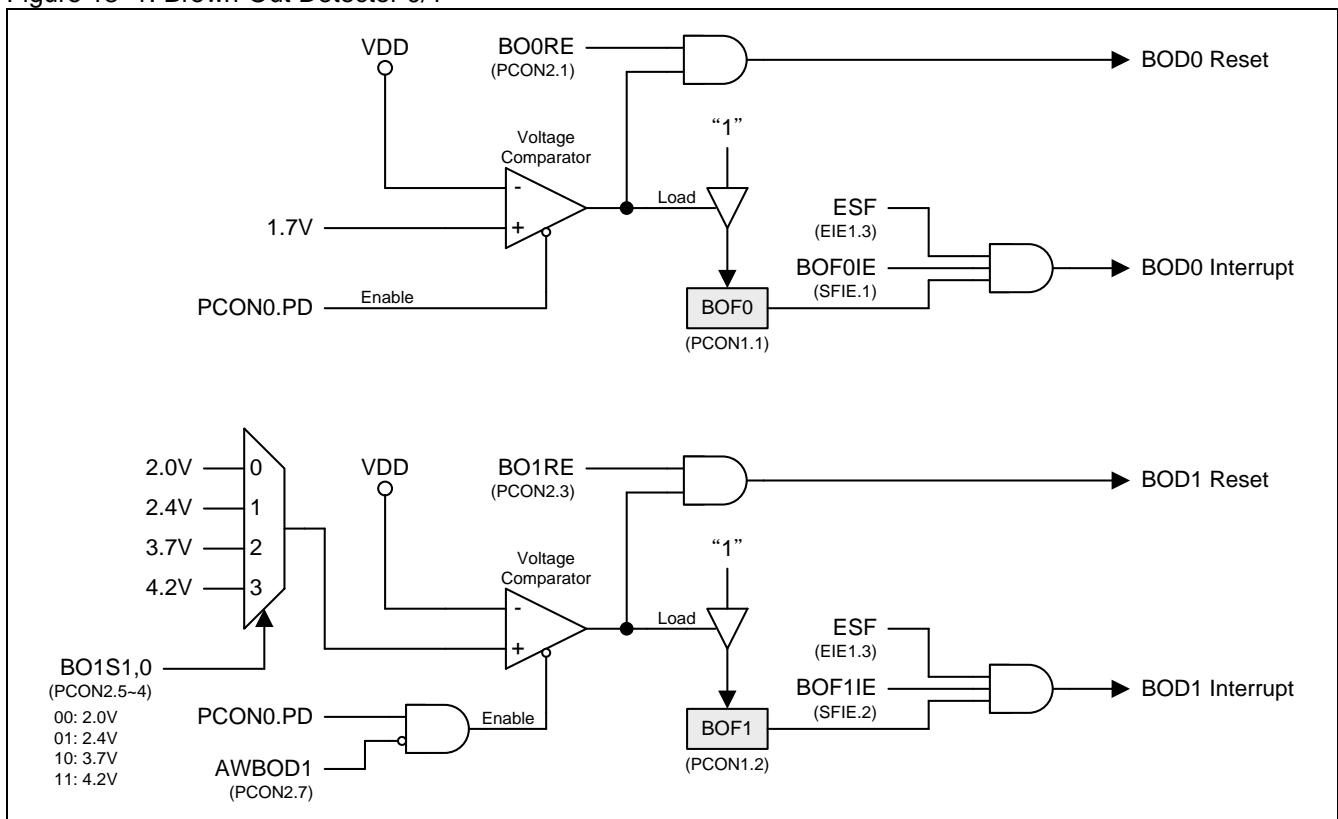
Figure 13–1. Brown-Out Detector 0/1
