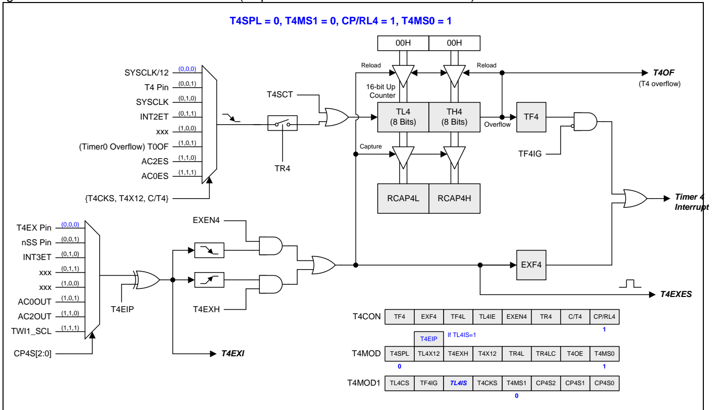
Figure 16–46. Timer 4 Mode 3 Structure (Capture with Auto-Zero on TL4 & TH4)
