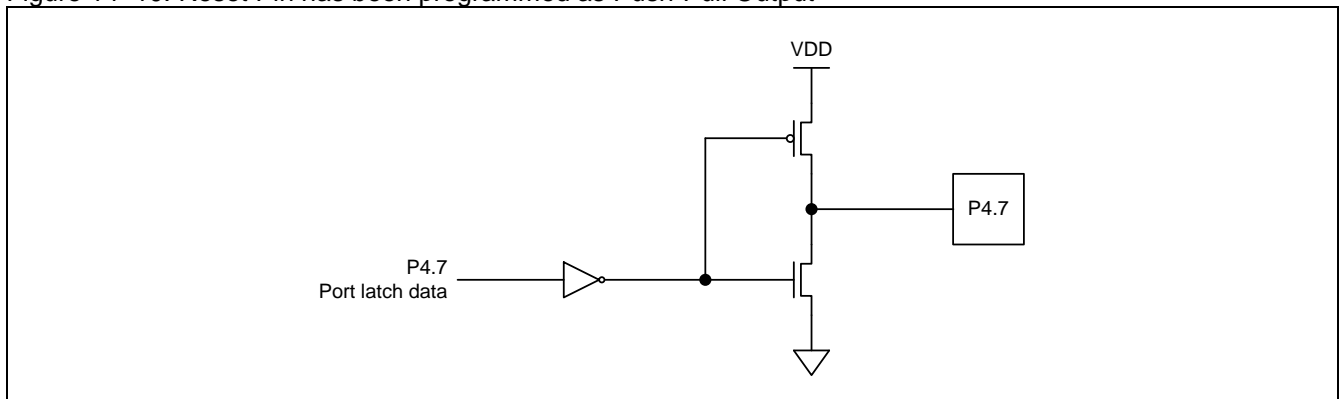
Figure 14–10. Reset Pin has been programmed as Push-Pull Output
