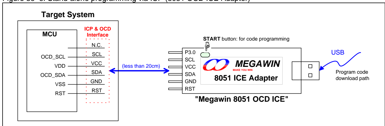
Figure 36-6. Stand-alone programming via ICP (8051 OCD ICE Adapter)
