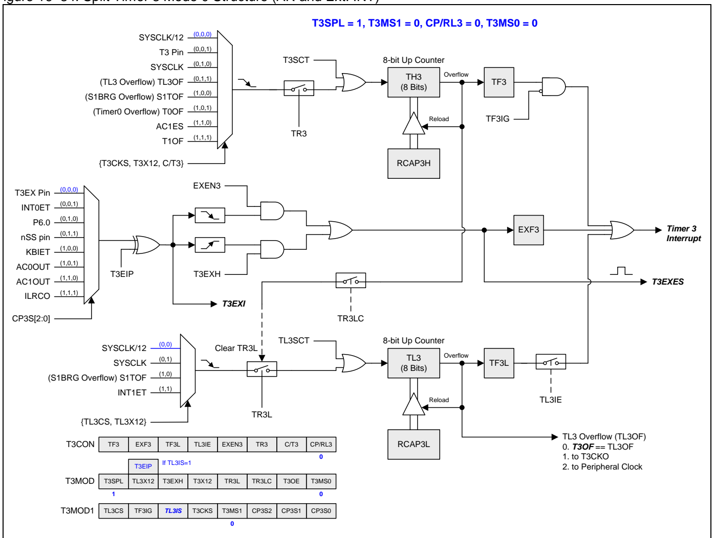
Figure 16–34. Split Timer 3 Mode 0 Structure (AR and Ext. INT)
