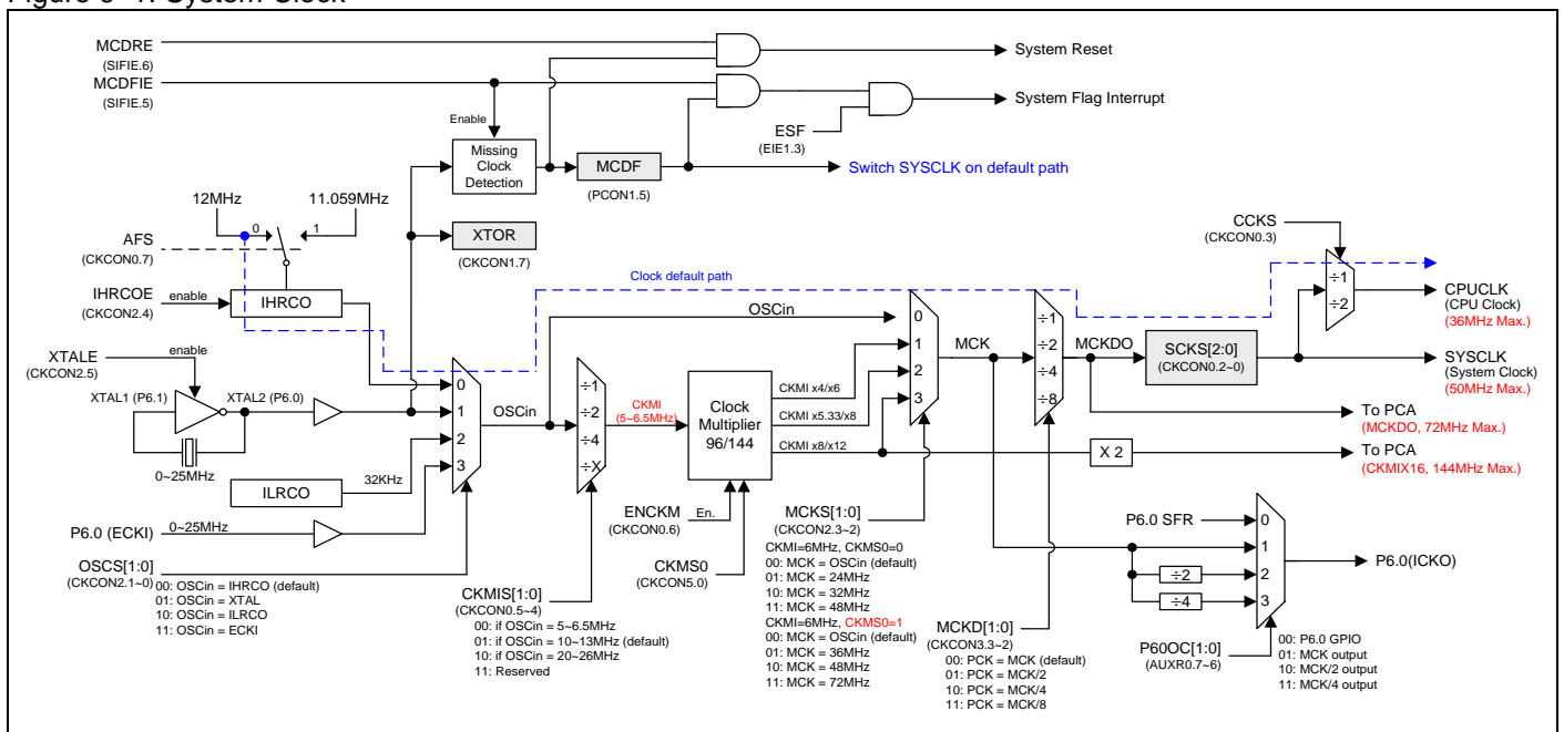
Figure 9–1. System Clock
