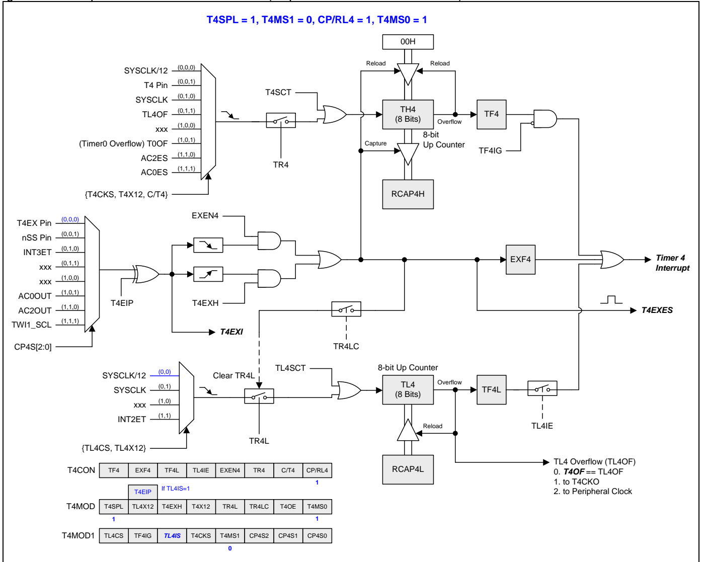
Figure 16–51. Split Timer 4 Mode 3 Structure (Capture with Auto-Zero on TH4)
