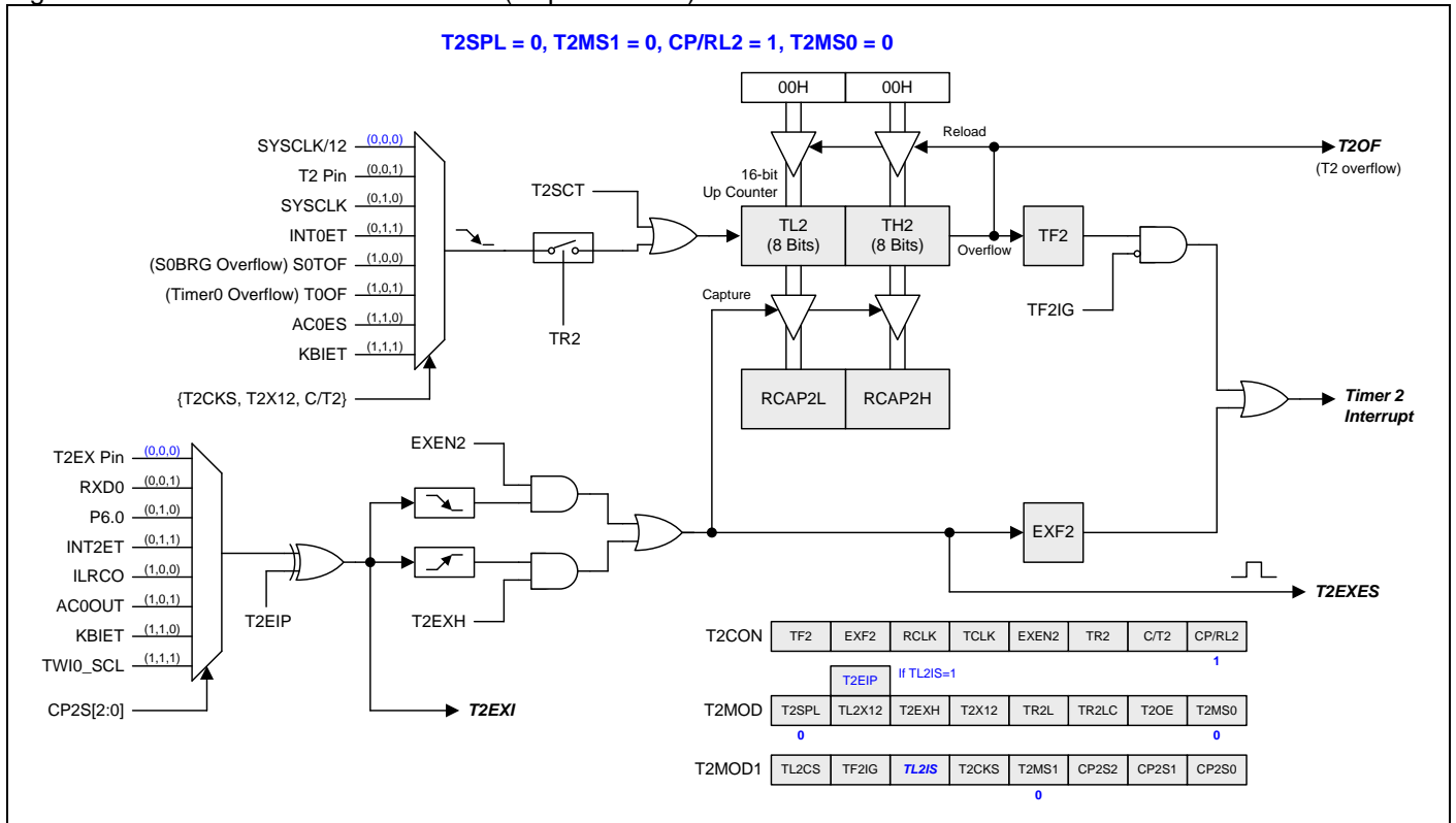
Figure 16–15. Timer 2 Mode 2 Structure (Capture Mode)
