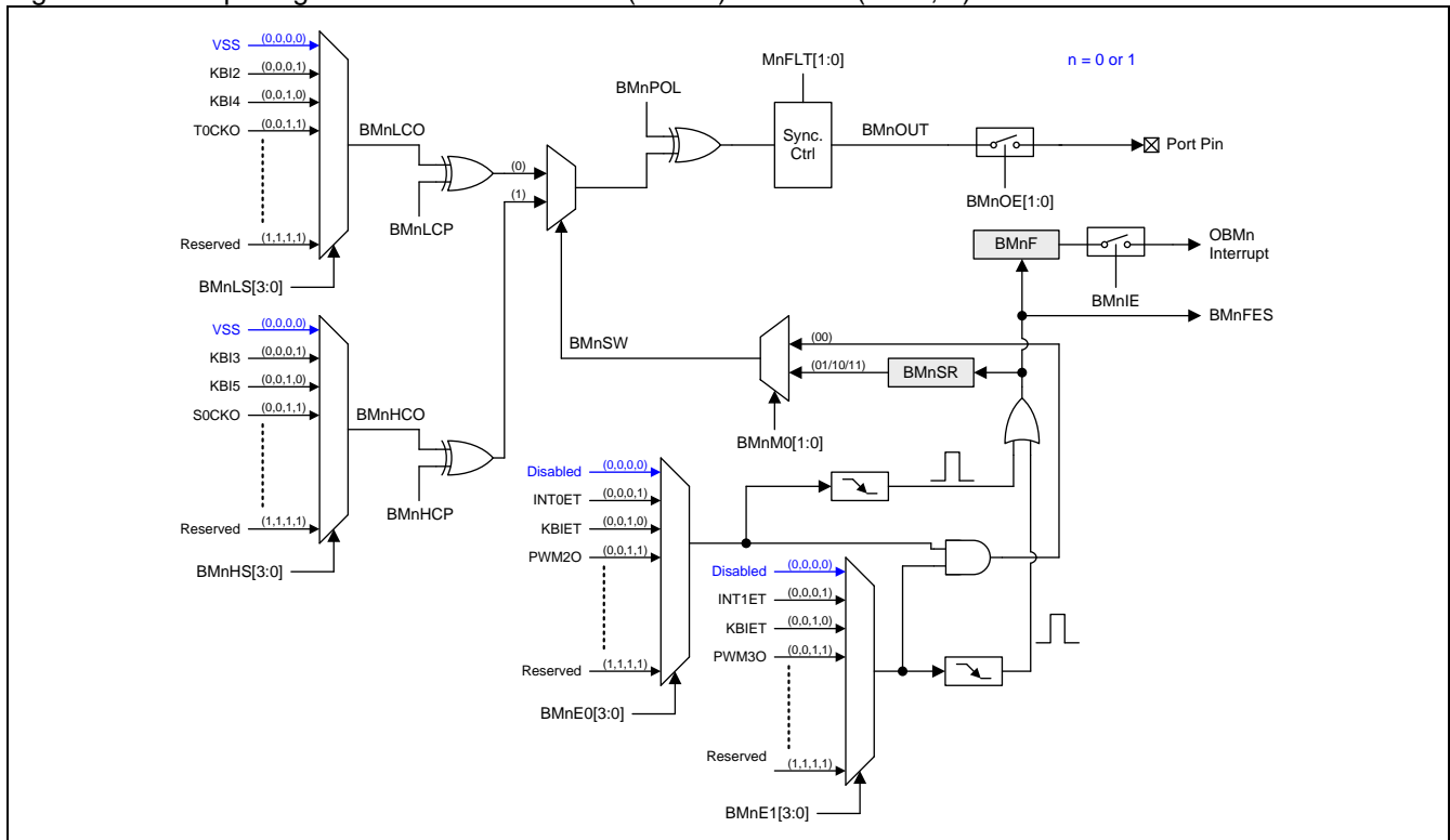
Figure 28–2. Output signal Break & Modulator n (OBMn) structure (n = 0, 1)
