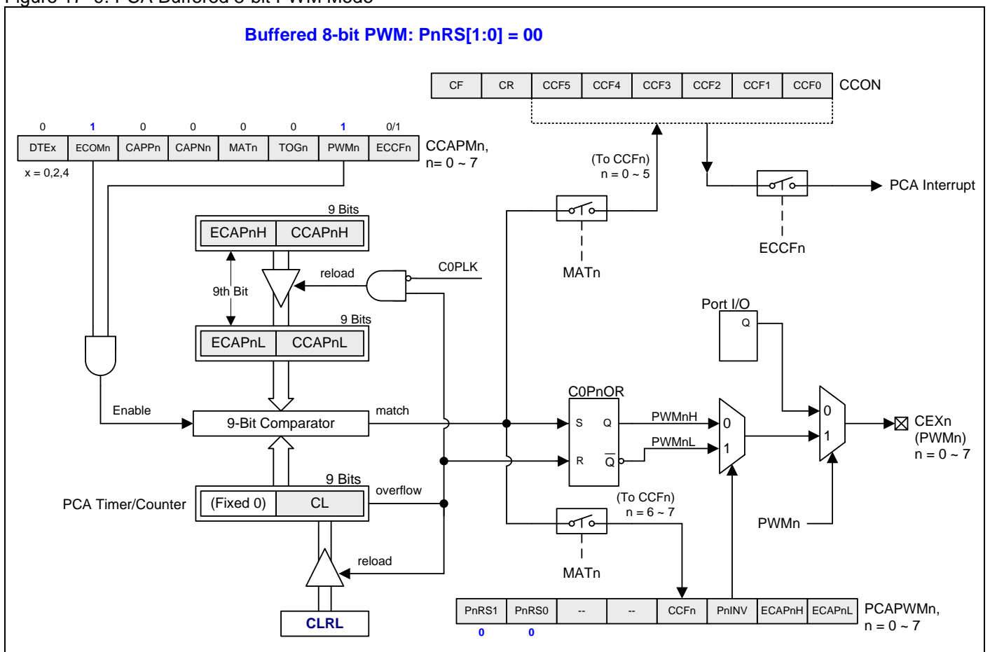
Figure 17–9. PCA Buffered 8-bit PWM Mode
