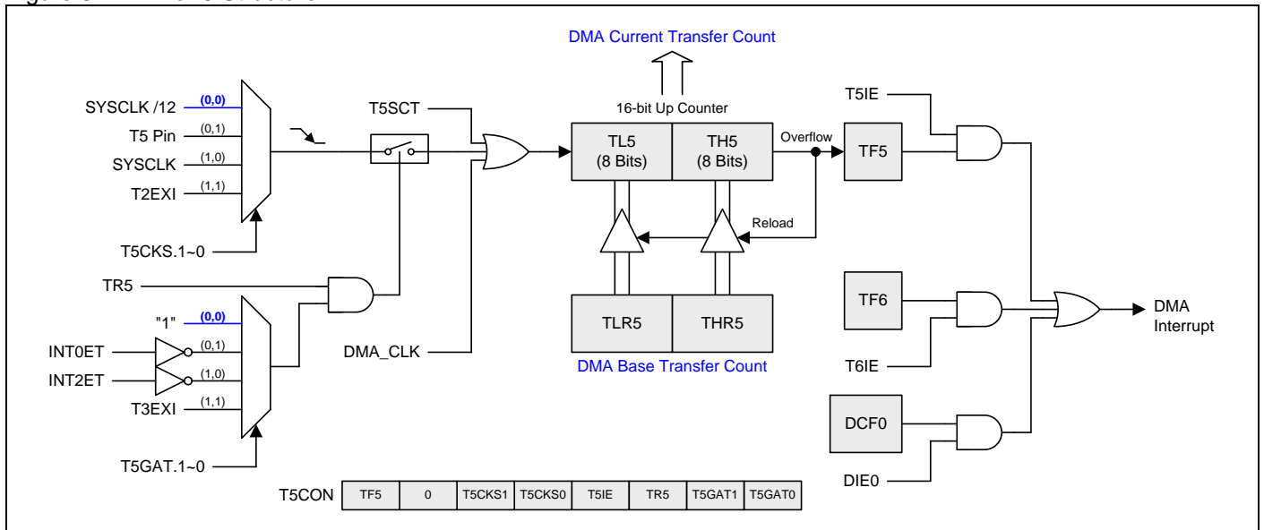
Figure 8-4. Timer 5 Structure
