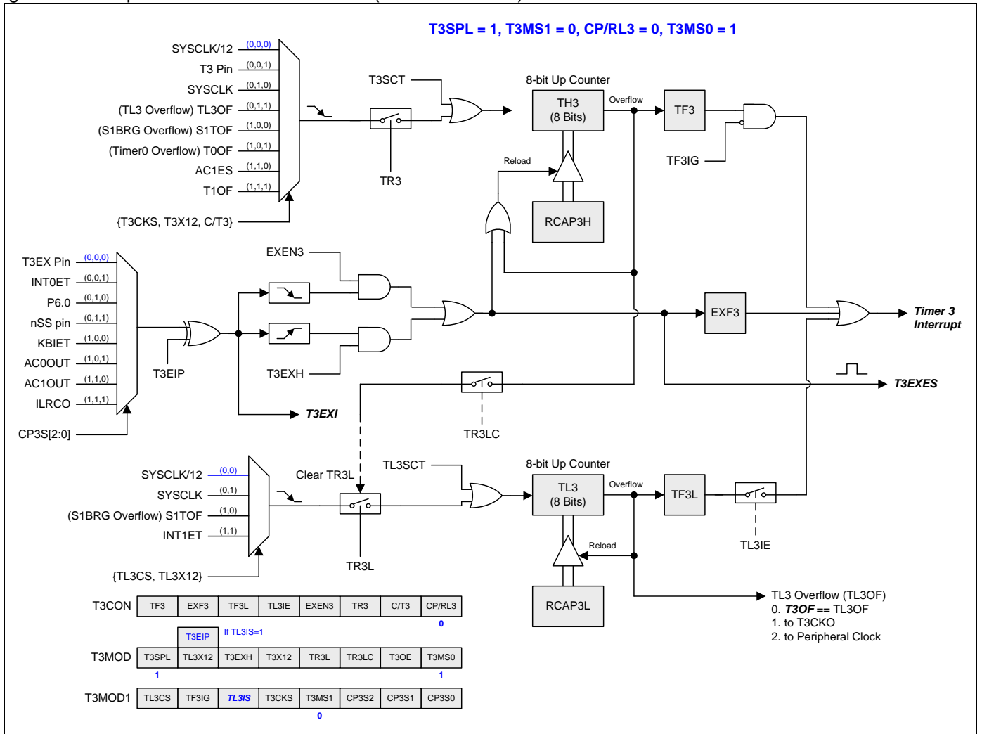
Figure 16–35. Split Timer 3 Mode 1 Structure (AR with Ext. INT)
