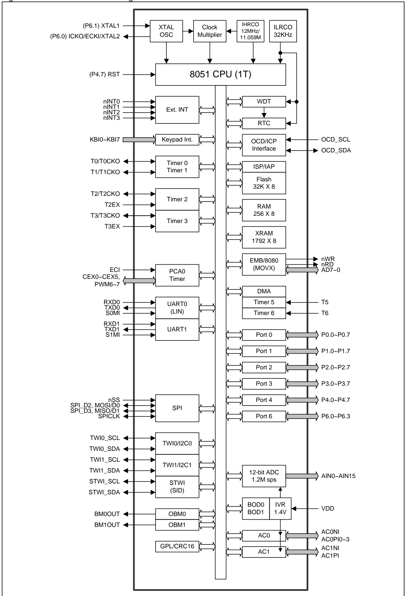
Figure 2–2. MG82G6D32 Block Diagram
