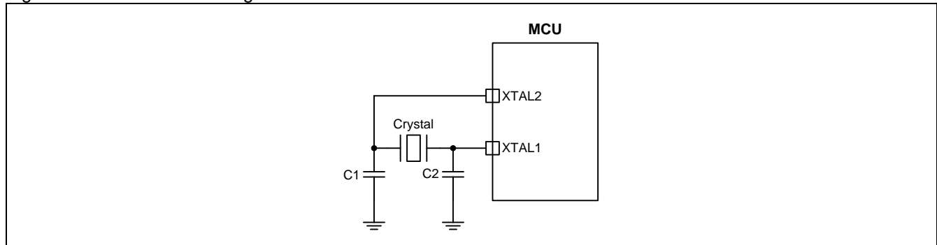
Figure 36–3. XTAL Oscillating Circuit
