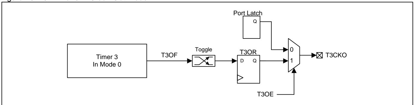
Figure 16–40. Timer 3 in Clock-Out Mode
