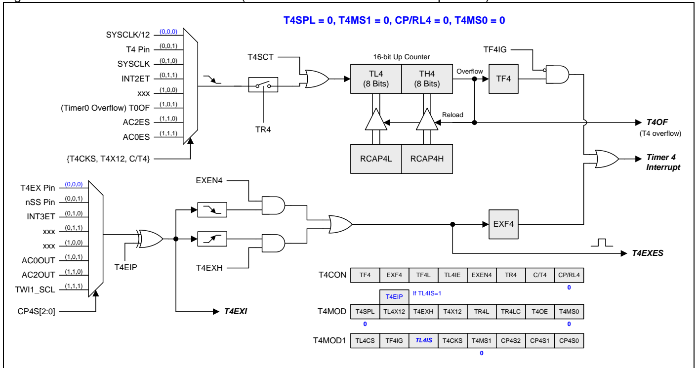
Figure 16–43. Timer 4 Mode 0 Structure (Auto-Reload and External Interrupt Mode)
