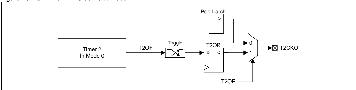
Figure 16–26. Timer 2 in Clock-Out Mode
