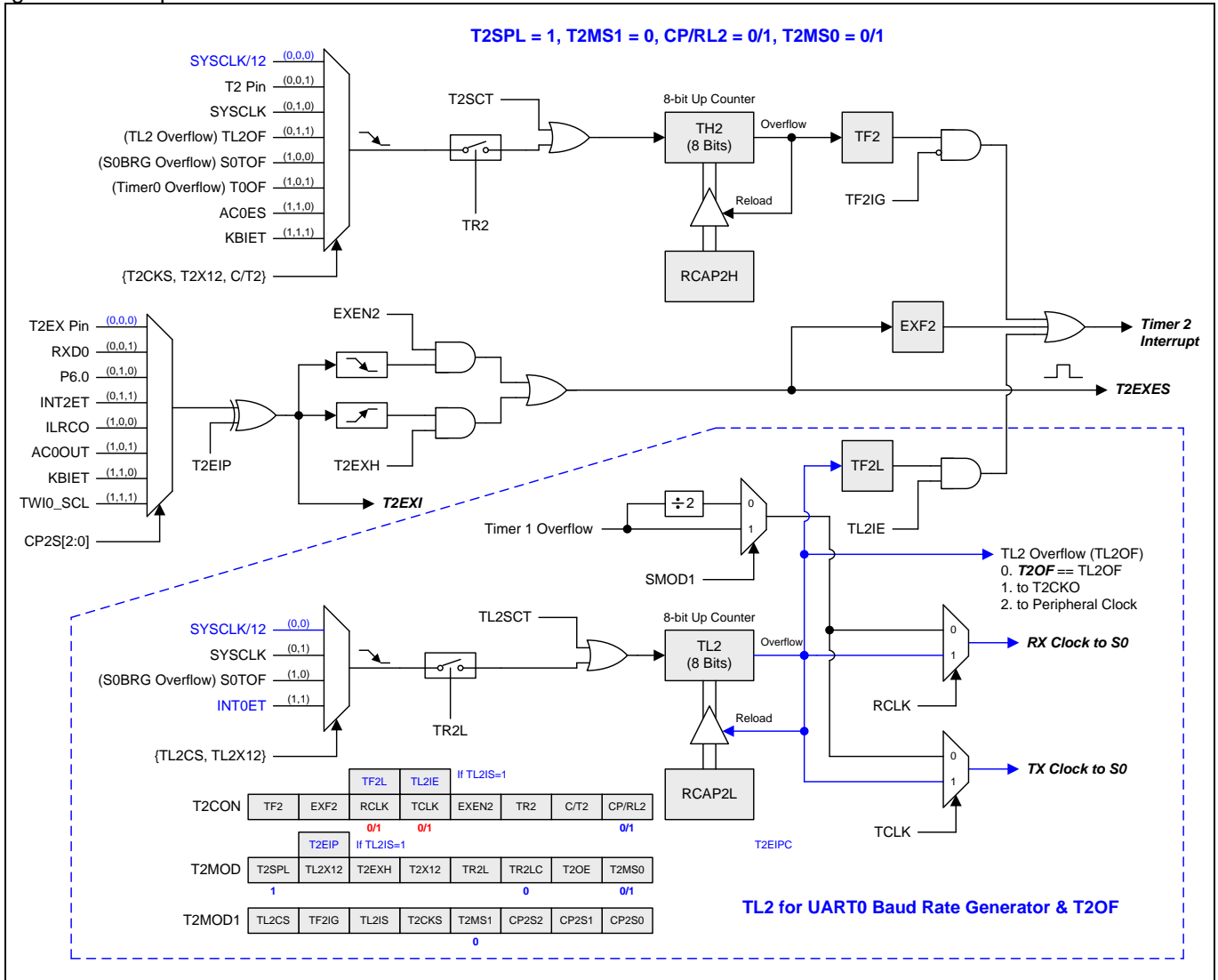
Figure 16–24. Split Timer 2 in Baud-Rate Generator Mode
