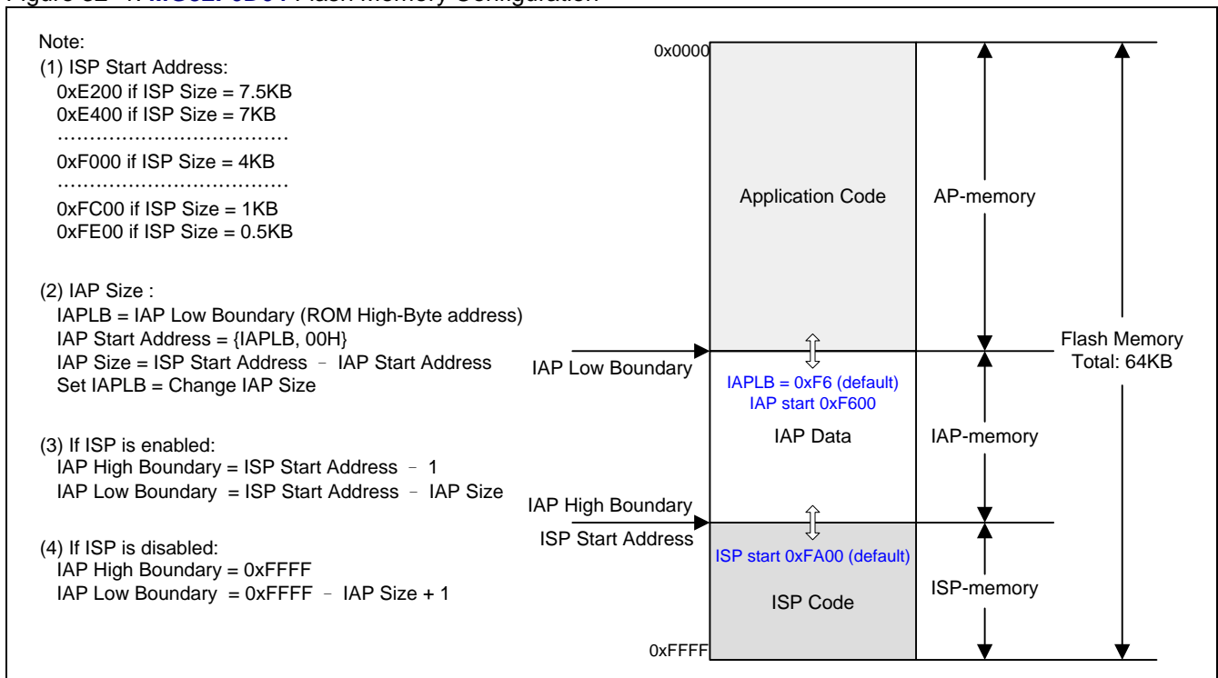
Figure 32–1. MG82F6D64 Flash Memory Configuration
