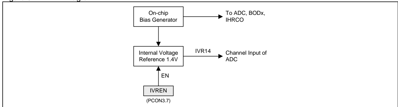
Figure 31–1. IVR Diagram
