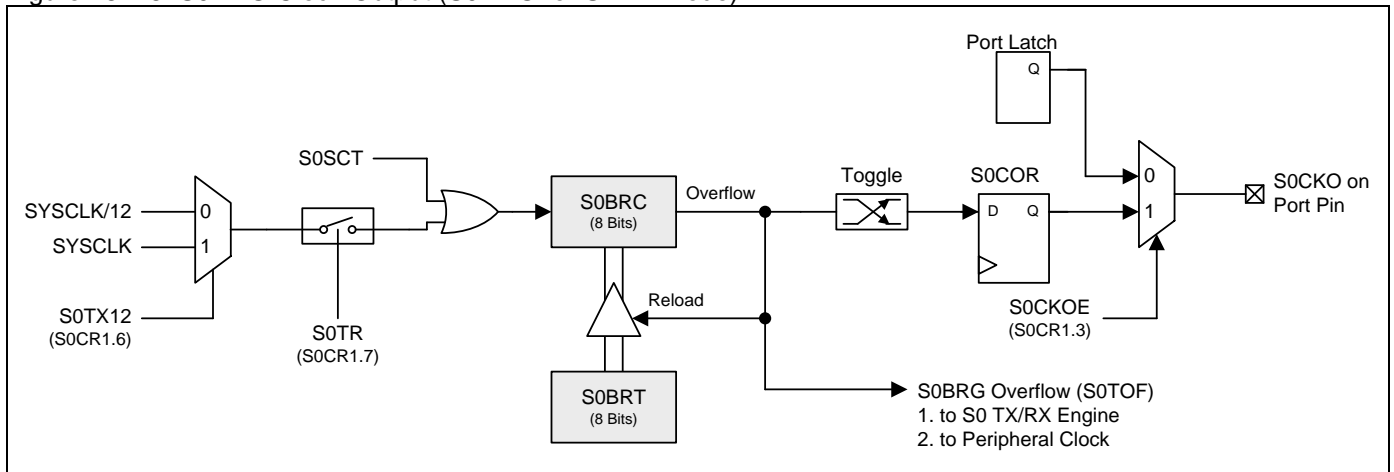
Figure 18–18. S0BRG Clock Output (S0BRG for UART Mode)
