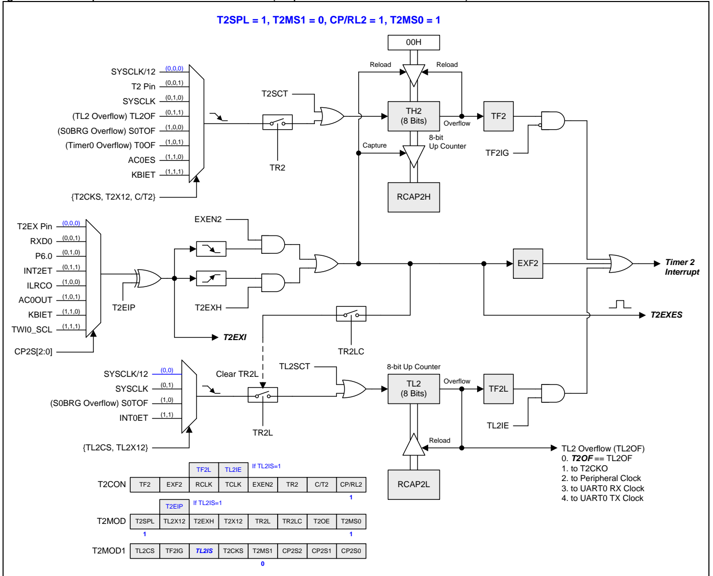
Figure 16–21. Split Timer 2 Mode 3 Structure (Capture with Auto-Zero on TH2)
