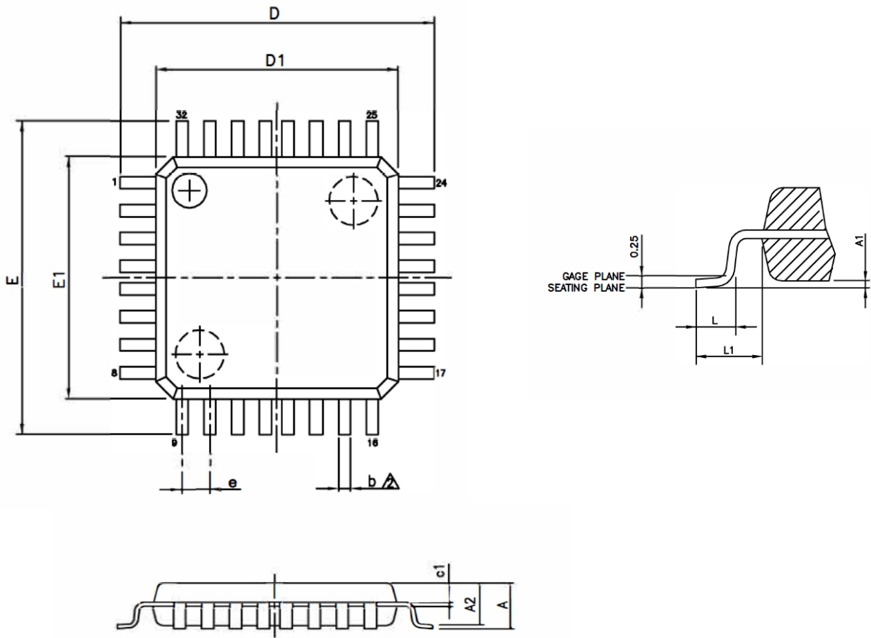
Figure 39-4. LQFP-32 (7mm X 7mm ) Package Dimension
