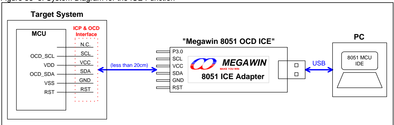
Figure 36–8. System Diagram for the ICE Function
