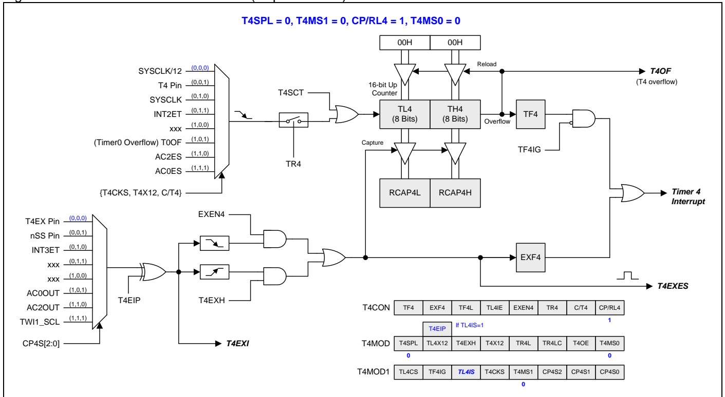
Figure 16–45. Timer 4 Mode 2 Structure (Capture Mode)
