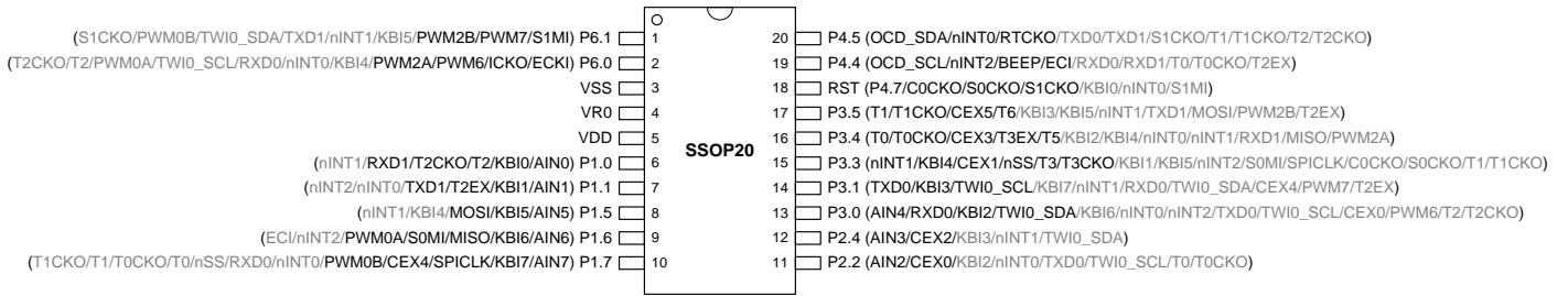
Figure 4–7. MG82F6D64AL20 SSOP20 Top View
