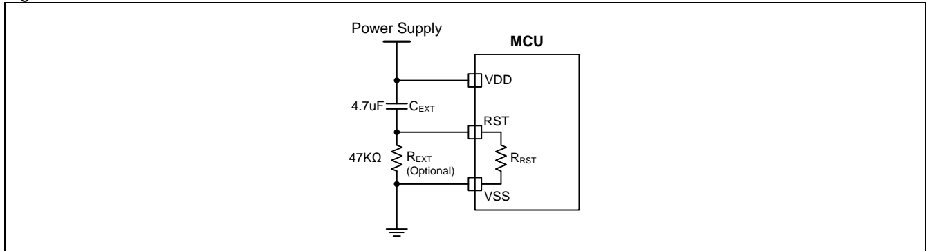
Figure 36–2. Reset Circuit
