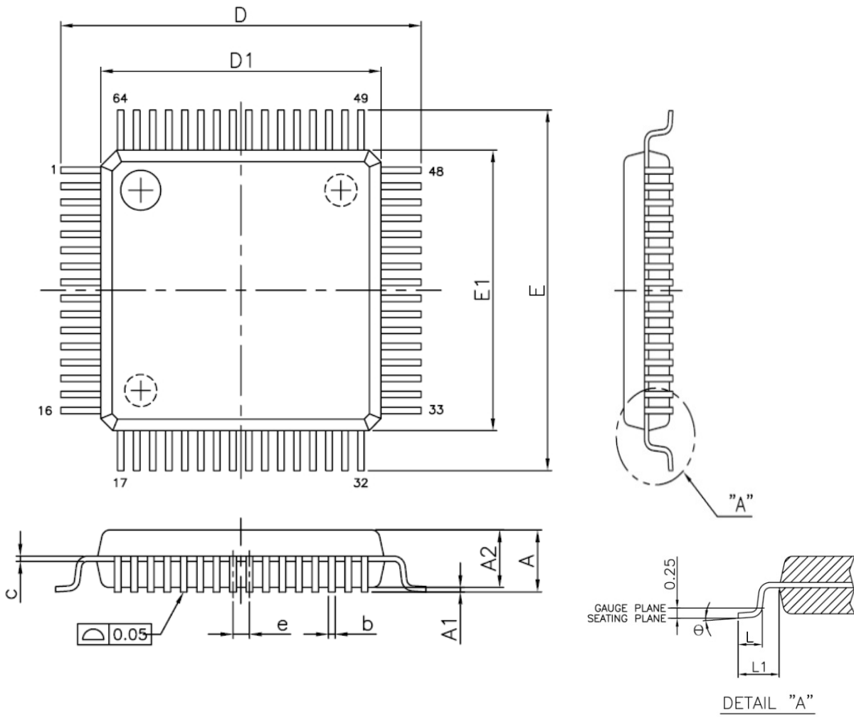
Figure 39-1. LQFP-64 (7mm X 7mm ) Package Dimension
