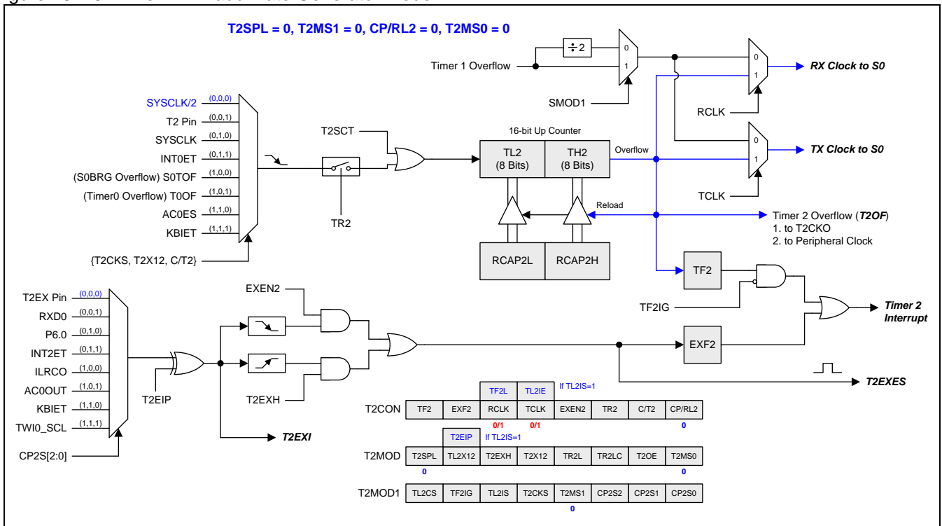
Figure 16–23. Timer 2 in Baud-Rate Generator Mode
