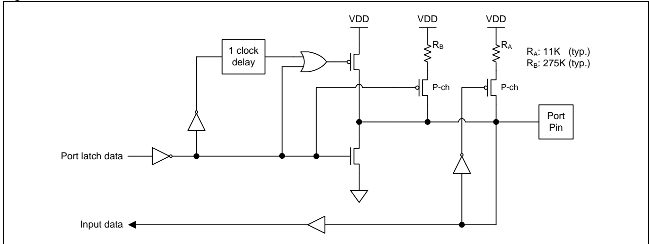
Figure 14–1. Port 3 Quasi-Bidirectional I/O
