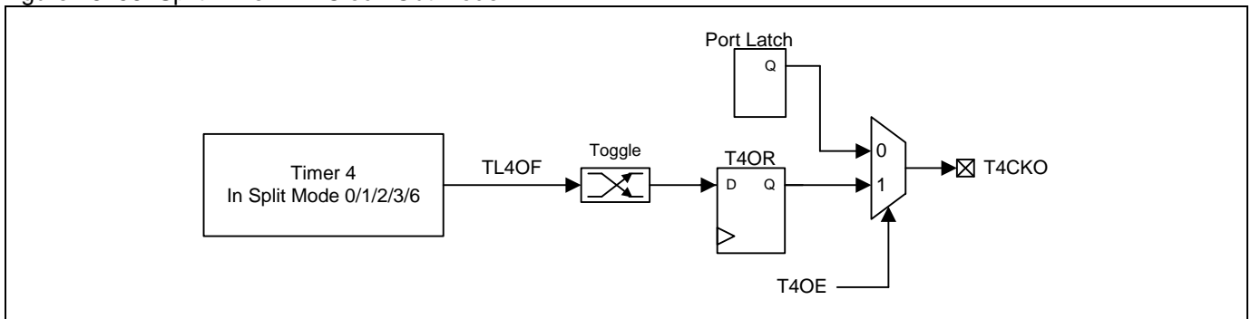
Figure 16–56. Split Timer 4 in Clock-Out Mode
