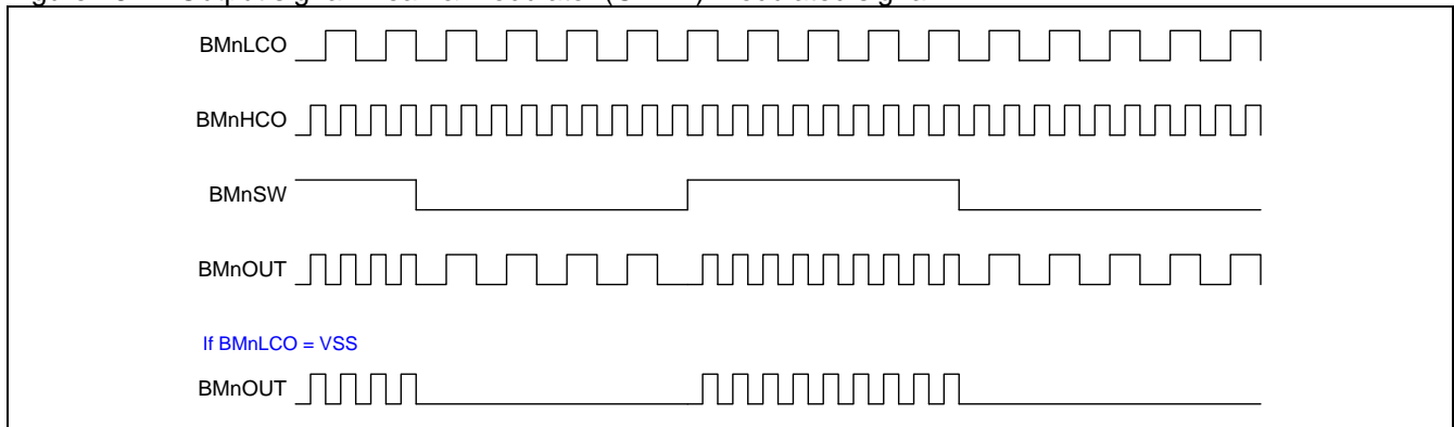
Figure 28–1. Output signal Break & Modulator (OBMn) modulated signal
