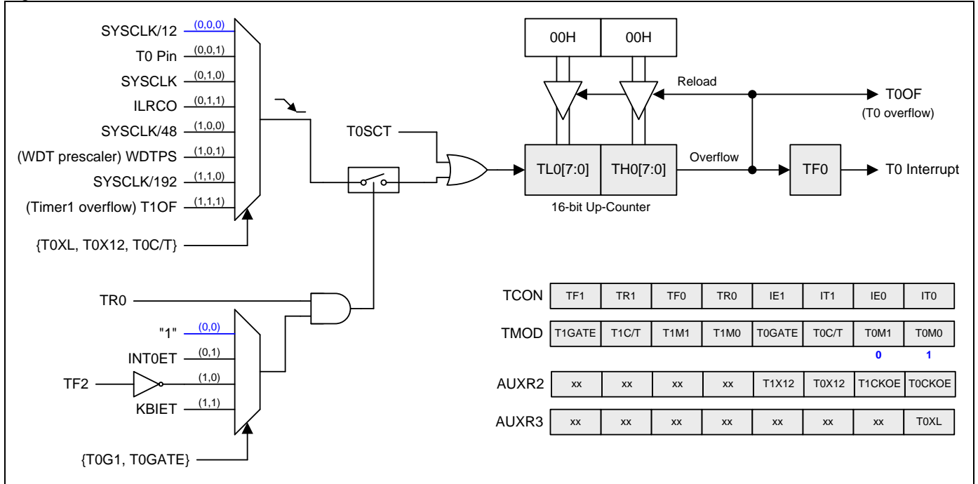
Figure 16–3. Timer 0 Mode 1 Structure
