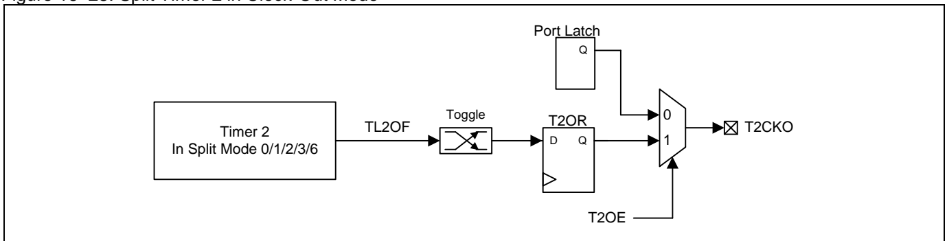
Figure 16–28. Split Timer 2 in Clock-Out Mode
