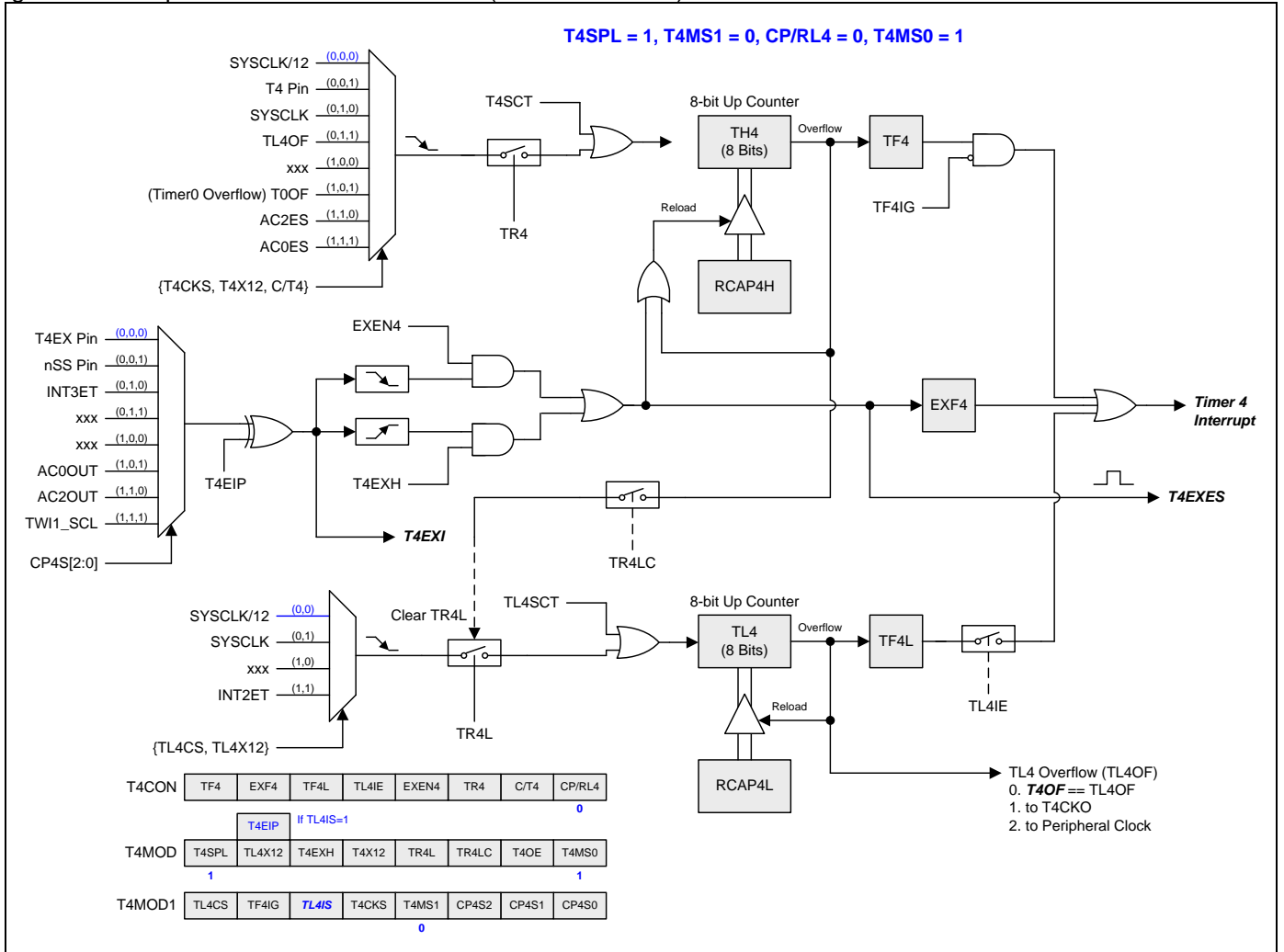
Figure 16–49. Split Timer 4 Mode 1 Structure (AR with Ext. INT)
