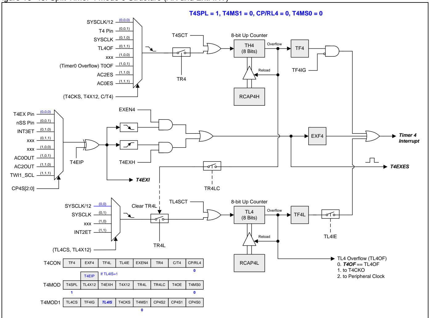
Figure 16–48. Split Timer 4 Mode 0 Structure (AR and Ext. INT)
