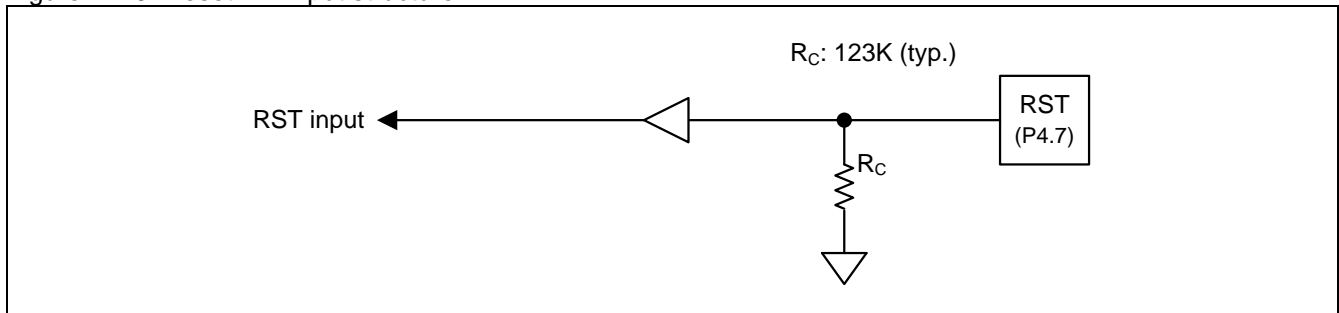
Figure 14–9. Reset Pin input structure
