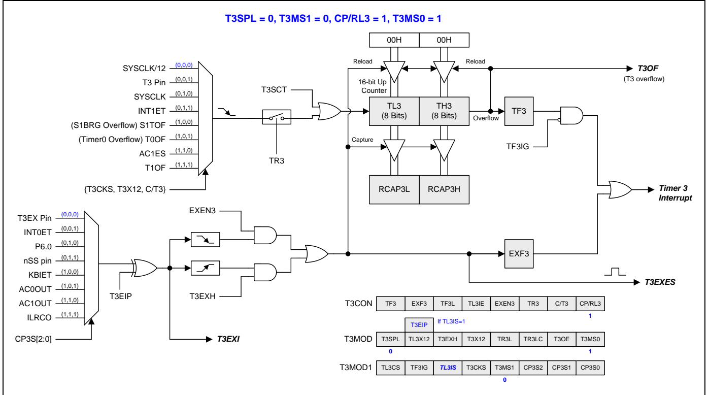
Figure 16–32. Timer 3 Mode 3 Structure (Capture with Auto-Zero on TL3 & TH3)
