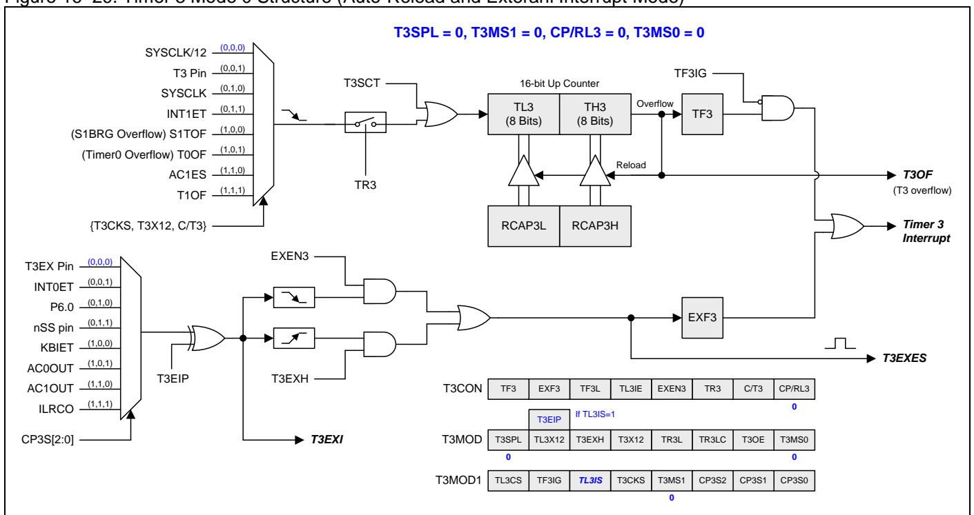
Figure 16–29. Timer 3 Mode 0 Structure (Auto-Reload and External Interrupt Mode)
