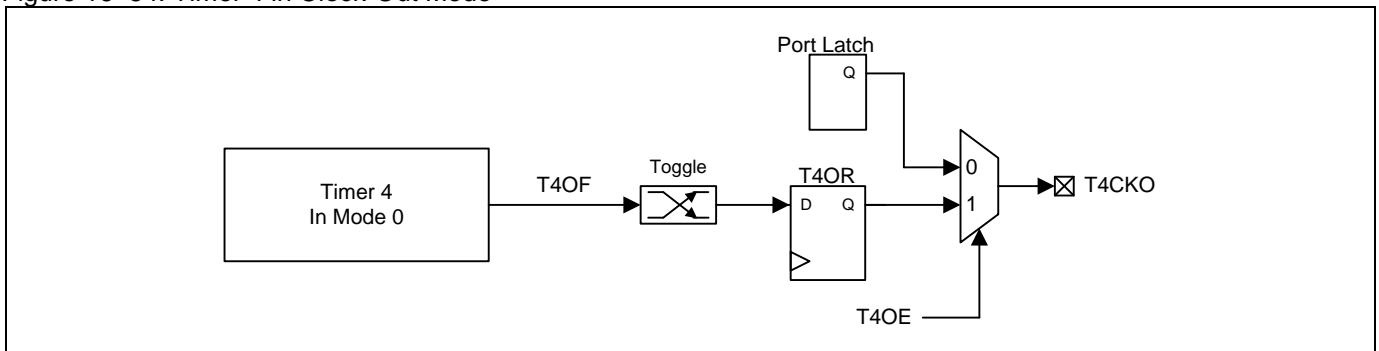
Figure 16–54. Timer 4 in Clock-Out Mode
