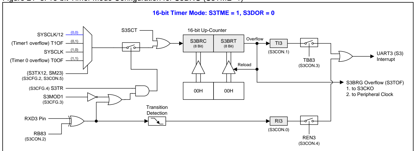
Figure 21-3. 16-bit Timer Mode Configuration for S3BRG (S3TME=1)
