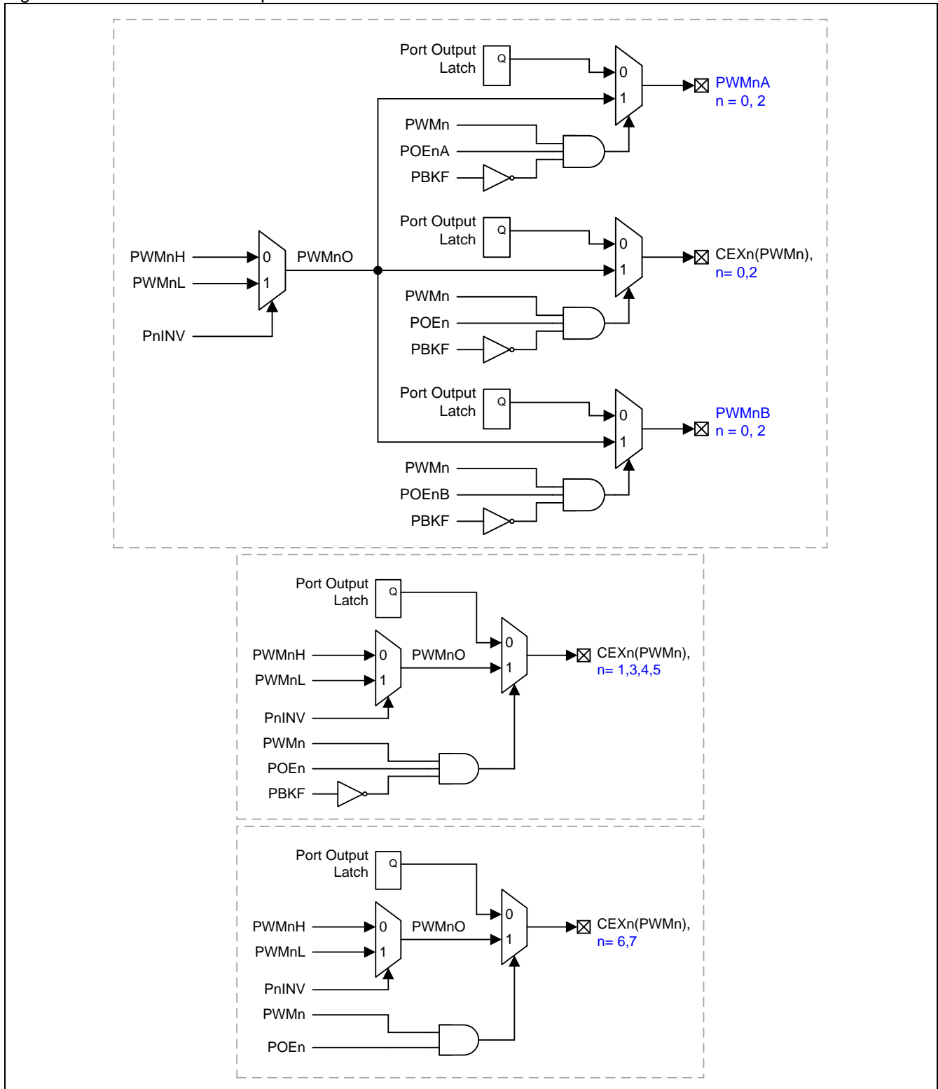
Figure 17–20. PCA Module output control
