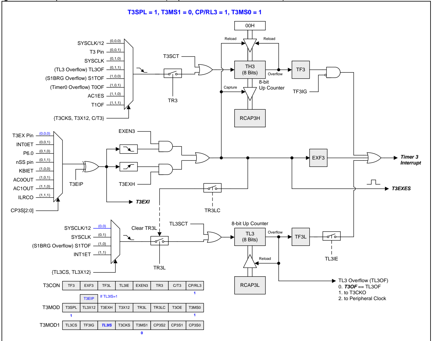
Figure 16–37. Split Timer 3 Mode 3 Structure (Capture with Auto-Zero on TH3)
