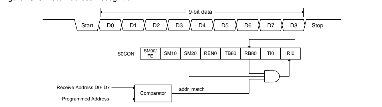
Figure 18–9. Auto-Address Recognition
