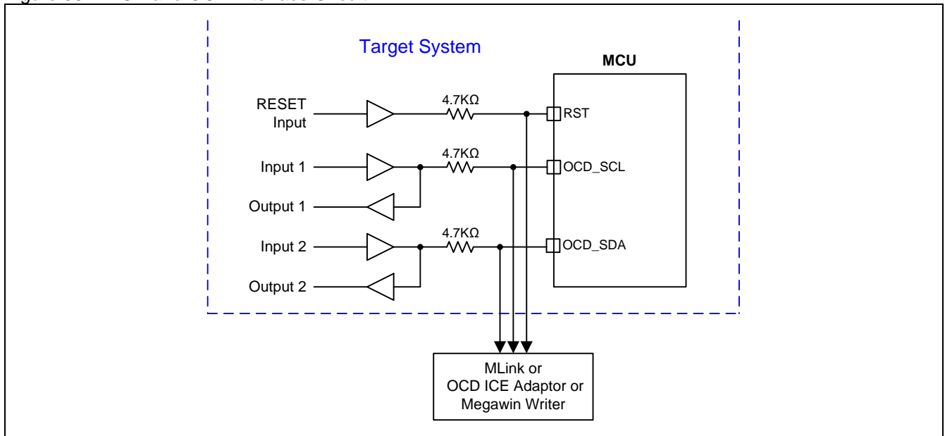
Figure 36–4. ICP and OCD Interface Circuit
