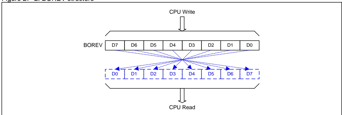
Figure 27–2. BOREV structure
