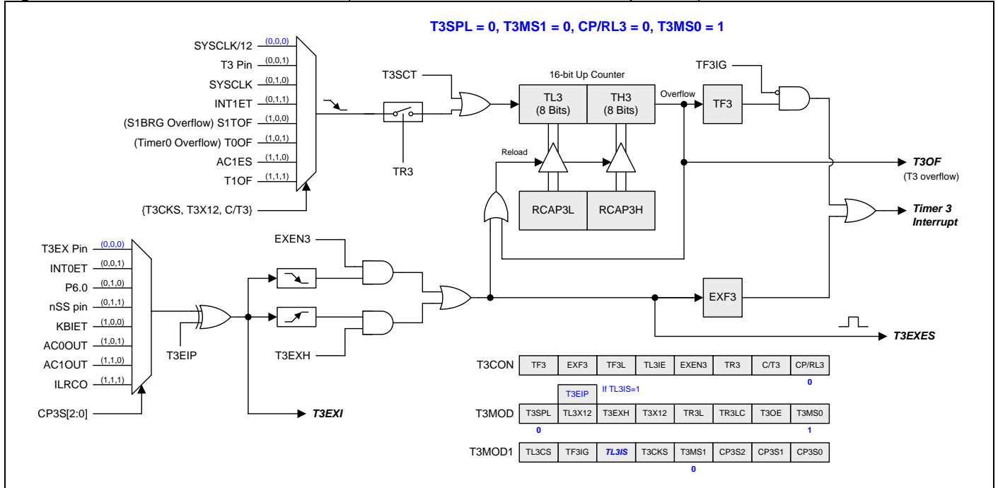
Figure 16–30. Timer 3 Mode 1 Structure (Auto-Reload with External Interrupt Mode)
