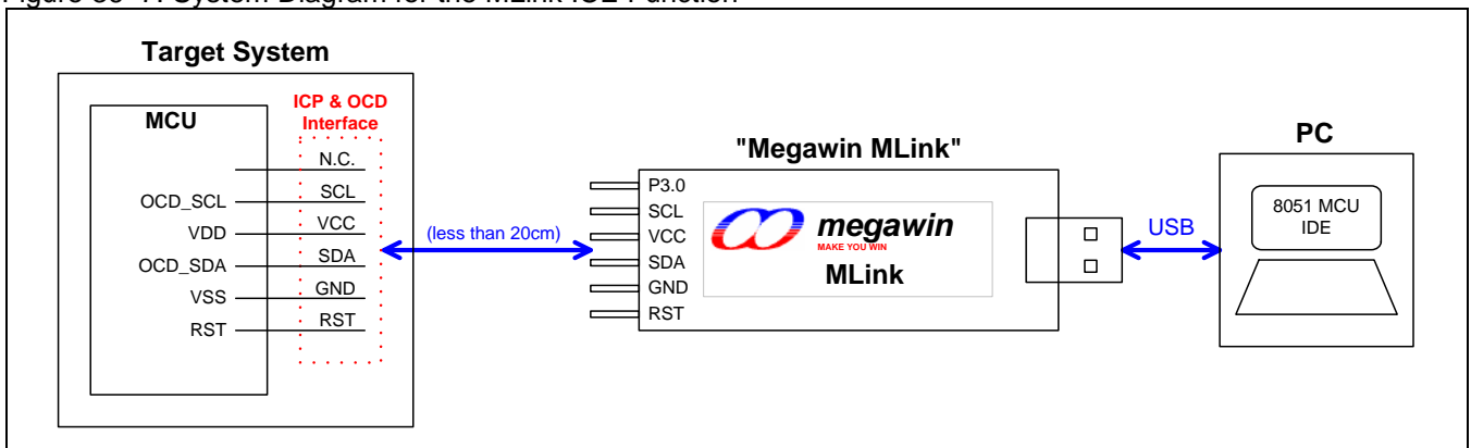
Figure 36–8. System Diagram for the ICE Function
