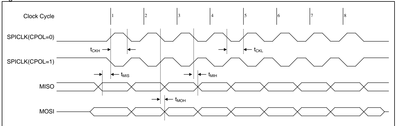
Figure 37–3. SPI Master Transfer Waveform with CPHA=0
