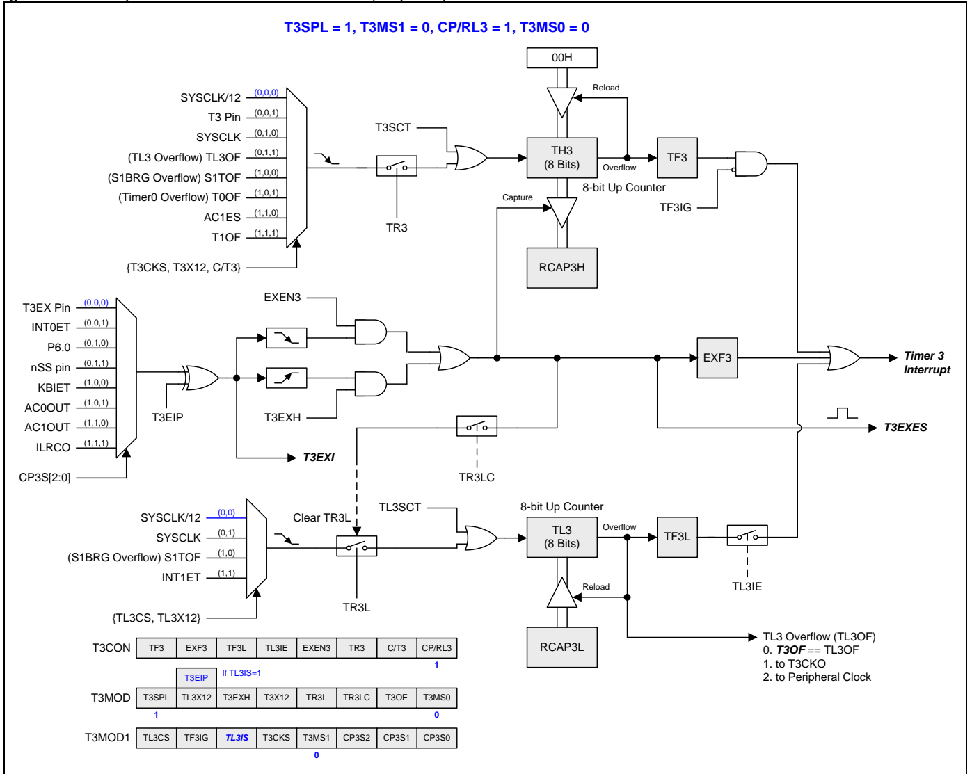
Figure 16–36. Split Timer 3 Mode 2 Structure (Capture)
