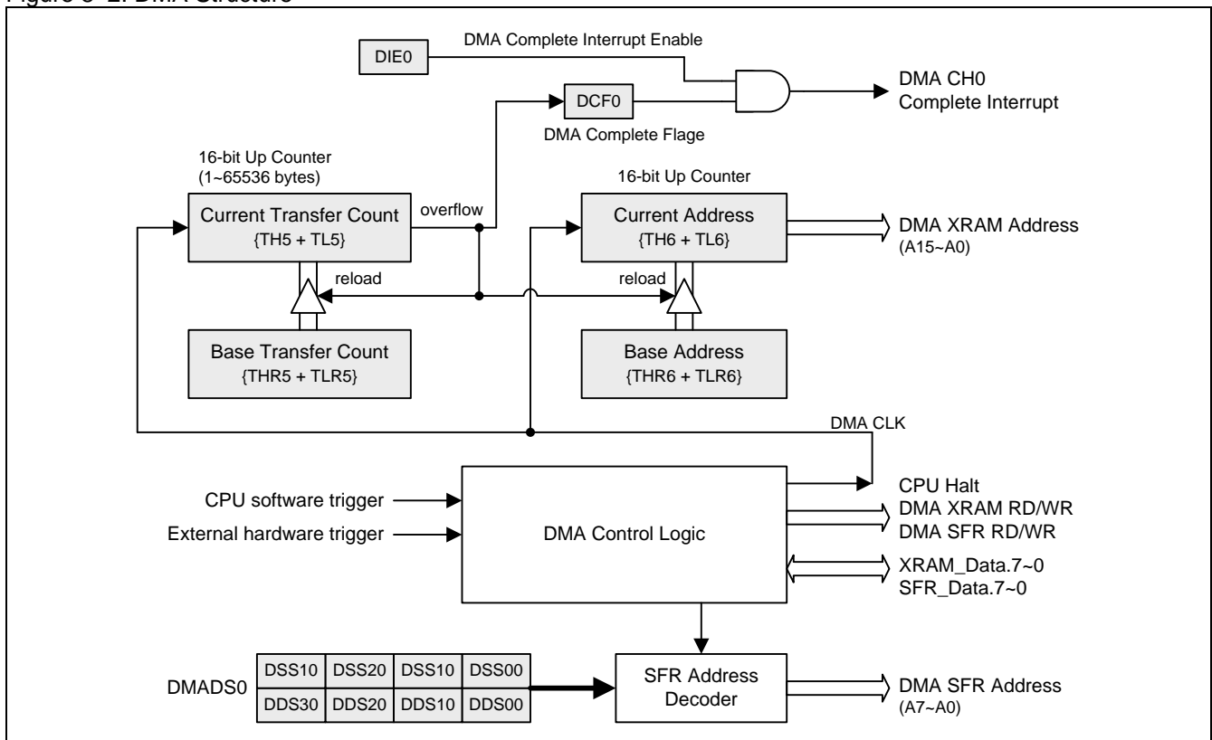
Figure 8-2. DMA Structure
