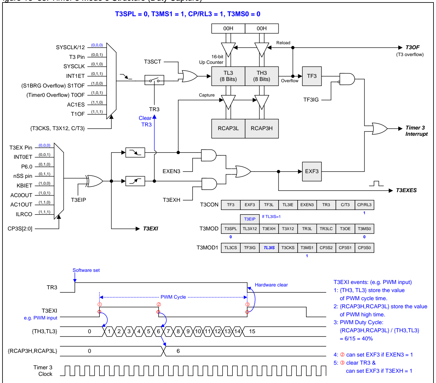
Figure 16–33. Timer 3 Mode 6 Structure (Duty Capture)
