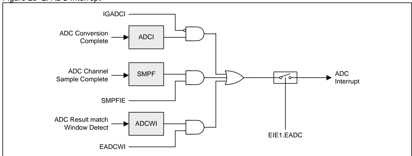
Figure 29–2. ADC Interrupt
