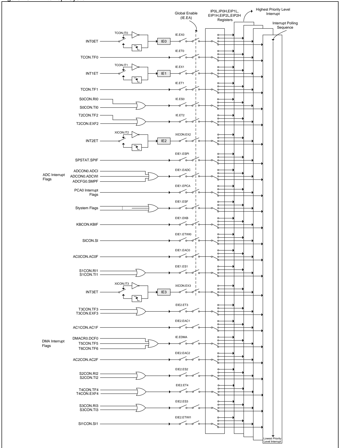
Figure 15–1. Interrupt System
