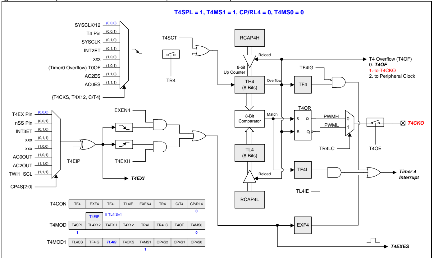
Figure 16–52. Split Timer 4 Mode 4 Structure (8-bit PWM mode)
