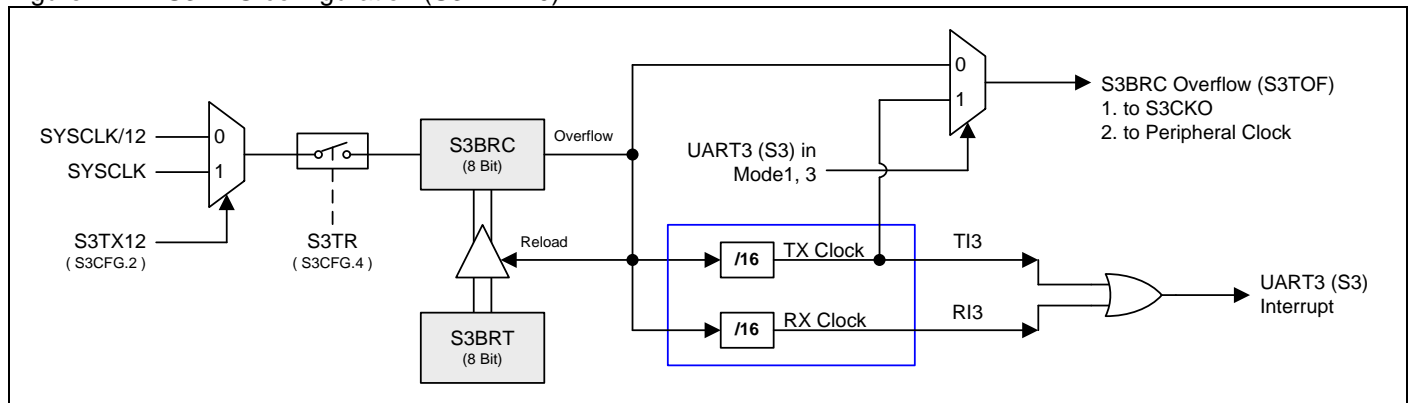
Figure 21–1. S3BRG configuration (S3TME=0)
