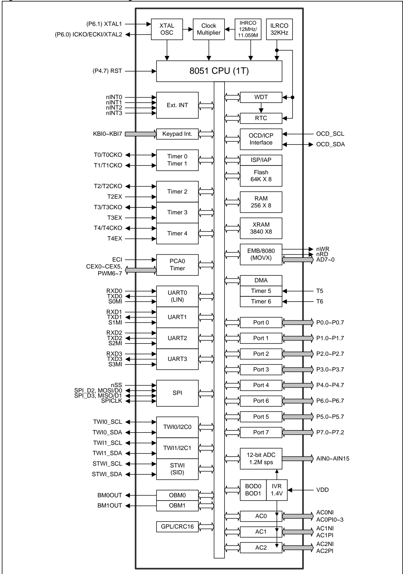
Figure 2-1. MG82G6D64 Block Diagram
