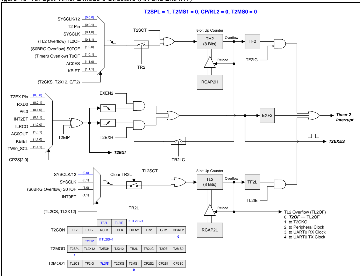
Figure 16–18. Split Timer 2 Mode 0 Structure (AR and Ext. INT)
