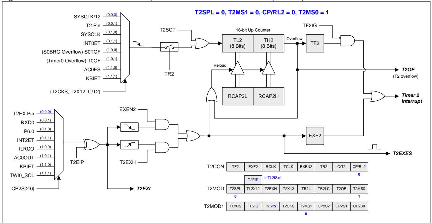
Figure 16–14. Timer 2 Mode 1 Structure (Auto-Reload with External Interrupt Mode)
