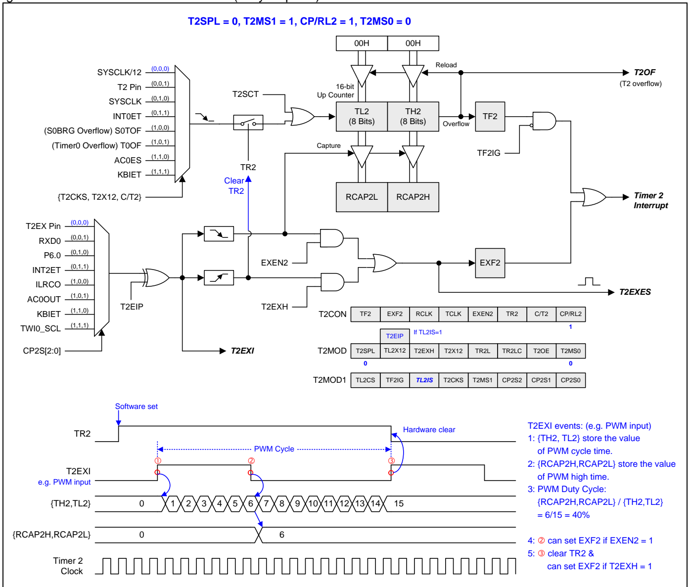
Figure 16–17. Timer 2 Mode 6 Structure (Duty Capture)
