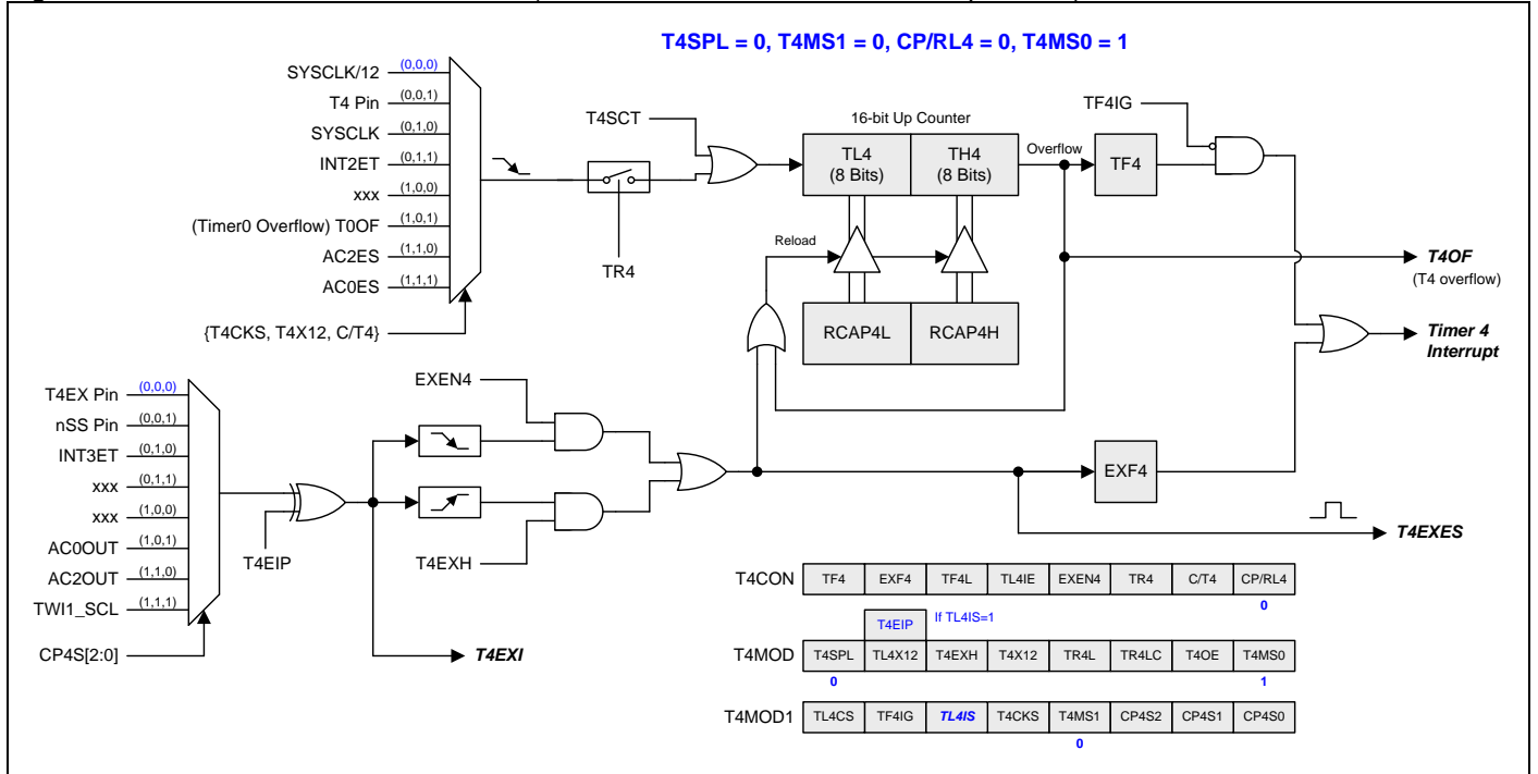
Figure 16–44. Timer 3 Mode 1 Structure (Auto-Reload with External Interrupt Mode)
