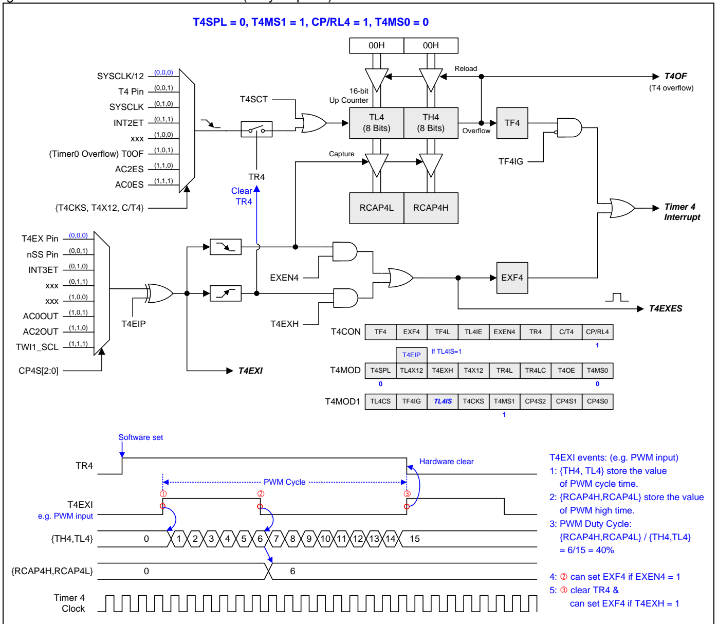
Figure 16–47. Timer 4 Mode 6 Structure (Duty Capture)
