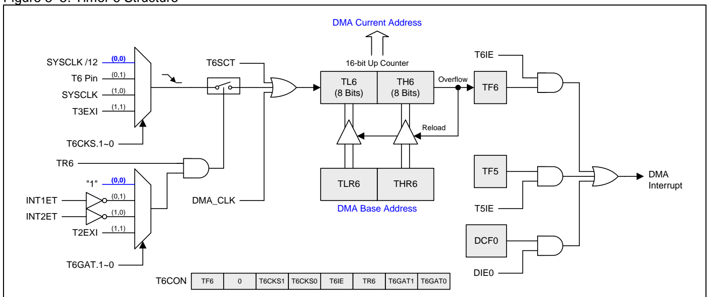
Figure 8-5. Timer 6 Structure
