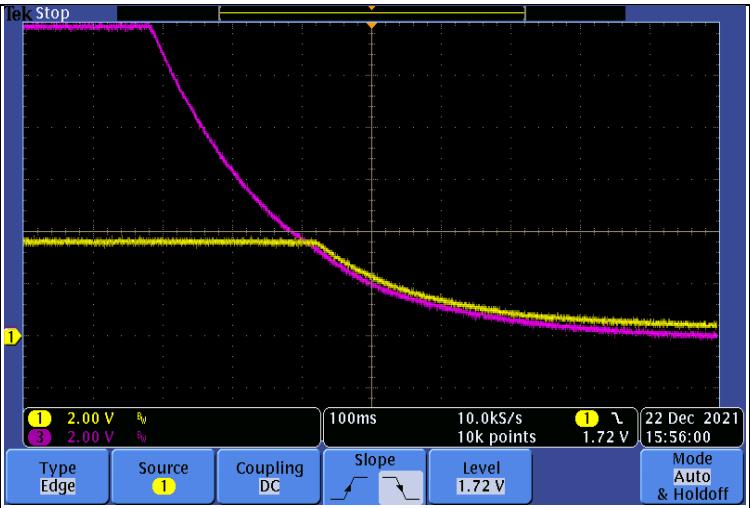
CH1: V_{IN} , CH3: V_{OUT} Fig 8. V_{IN} Shut down
