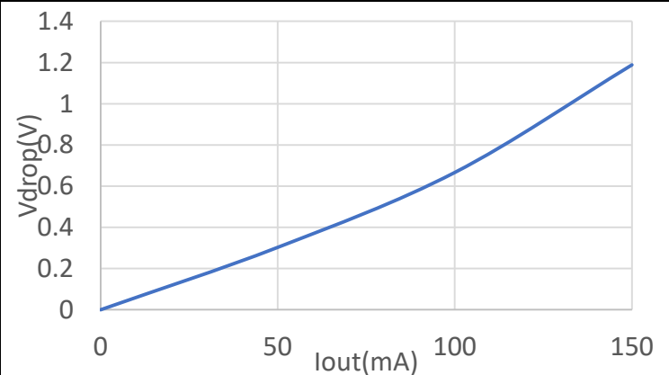
Fig 4. Dropout vs Load
