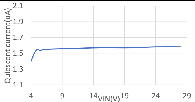
Fig 2. I_Q vs V_{IN}
