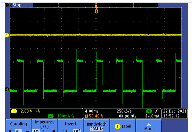
CH1: V_{OUT} , CH4: I_{OUT} Fig 6. V_{OUT} Short to GND
