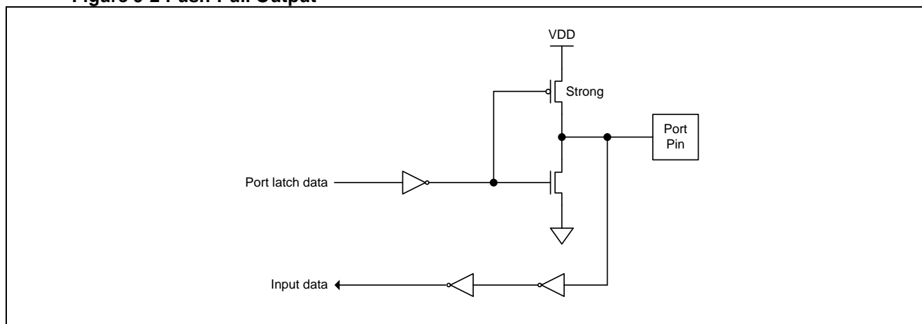
Figure 9-2 Push-Pull Output
