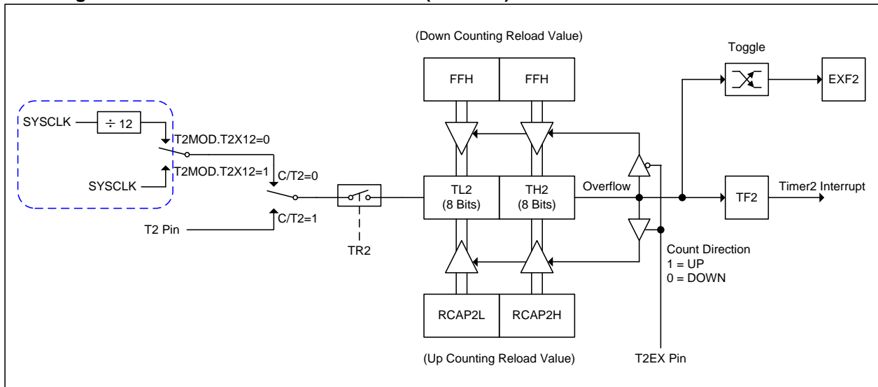
Figure 11-8 Timer 2 in Auto-Reload Mode (DCEN=1)
