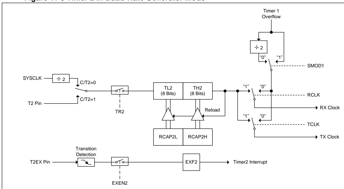
Figure 11-9 Timer 2 in Baud-Rate Generator Mode
