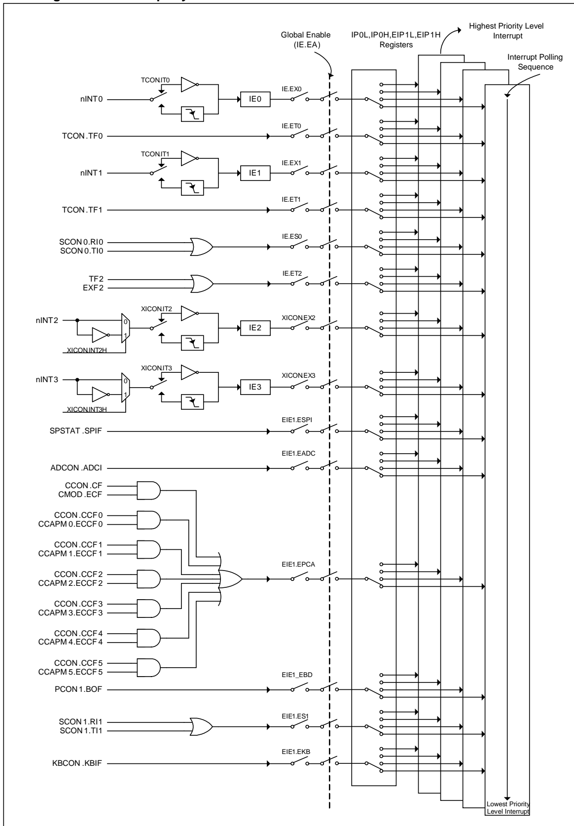
Figure 10-1 Interrupt System
