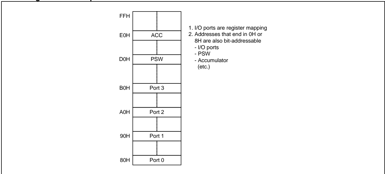
Figure 7-4 SFR Space
