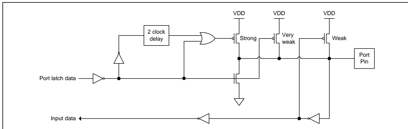
Figure 9-1 Quasi-Bidirectional I/O
