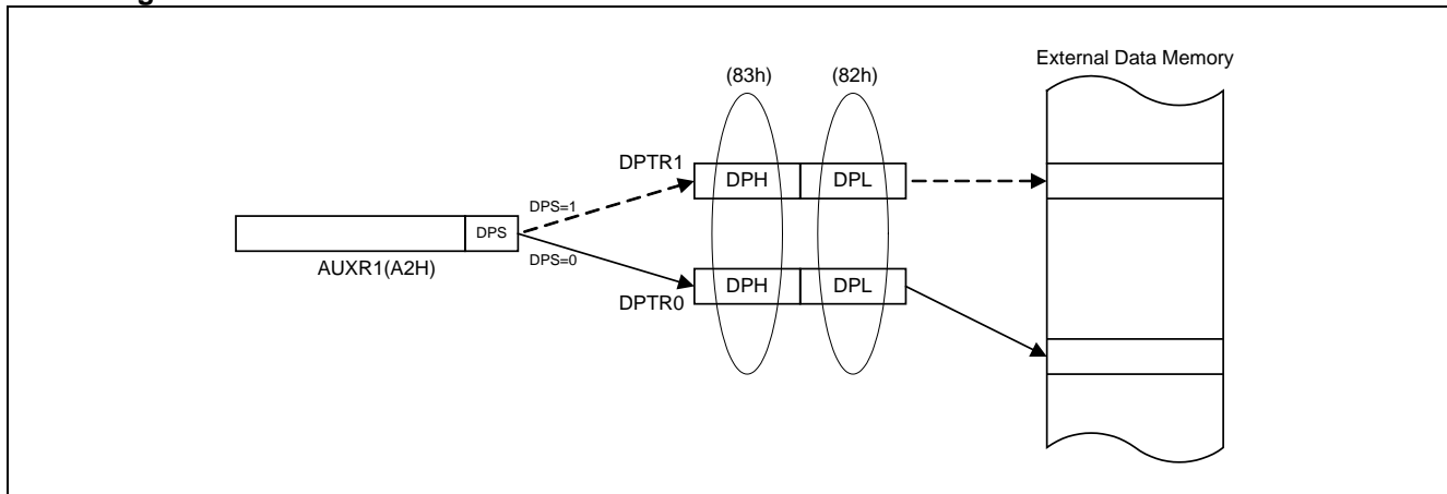
Figure 8-1 Dual DPTR
