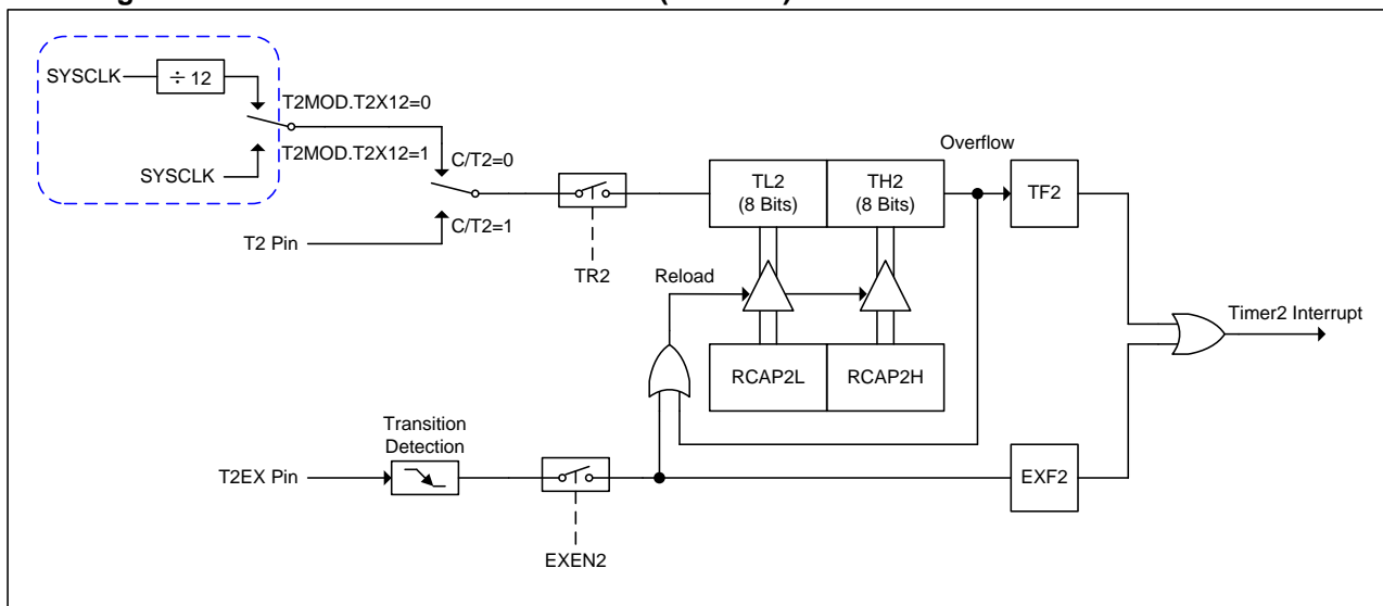
Figure 11-7 Timer 2 in Auto-Reload Mode (DCEN=0)
