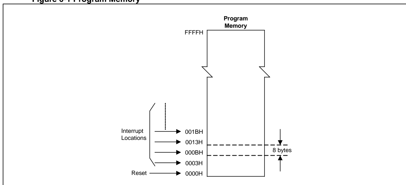
Figure 6-1 Program Memory
