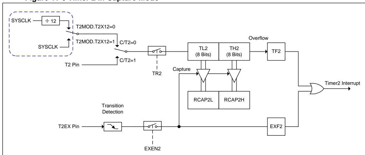
Figure 11-6 Timer 2 in Capture Mode
