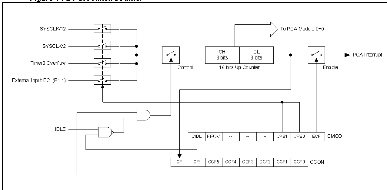
Figure 14-2 PCA Timer/Counter
