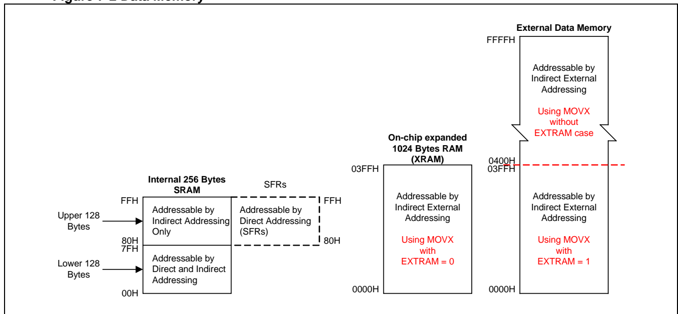
Figure 7-2 Data Memory
