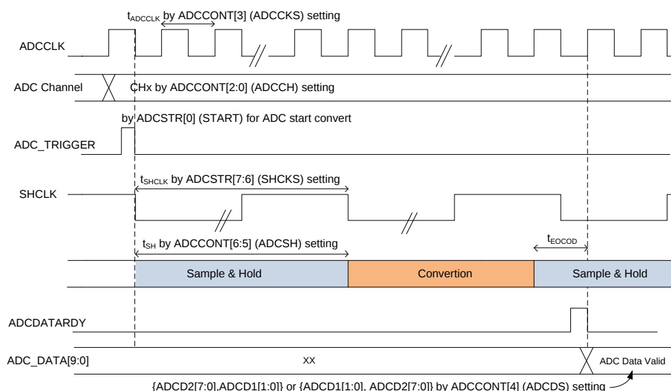
Figure 16.1.1 ADC conversion timing
