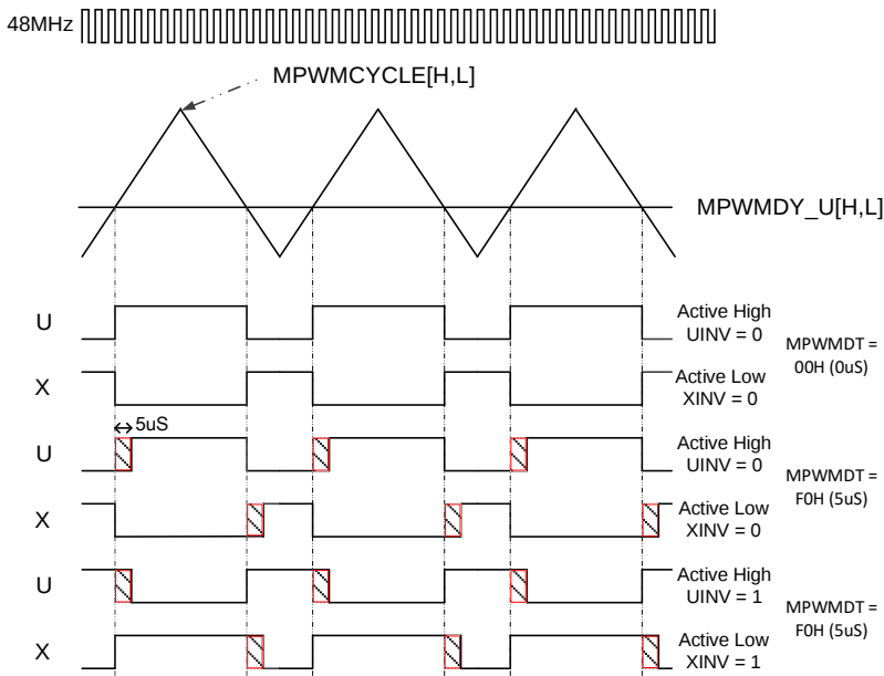
Figure25.6.8 PWM Output with Dead Time and PWM mode
