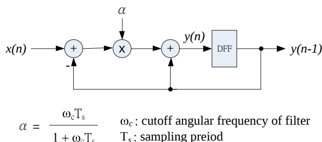
Figure 25.11.1 : first order digital low-pass filter Architecture
