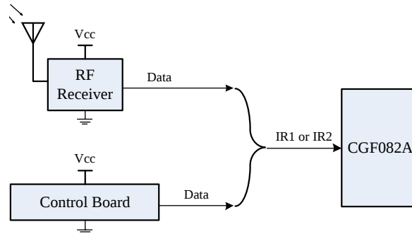
Figure 23.1 : One wire signal decode by CGF002A
