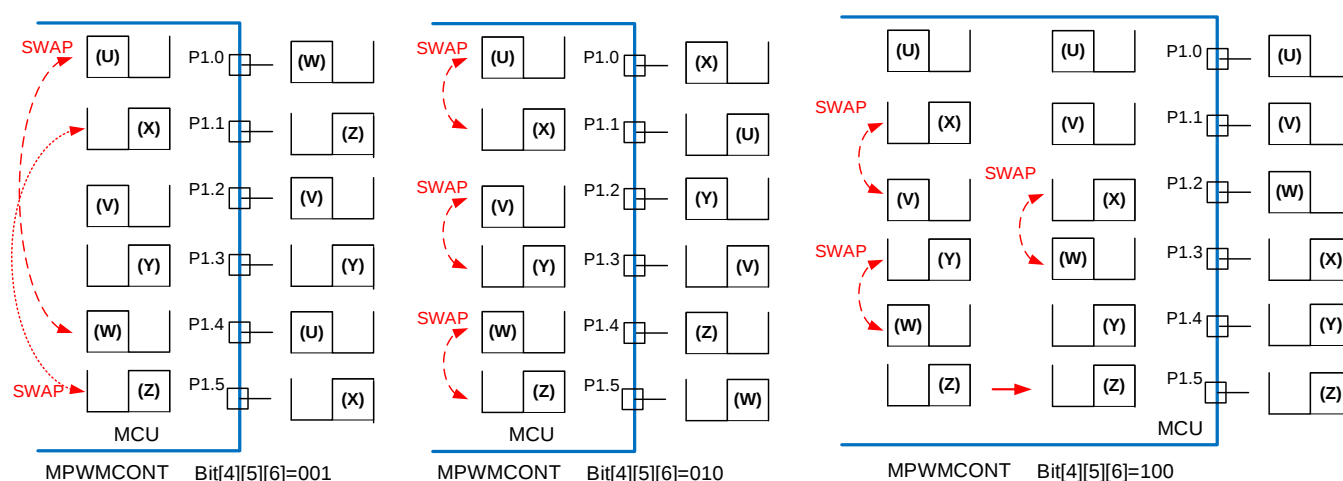
Figure25.6.7 : PWM Pin swap Unit Architecture
