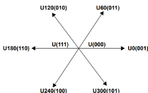
Figure 25.6.2 : Space Vector Pulse Width Modulation (SVPWM)
