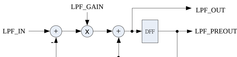
Figure 25.11.2 : LPF architecture and corresponding parameters
