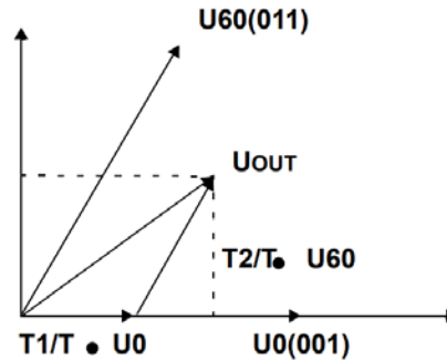
Figure 25.6.3 : AVERAGE SVPWM
