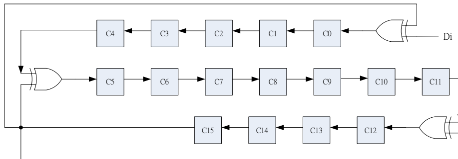
Figure 21.1 : The general LFSR architecture of CRC16-CCITT
